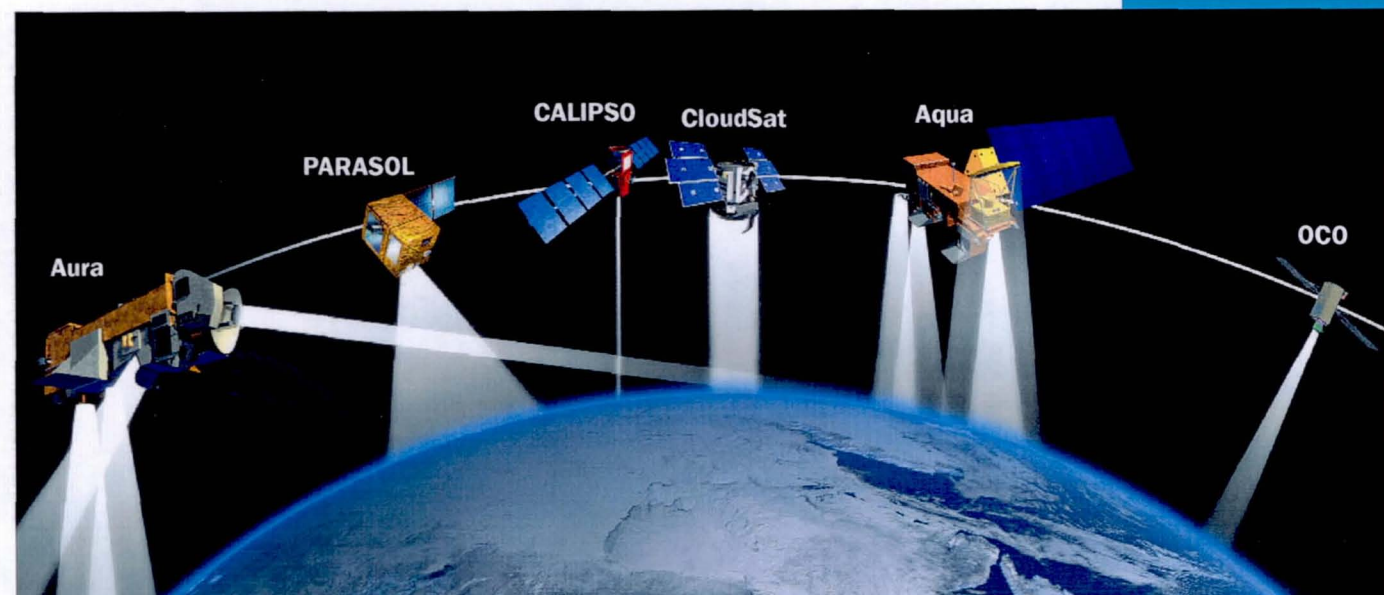
The satellites of the A-Train.
