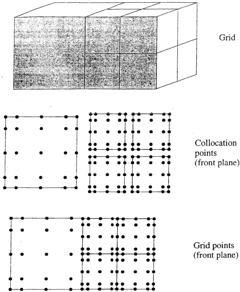
Figure 2: Collocation and grid points for simple grid
