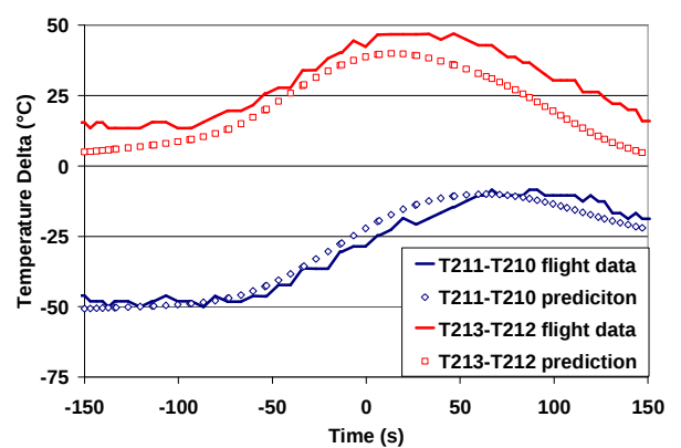
Figure 14. MGS temperature deltas, hot to cell side.
