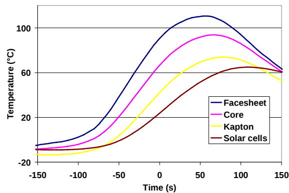
Figure 17. MGS material maximum predictions.
