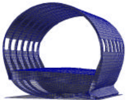
c. Front view at time = .10 seconds.
