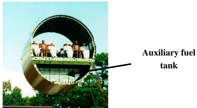
Figure 1. Pre-test photograph of the B737 fuselage section with auxiliary fuel tank.
