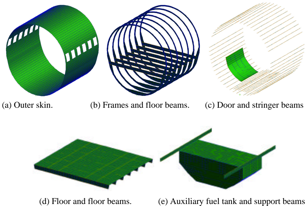
Figure 5. Components of the MSC.Dytran model of the B737 fuselage section.
