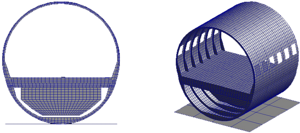
Figure 4. MSC.Dytran model of the B737 fuselage section with an auxiliary fuel tank.
