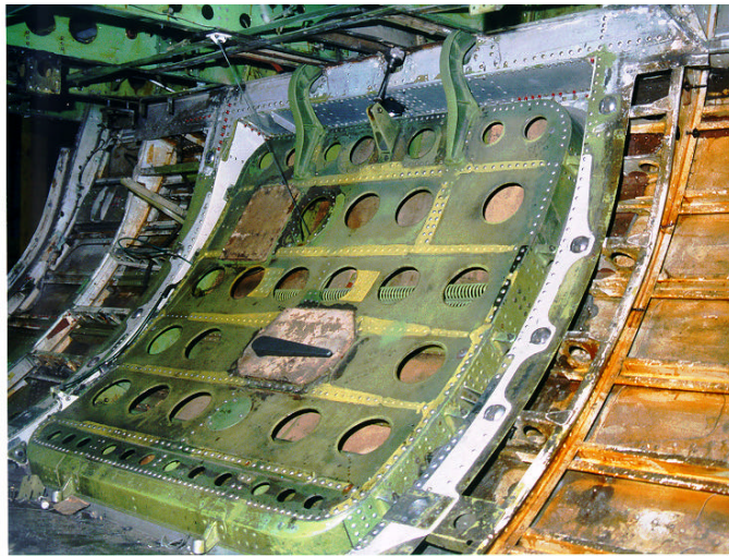
Figure 2. Photograph of the door located on the lower right side of the fuselage section.
