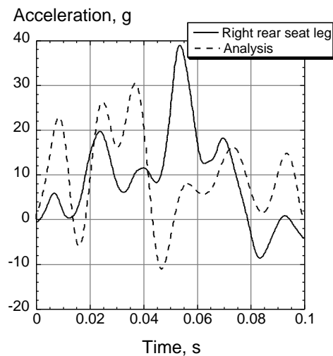
Figure 12. Comparison of measured floor acceleration at right rear seat (right rear leg) with analysis.
