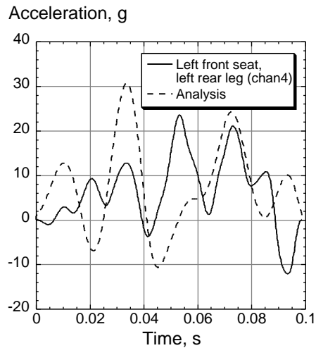
Figure 14. Comparison of measured floor acceleration at left front seat (left rear leg) with analysis.
