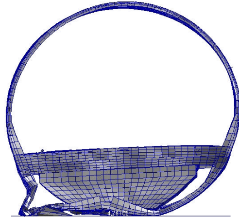
b. Analysis rear view at time 70 ms.
