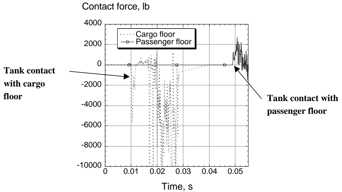
Figure 6. Contact for tank into cargo floor (10ms) and passenger floor (50ms).
