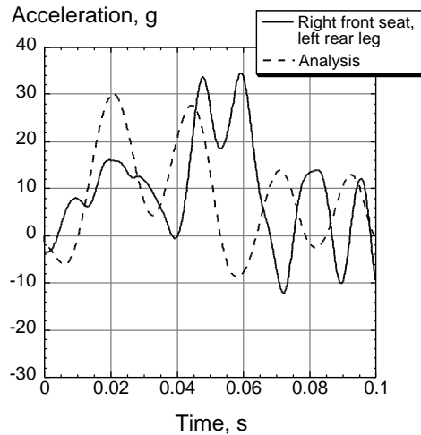
Figure 13. Comparison of measured floor acceleration at right front seat (left rear leg) with analysis.
