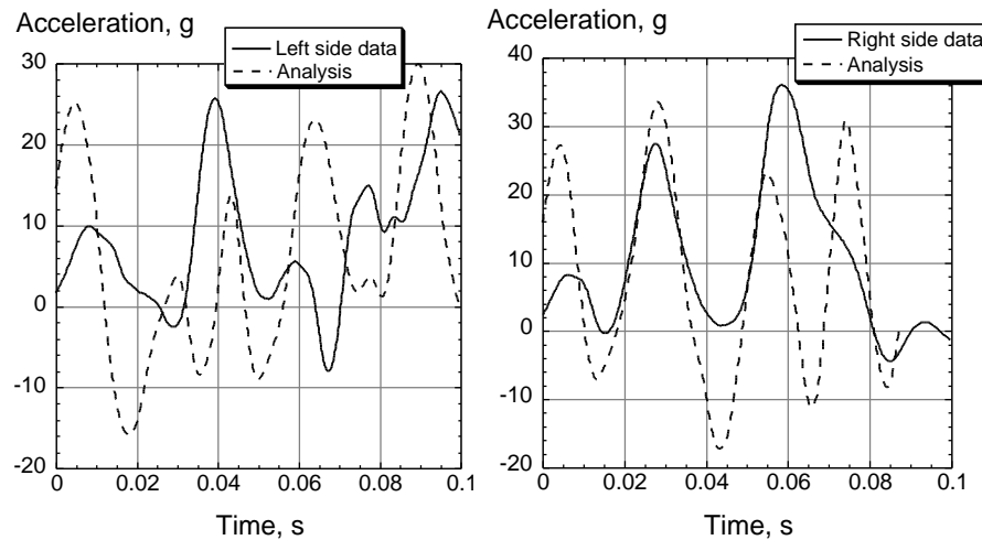
Figure 11. Left and right side floor accelerations compared with analysis.
