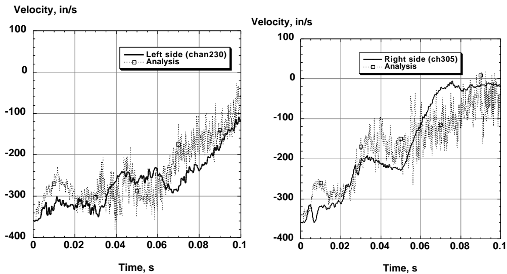
Figure 10. Left and right side measured floor velocity compared with analysis.
