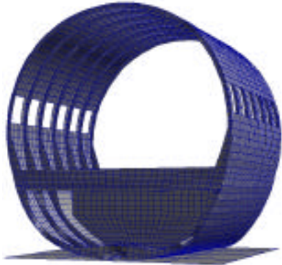
a. Front view at time = .02 seconds.
