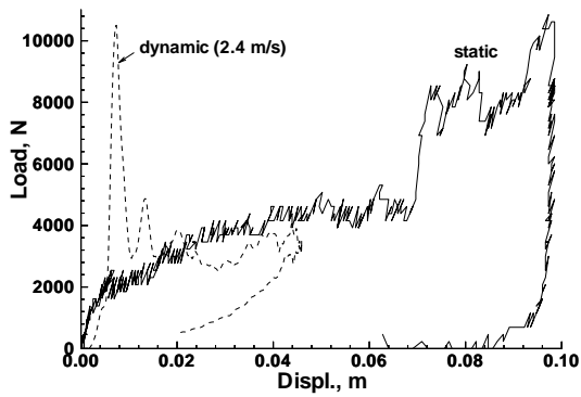
Fig. 8 Static and Dynamic crush of 0.001 m thick, 0.3 m Diameter, graphite-epoxy shells.
