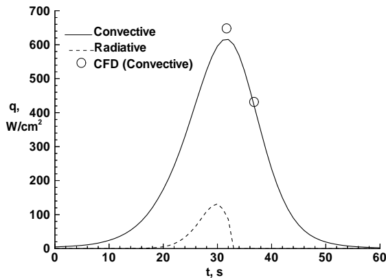
Fig. 15 Estimate of convective and radiative heating at the stagnation point
