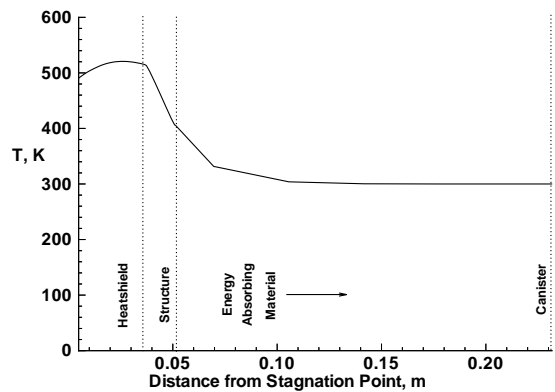
Fig. 19 Temperature distribution across heatshield, structure, and energy absorbing material at time of ground impact.
