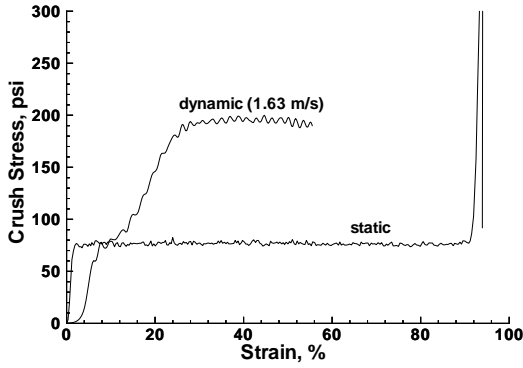
Fig. 2 Static and dynamic crushing strength of 60 kg/m 3 carbon foam
