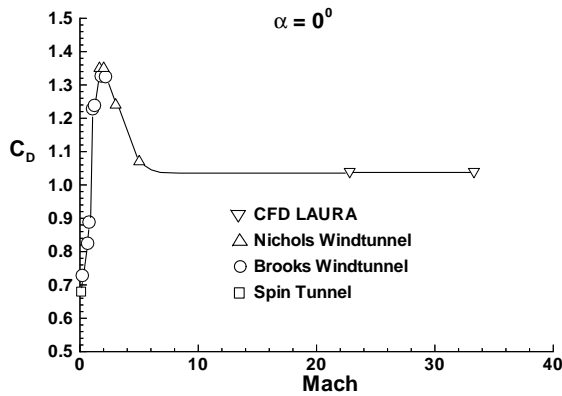
Fig. 10 Drag coefficient variation with Mach number for 45-degree half-angle design.
