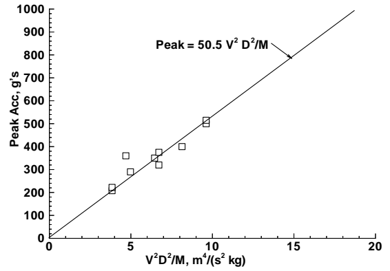
Fig 5 Variation in maximum acceleration from UTTR impact tests
