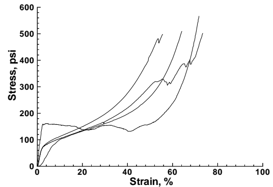
Fig. 7 Static Crush strengths of four samples of PICA-15 taken from arc-jet tested coupon.
