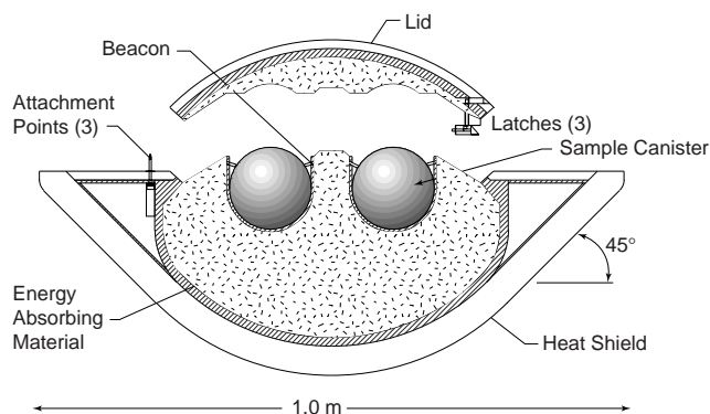
Fig 1. Schematic of entirely passive design
