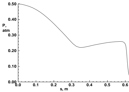
Fig. 9 Maximum forebody pressure distribution at Mach 23 for 45 degree half-angle cone design
