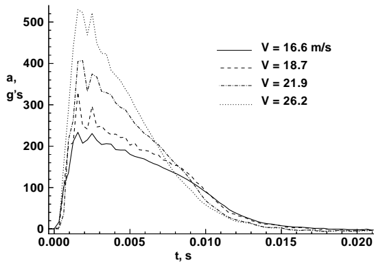
Fig. 4 Acceleration waveforms of 0.5 m, 18.5 kg penetrator impacts on UTTR surface
