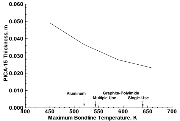
Fig. 18 Relationship between heat shield thickness and maximum temperature experienced by the underlying structure.
