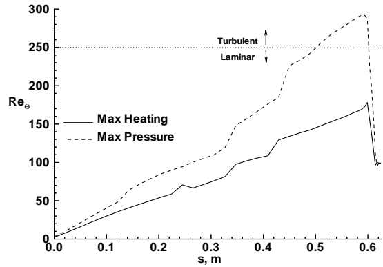
Fig. 17 Momentum thickness Reynolds numbers extracted from maximum heating and pressure CFD Solutions.
