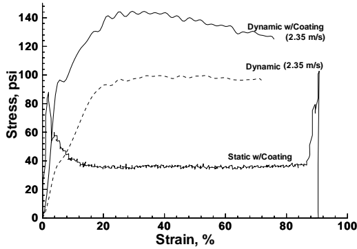
Fig. 3 Effect of surface coating on static and dynamic crushing strength of 51 kg/m 3 carbon foam
