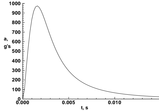
Fig. 6 Modified Meyer's law prediction of 39 m/s impact of 0.425 m radius, 43.9 kg, rigid shell with UTTR surface
