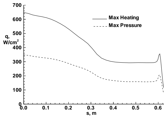
Fig. 16 Nonablating, laminar, forebody heating at maximum heating and pressure trajectory points from LAURA CFD
