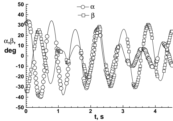
Fig. 12 Decay of large perturbation on 0.356 scale model of 45-degree half-angle design in 20-Foot Vertical Spin Tunnel
