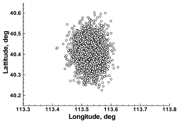
Fig. 14 Landing footprint from dispersion on entry angle, entry mass, atmosphere, and drag
