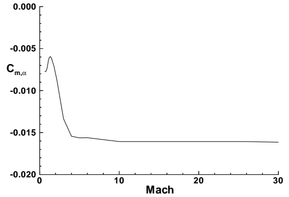
Fig 11 Moment coefficient slope variation with Mach number for 45-degree half-angle design
