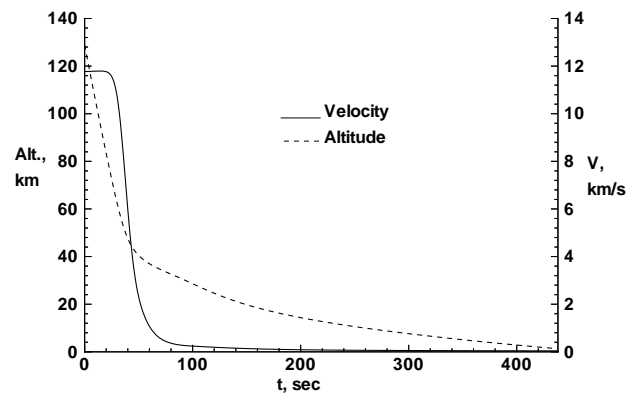
Fig. 13 Entry trajectory speed and altitude for -11.8 degree entry angle
