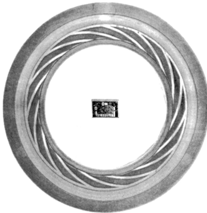
Figure 42.—Seal nosepiece with chemically etched inward-pumping spiral grooves. (Strom et al., 1967.)
