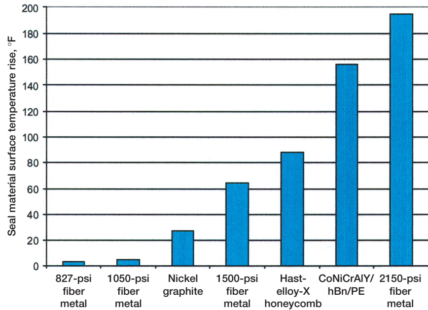
Figure 28.—Surface temperature rise with low-speed abrasability test. (Chappel et al., 2001b.) Courtesy Technetics Corp.
