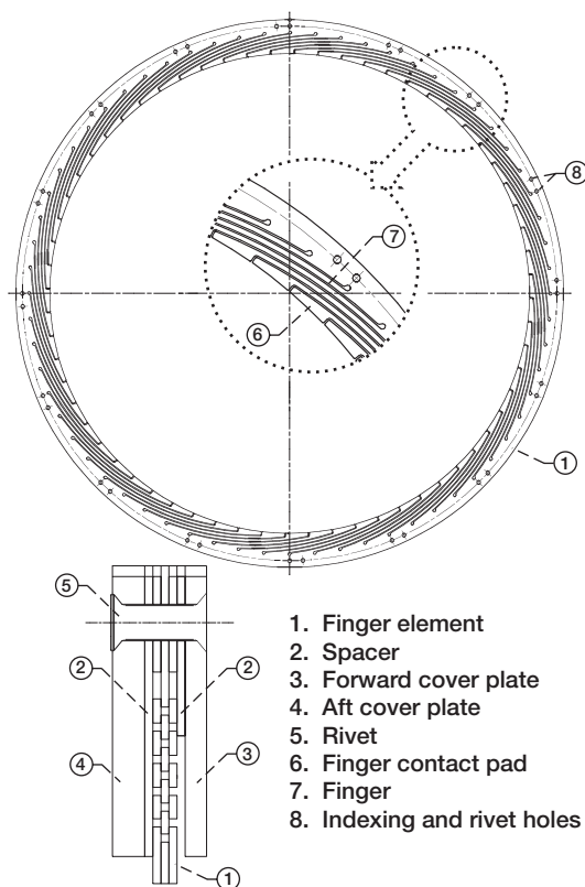
Figure 36.—Finger seal design. (Proctor et al., 2002.)
