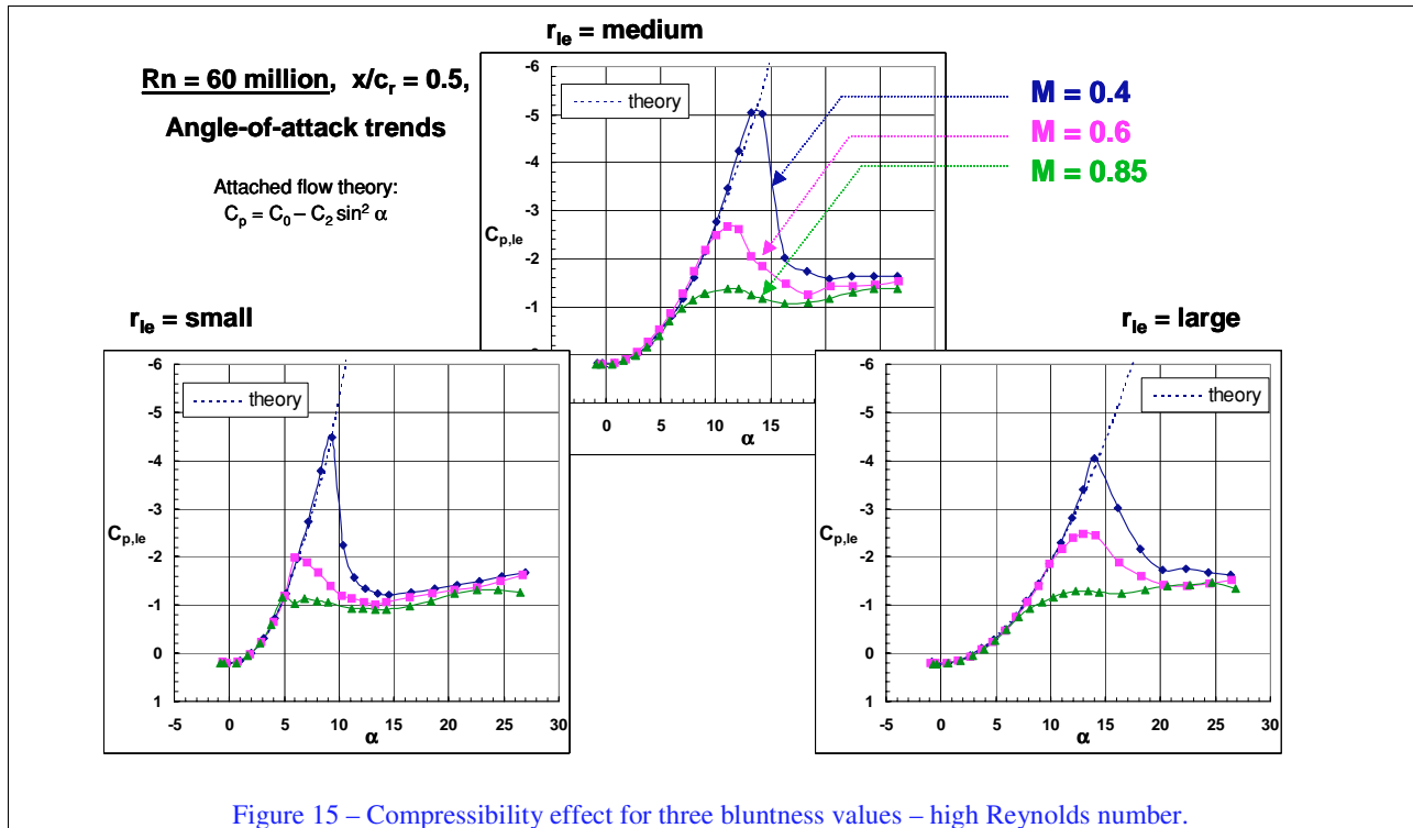
Figure 15 – Compressibility effect for three bluntness values – high Reynolds number.
