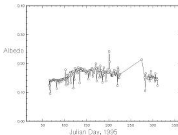
Figure 3 -- Instantaneous surface albedo over forest site for a solar zenith angle of 49 degrees.
