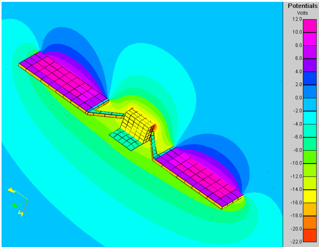
Figure 4a. Potentials calculated for spacecraft in solar wind environment.
