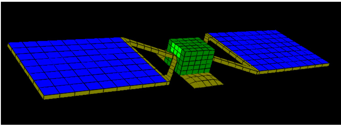
Figure 2d. Object Toolkit model of spacecraft.
