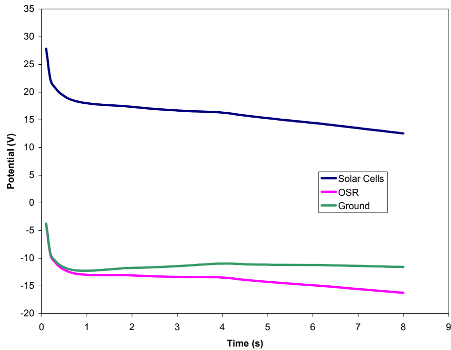
Figure 4b. Time history of potentials for solar wind calculation.
