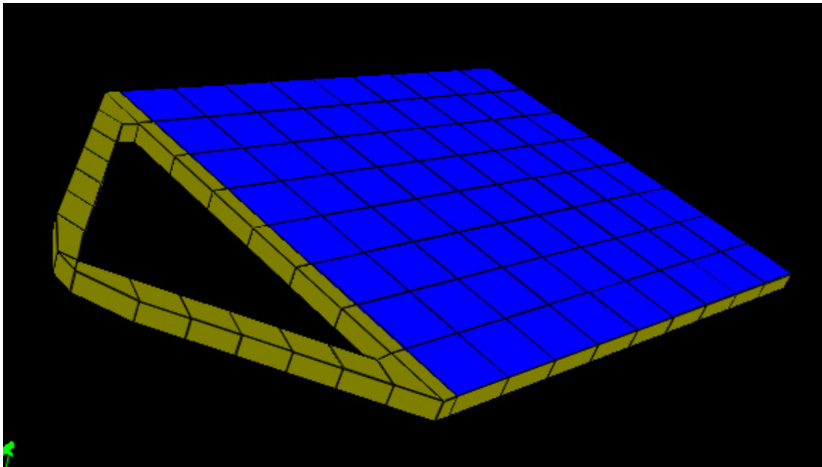
Figure 2b. Object Toolkit model of solar array wing.
