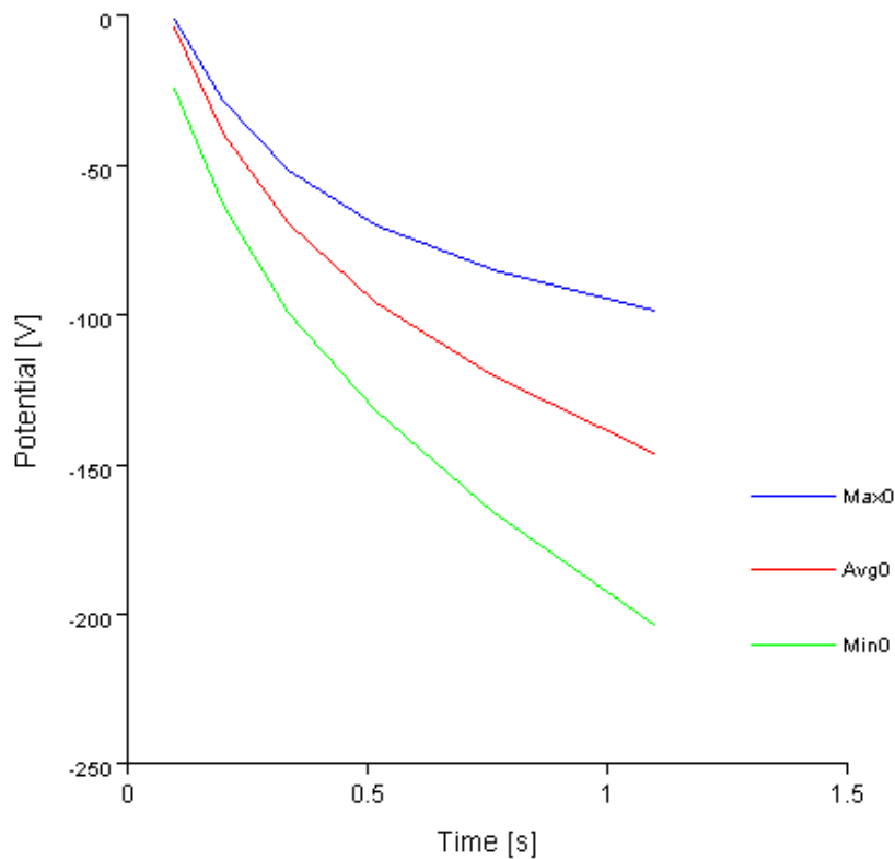
Figure 5b. Time dependence of overall and differential charging for the sample auroral charging calculation.
