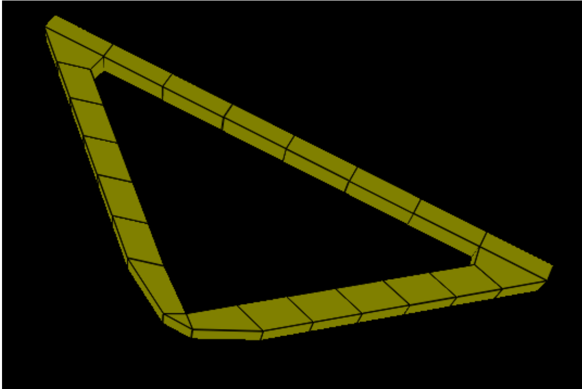
Figure 2a. Object Toolkit model of truss for mounting solar array.
