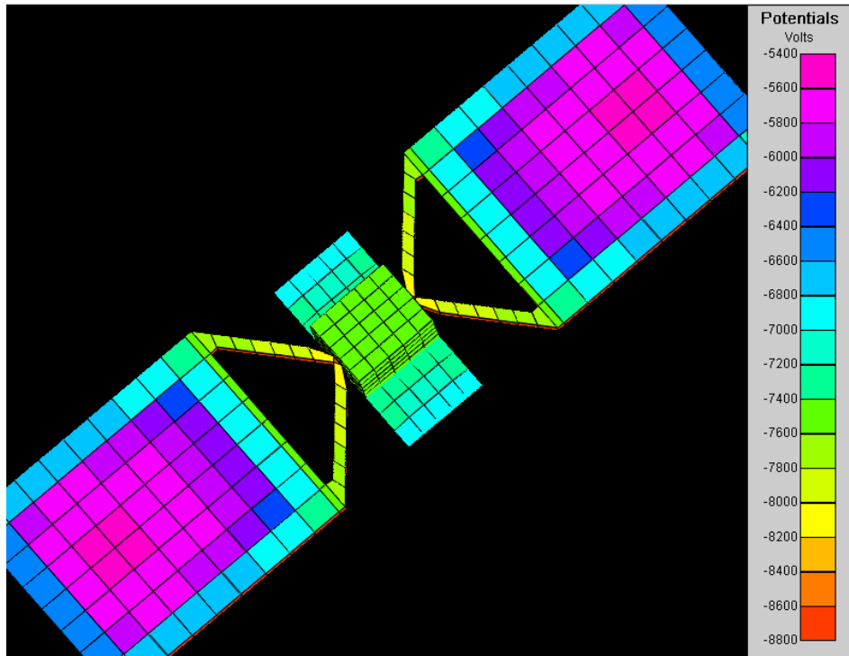
Figure 3a. Geosynchronous charging result, showing maximum differential charging toward outboard end of solar panels.
