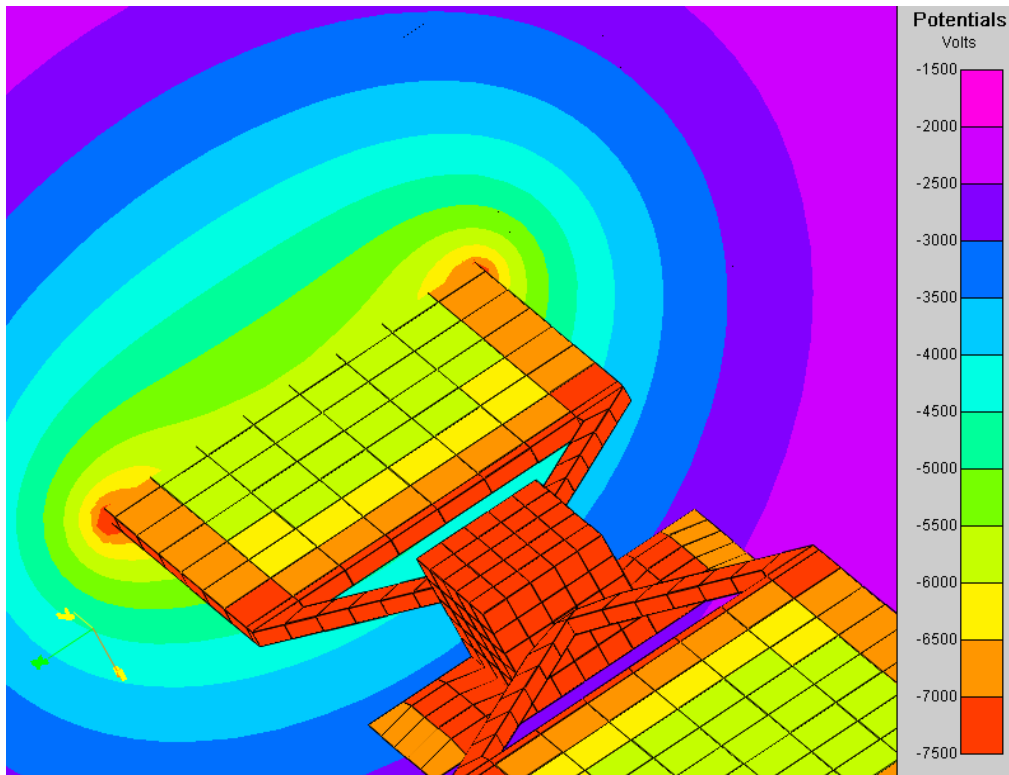
Figure 3b. Geosynchronous charging result, showing saddle point over solar panel.
