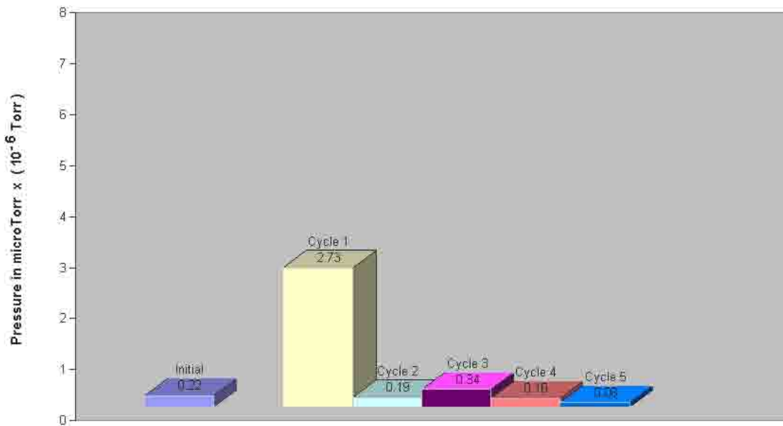
Figure 4.b: Partial Pressure of water in the Teney vacuum chamber after each heating cycle. Recorded pressures were obtained after the arrays cooled back down to 11 deg. Celsius.
