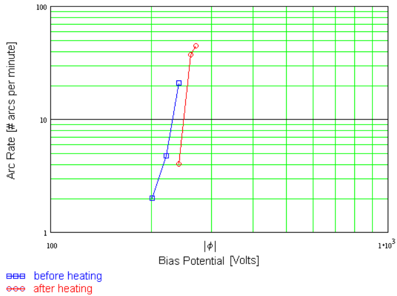
Figure (5.a): Arc inception voltage before and after 3 heating cycles
