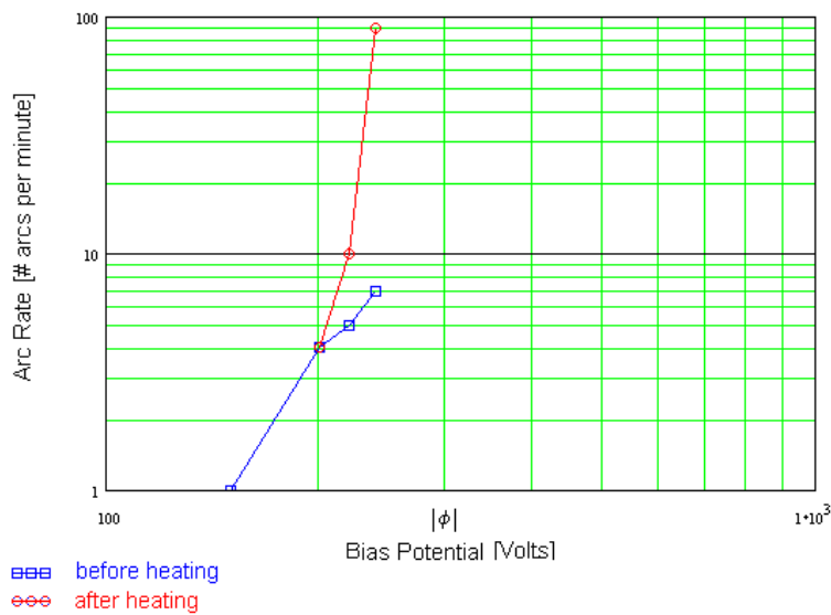
Figure (5.d): Arc inception voltage before and after 5 heating cycles
