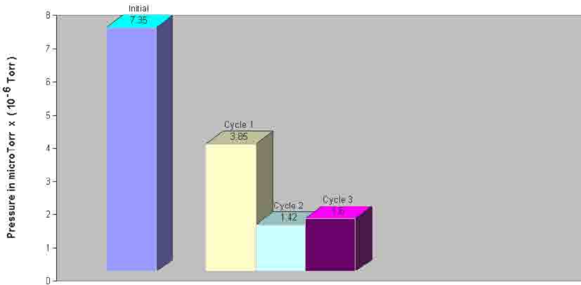
Figure 4.a: Partial pressure of water in the vertical chamber after each heating cycle. The recorded pressures were obtained after the arrays were cooled back down to the 11 deg. Celsius.
