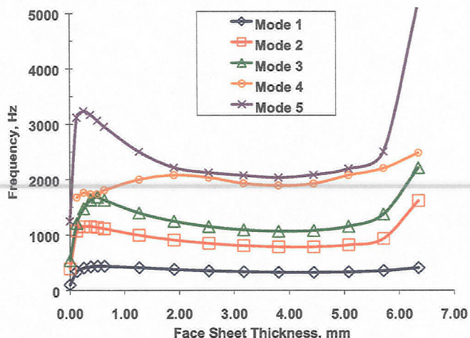
Figure 8: Variation of the natural frequency as a function of the face sheet thicknesses for the 160.0 x 82.6 x 12.7 mm having an overall constant plate thickness.
