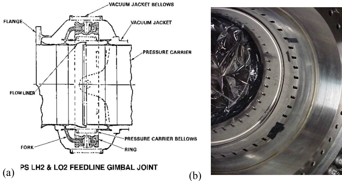
Figure 1. (a) The liquid hydrogen line joint and the location of the flow liner. (b) The inside of the joint and the slotted flow liner configuration.
