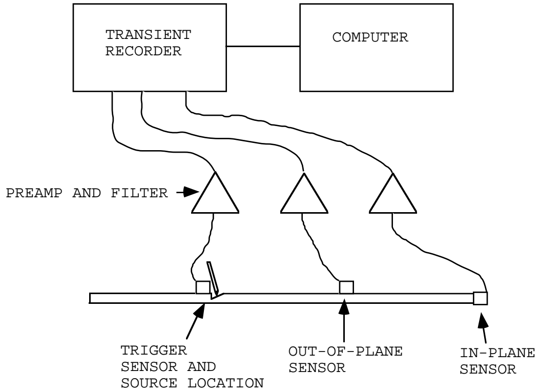
Fig. 3 Experimental setup.
