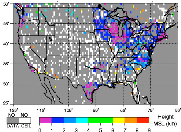
Fig. 3. Cloud base heights from ASOS ceilometers, 1900 UTC, 18 March 2004.
