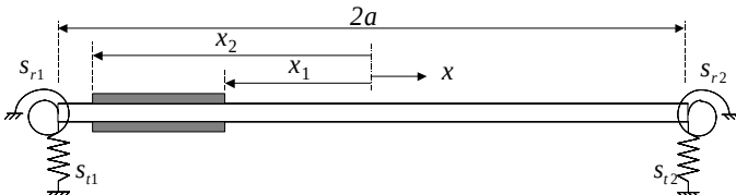
Figure 3. Flexural vibration of the beam under generally supported boundary condition.
