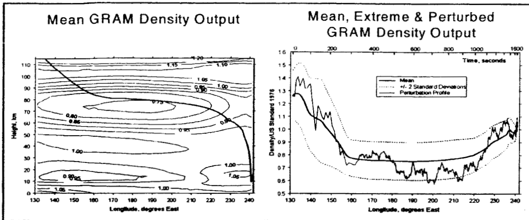
Figure 5. Resultant GRAM-99 Mean and Extreme Density Values Computed Along the Example January Re-entry Trajectory into Edwards AFB. Density is expressed as a ratio to the US76 Standard Atmospheric Density. Left figure is plot of mean January Density (vs. Height and Longitude). Right figure is Density Ratio vs. Longitude for Mean January, \pm 2 -Sigma, and Monte-Carlo density realization.
