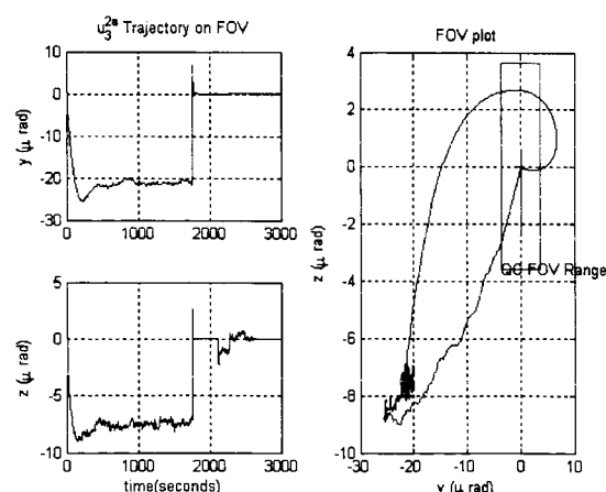
Figure 13 Time History of Telescope Pointing Error: Link 6
