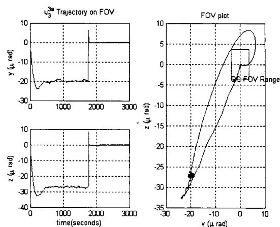
Figure 12 Time History of Telescope Pointing Error: Link 5
