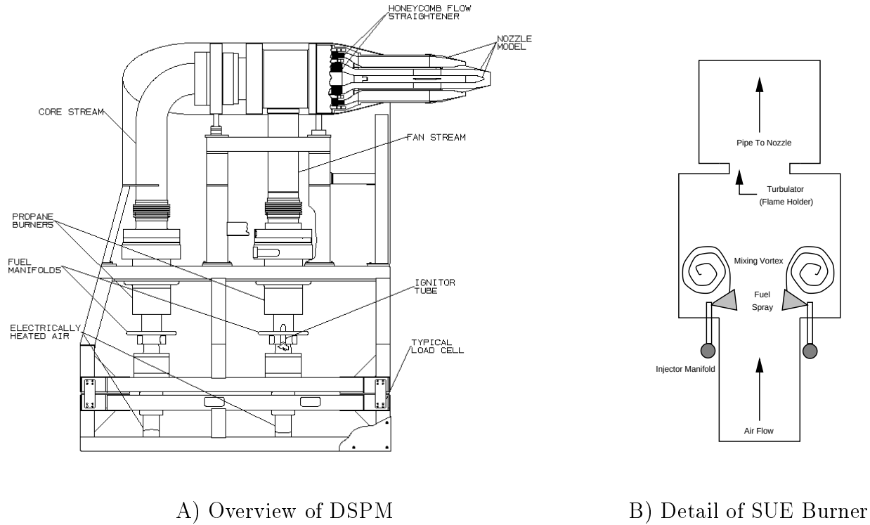
Figure 2: Dual Stream Propulsion Model
