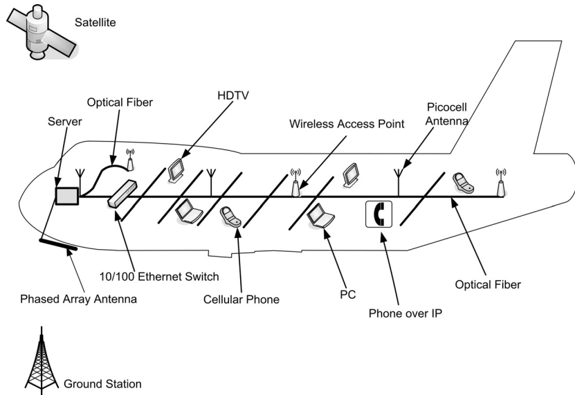
Figure 1.—Prospective services onboard of a commercial aircraft in the near future.
