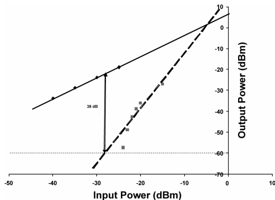
Figure 15.—Dynamic Range for Ch31.
