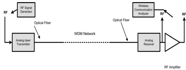
Figure 3.—The Experimental Setup for Measuring Signal-to-Noise Ratio (SNR).
