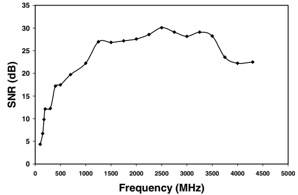
Figure 6.—Results of SNR Measurements for Ch1310.
