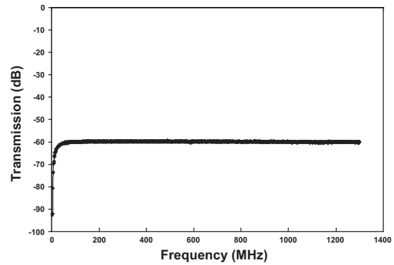
Figure 12.—Results of Transmission Response Measurements for Ch1550.
