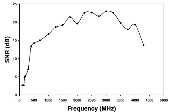
Figure 7.—Results of SNR Measurements for Ch1550.
