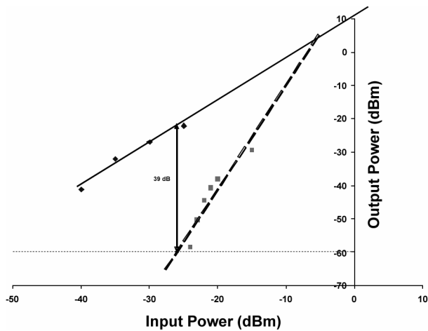
Figure 14.—Dynamic range for Ch29.
