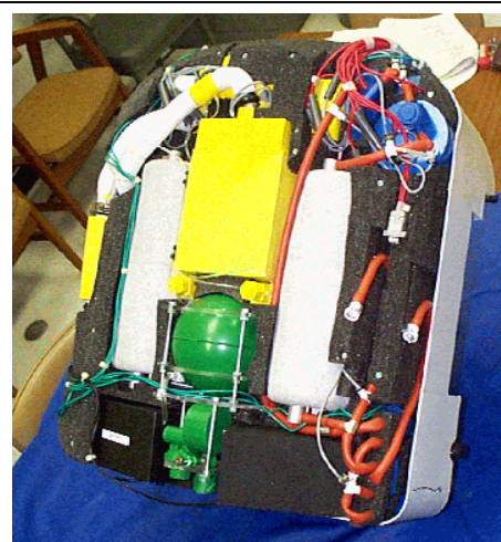
Figure C.1-15. “Foam” advanced PLSS concept.
