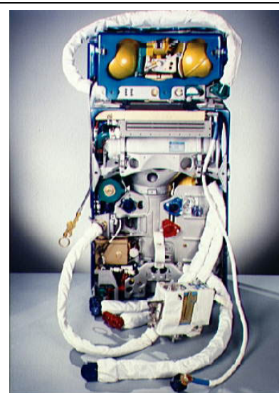
Figure B.1-7. The Apollo PLSS showing the OPS (in blue on top), the PLSS (in the center), and the Remote Control Unit (in the lower foreground). (MSC photo S70-39666).
