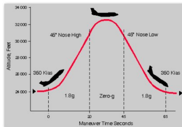
Figure B.5-5. A typical parabolic flight profile used to simulate a reduced-gravity environment.
