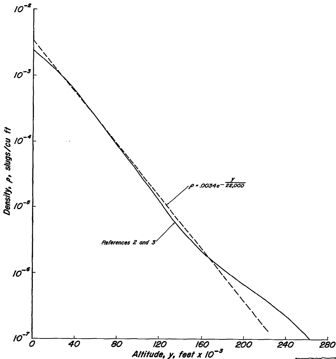
Figure 1.— Variation of density with altitude.
