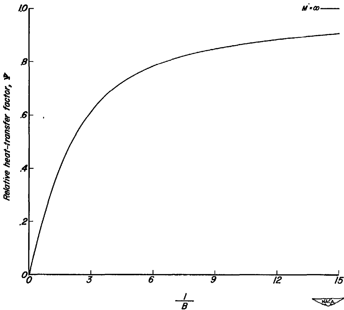
Figure 9.- Variation of relative heat-transfer factor \Psi with 1/B .
