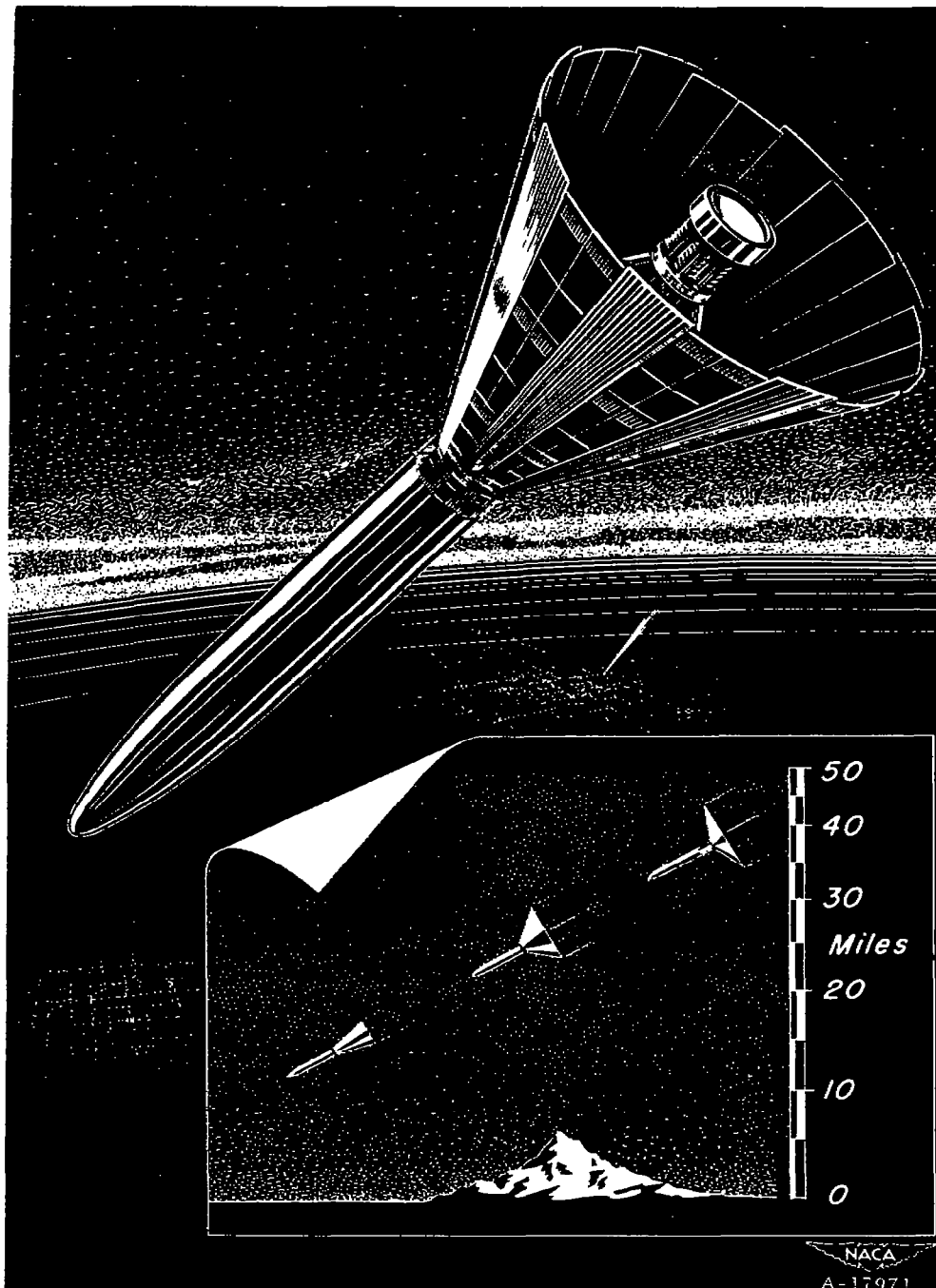
Figure 12.- Flared-skirt missile penetrating the earth's atmosphere.
