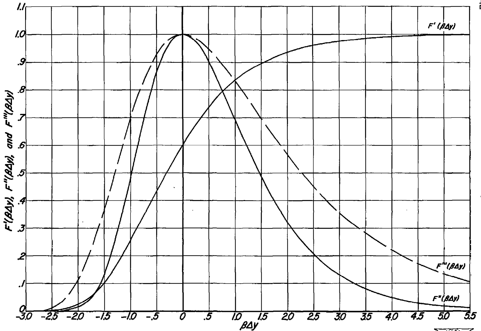
Figure 4.- Variations of F'(\beta\Delta y) , F''(\beta\Delta y) , and F'''(\beta\Delta y) with \beta\Delta y .
