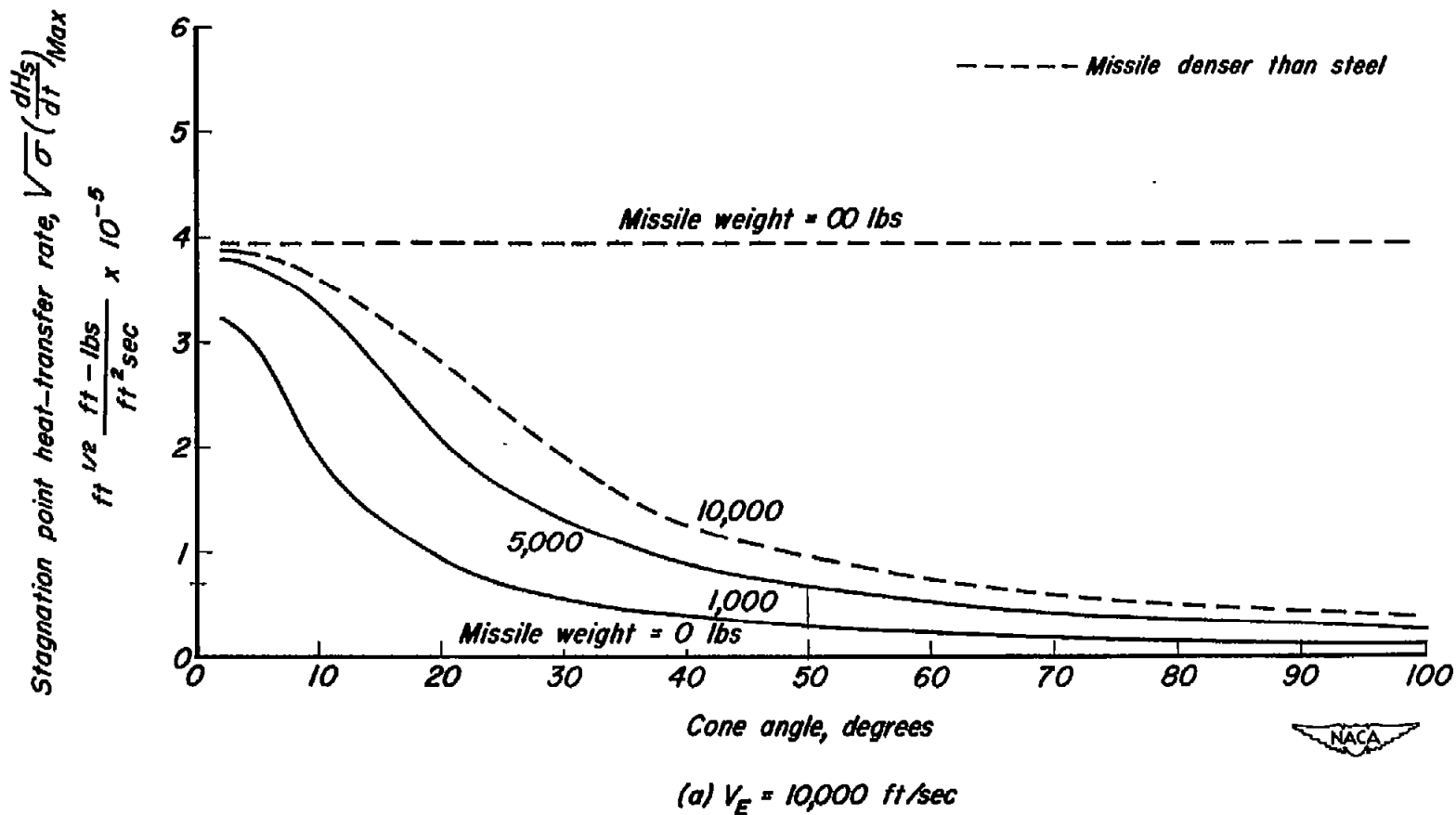
Figure 11.— Maximum rate of convective heat transfer to the stagnation point of spherically tipped cones of the same volume entering the earth's atmosphere at an angle of 30^\circ to the horizontal and velocities of 10,000, 20,000, and 30,000 ft/sec (volume = 16.34 cu ft).
