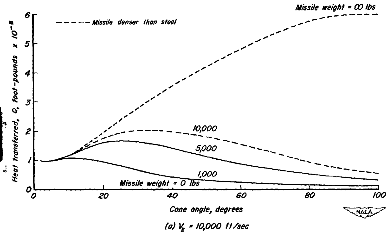
Figure 6.— Convective heat transferred at impact to conical missiles of same volume entering the earth's atmosphere at an angle of 30^\circ to the horizontal and velocities of 10,000, 20,000, and 30,000 ft/sec (volume = 16.34 cu ft).
