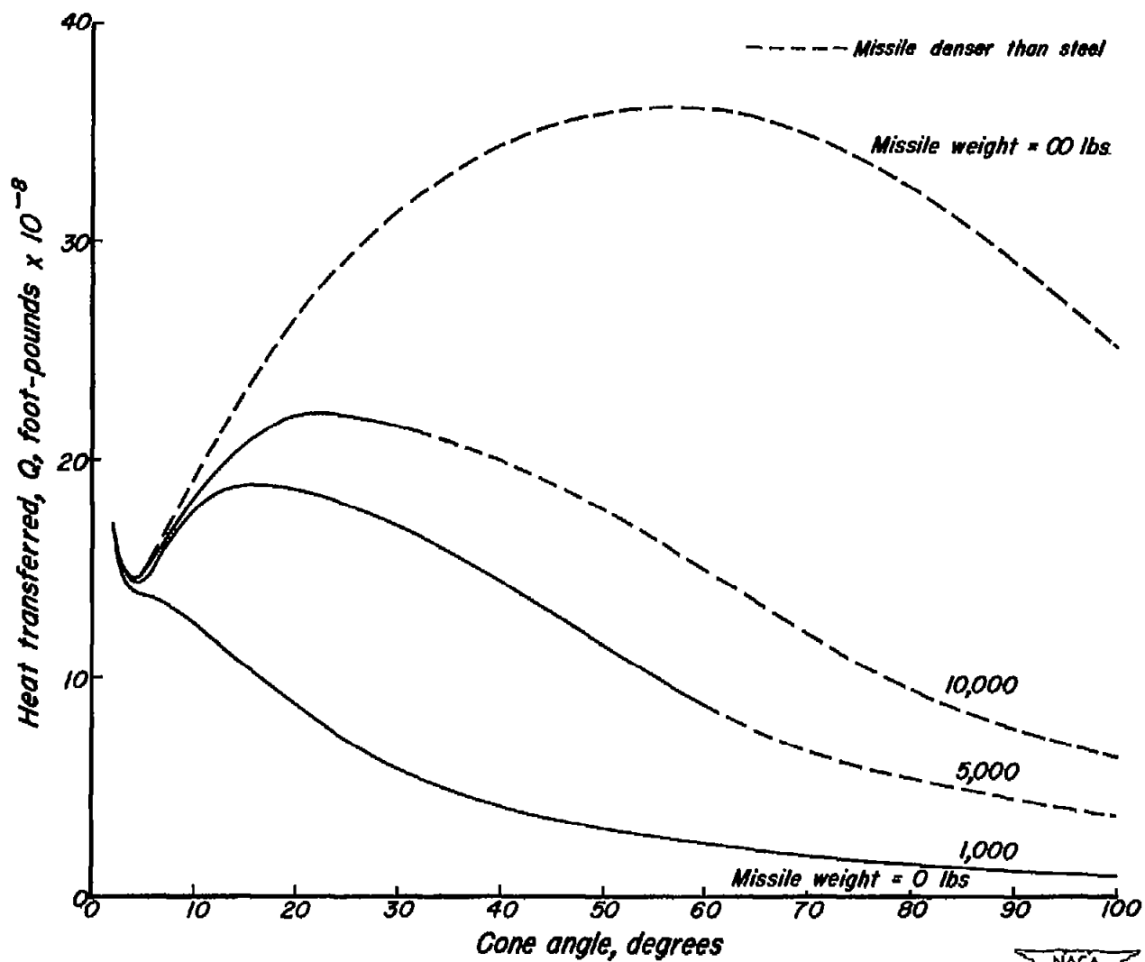
(c) V_E = 30,000 ft/sec Figure 5.- Concluded.
