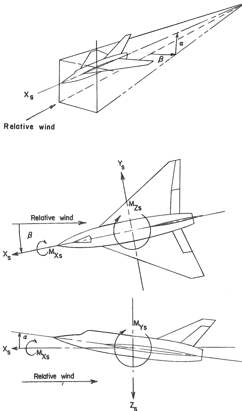
(b) Stability axes.
