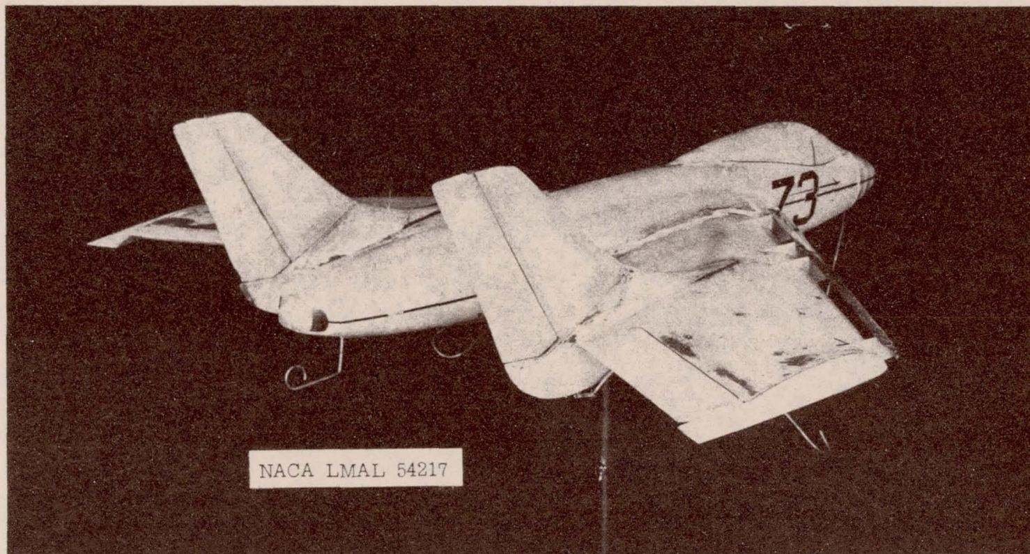
Figure 6.- Three-quarter rear view of \frac{1}{10} -scale model of Chance Vought XF7U-1 with slats extended.
