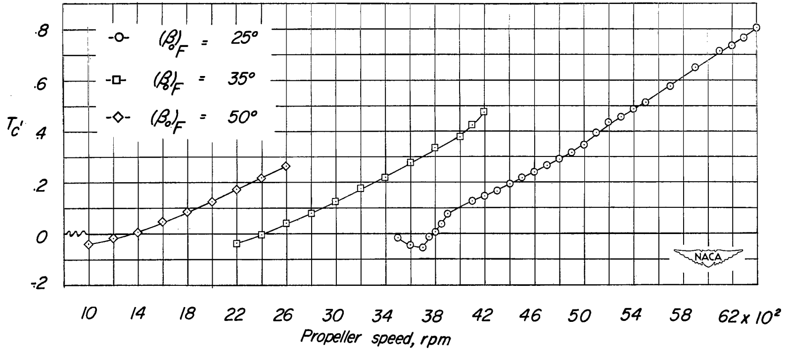
Figure 5.- Variation of thrust coefficient with propeller speed for various propeller-blade angles. \alpha = 0^\circ . q = 16 \text{ lb/sq ft} .
