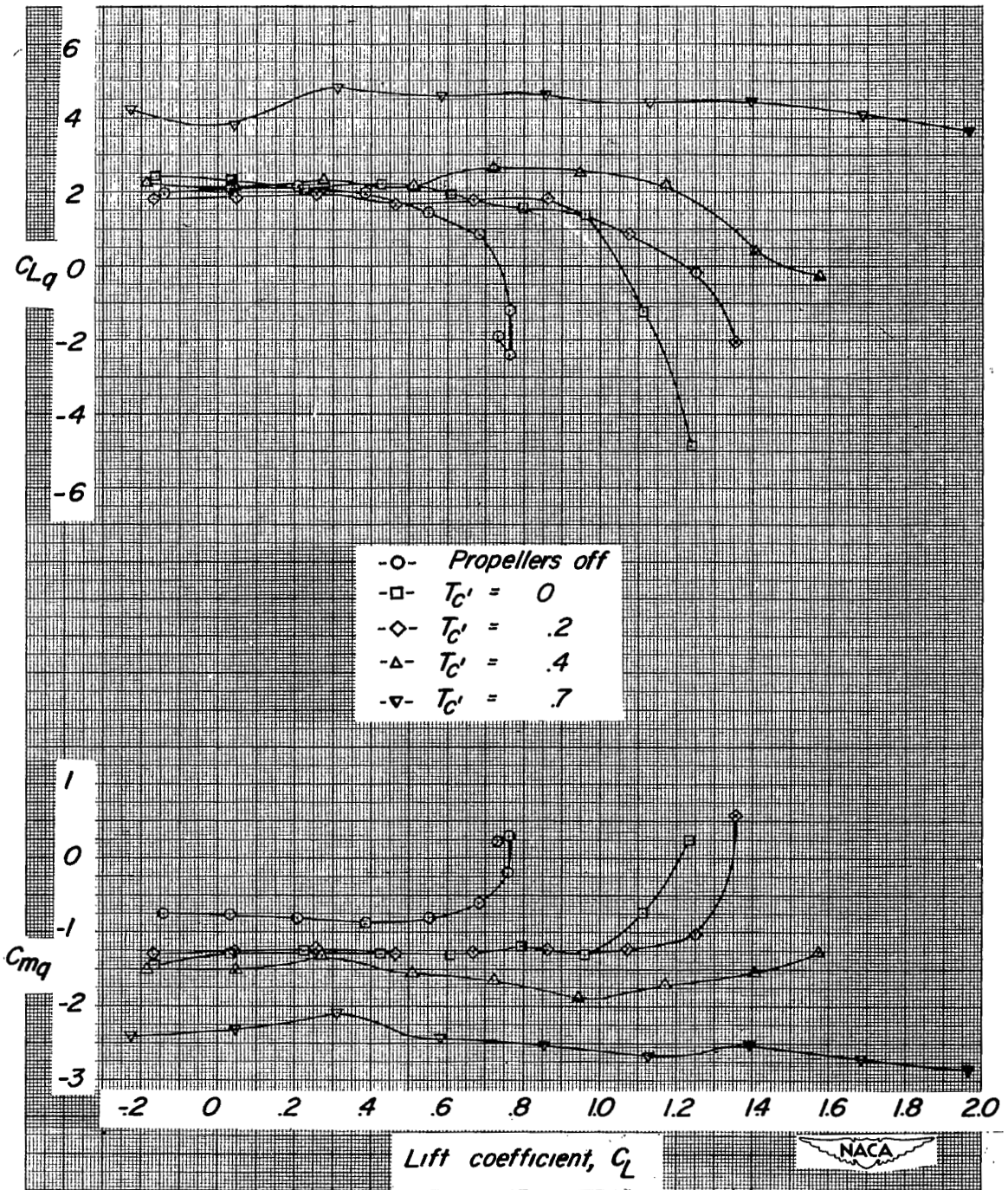
Figure 6.- Effect of thrust coefficient on the pitching stability derivatives of a 1/9-scale powered model of the Convair XFY-1 vertically rising airplane. (\beta_0)_F = 25^\circ .
