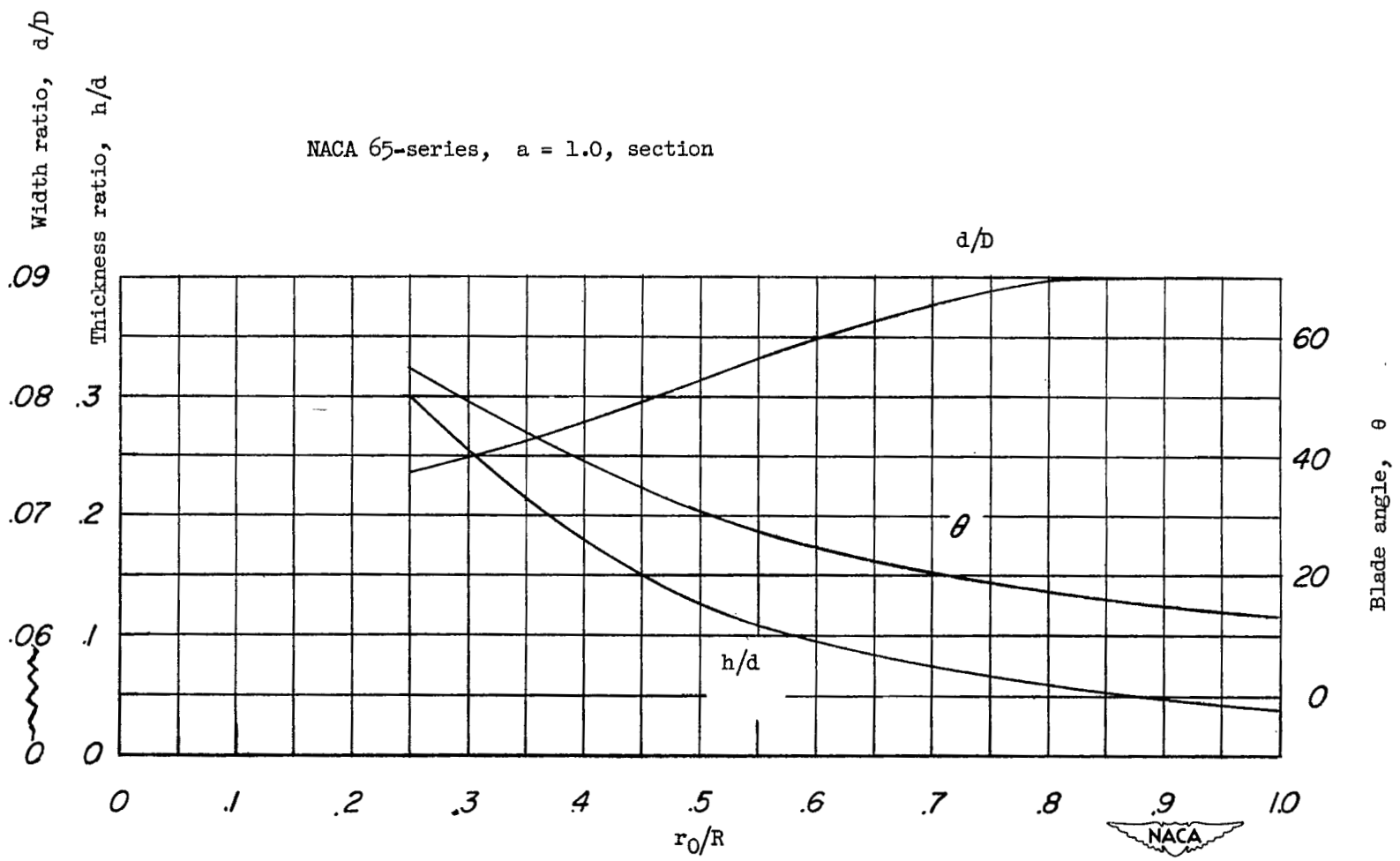
Figure 3.- Geometric characteristics of propeller blades used on a 1/9-scale model of the Convair XFY-1 vertically rising airplane. R = 0.889 foot.
