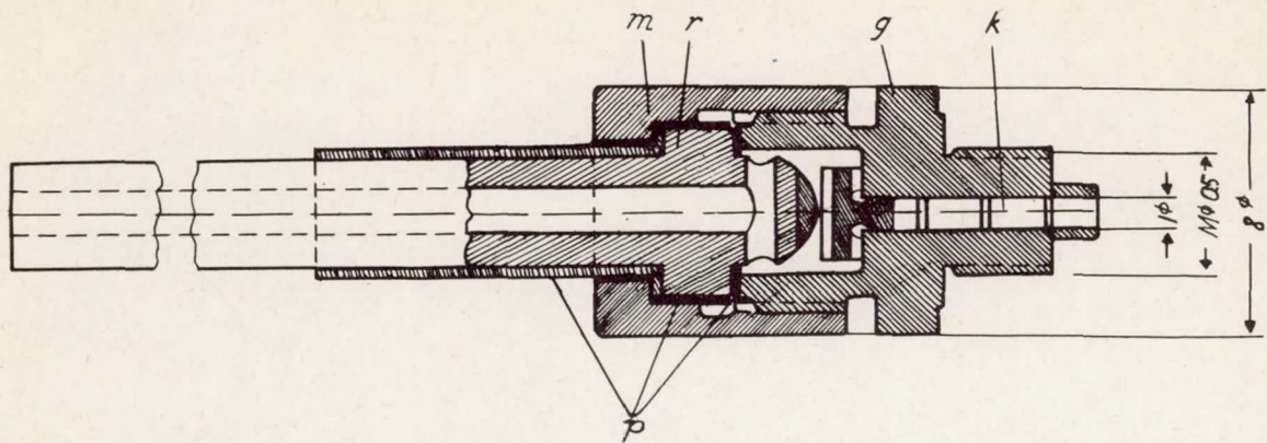
Figure 1.- Pickup for oil film pressure recording device.
