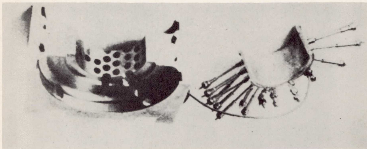
Figure 9.- Experimental bushing and bearing housing.
