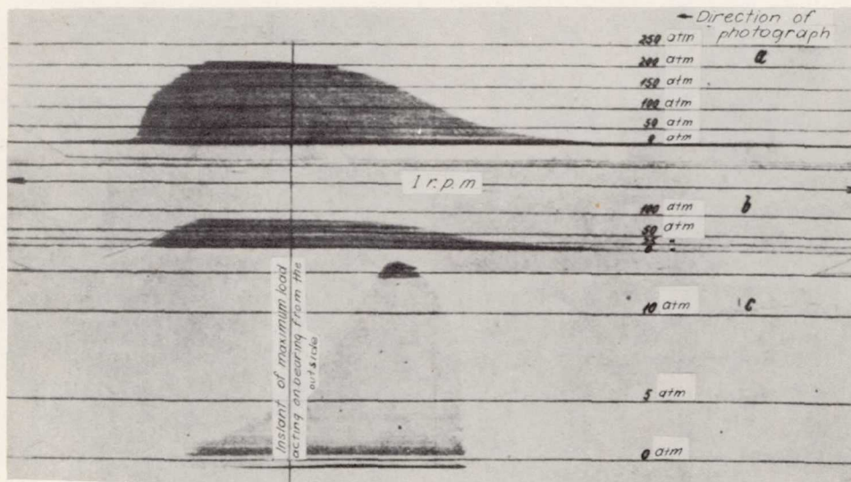
Figure 21a.- Instrument 11. p_{\max} \sim 220 atm.
