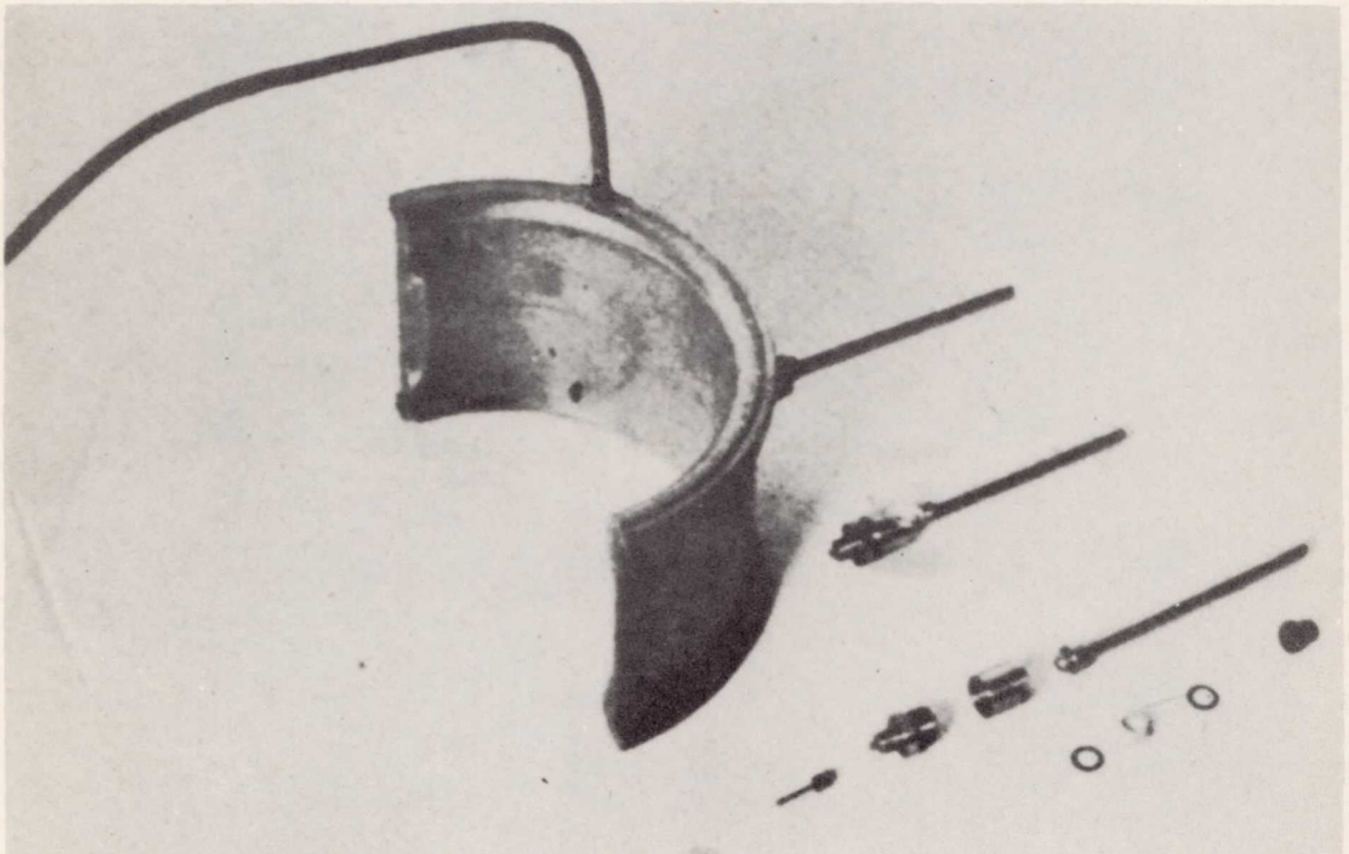
Figure 2.- Pickup for oil film pressure recording device showing exploded view, assembled and mounted in bearing shell.
