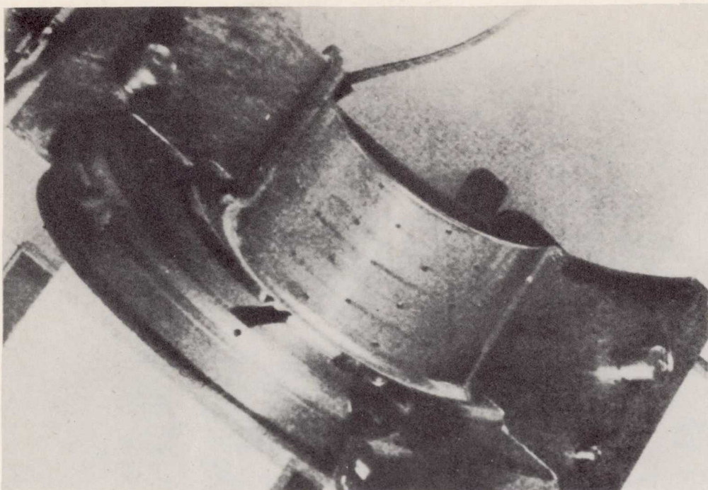
Figure 11.- Upper part of test bearing after 50 hours of operation.
