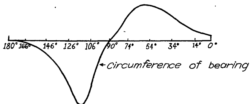
Figure 19e.- Horizontal components of the radial pressures of figure 19a.
