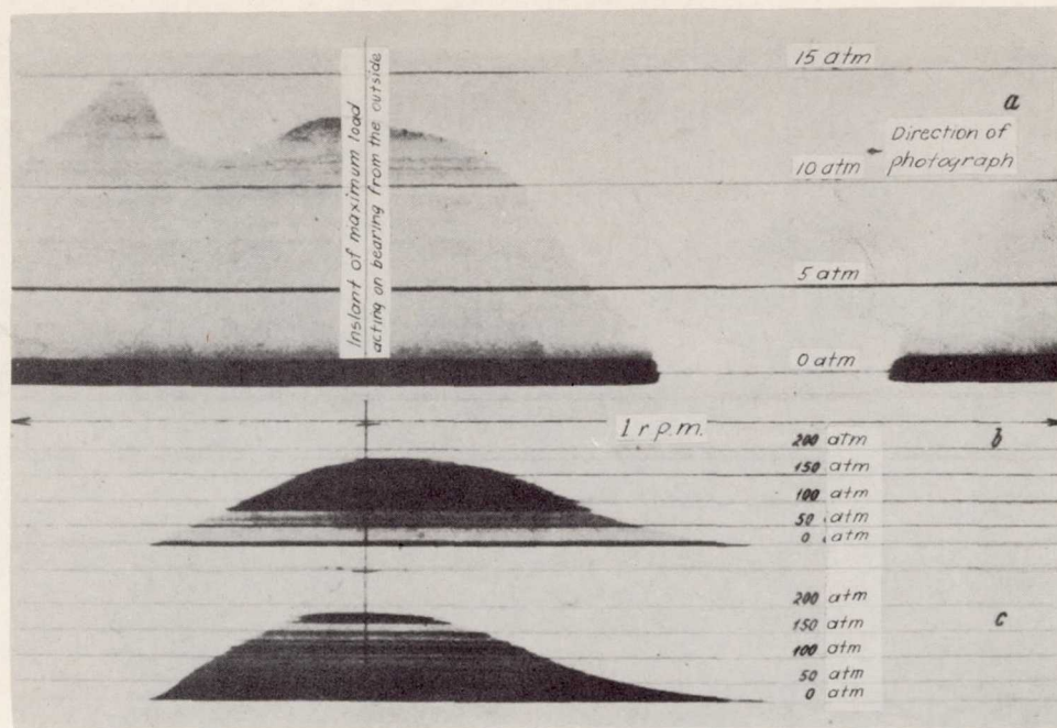
Figure 20a.- Instrument 1. p_{\max} \sim 14.5 atm. Weak spring record.
