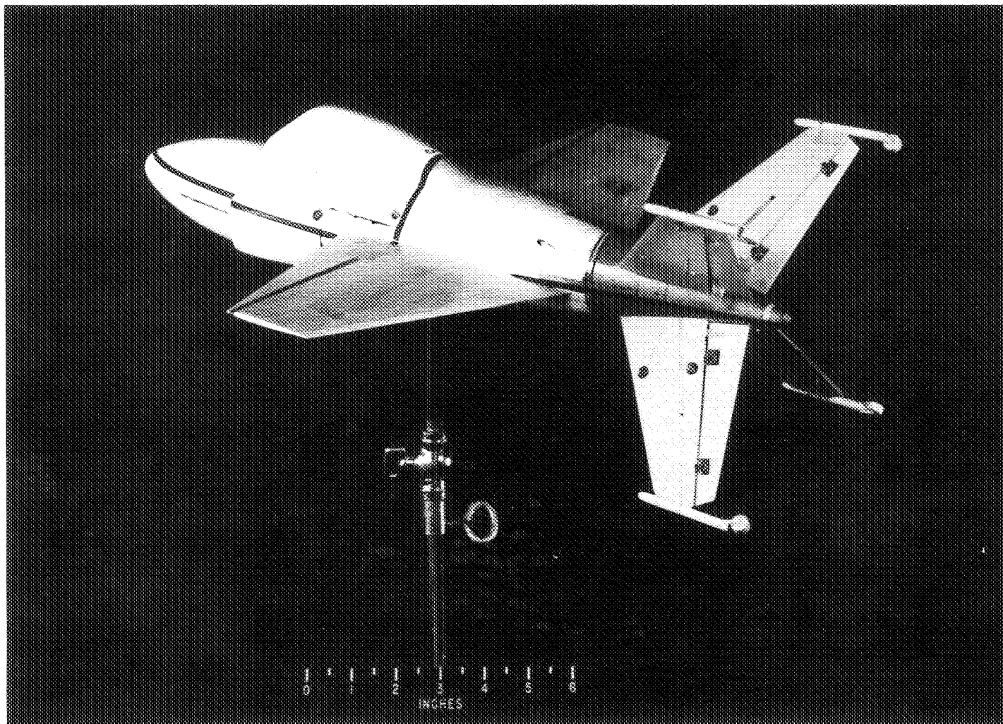
Figure 2.- The 1/25-scale model of the Lockheed XFV-1 airplane with wing-tip pods removed as tested in the Langley 20-foot free-spinning tunnel.
