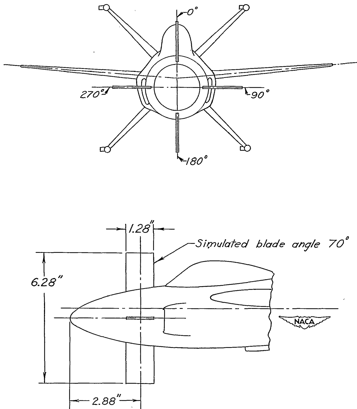
Figure 4.- Drawing of the fin area simulating the propeller as tested on the 1/25-scale model of the Lockheed XFV-1 airplane. Dimensions are model values.
