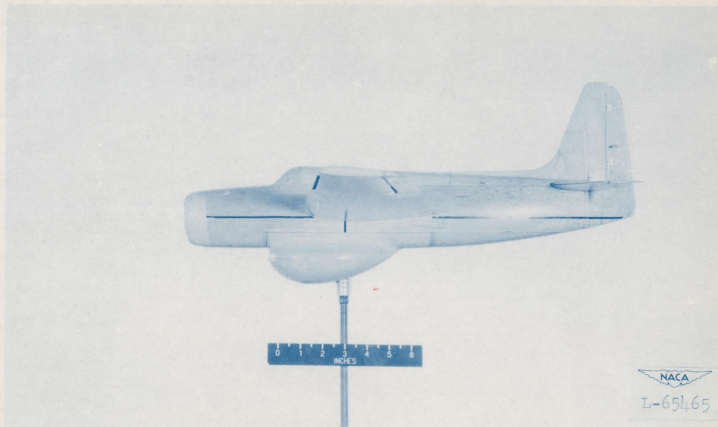
Figure 7.- Photograph of the \frac{1}{24} -scale model of the Grumman AF-2W airplane equipped with the original tail.
