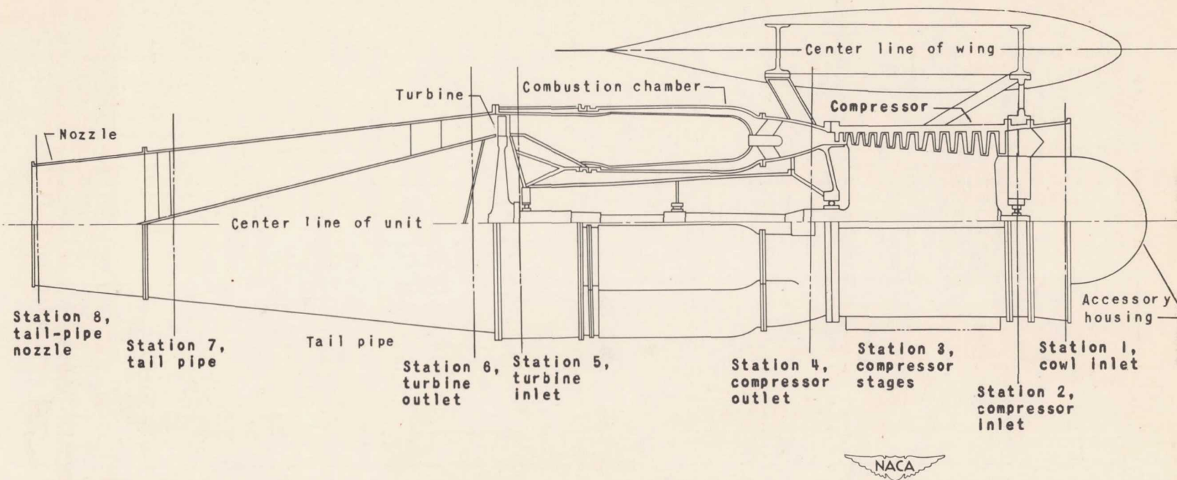
Figure 4. - Side view of 4000-pound-thrust axial flow turbojet installation showing measuring stations.
