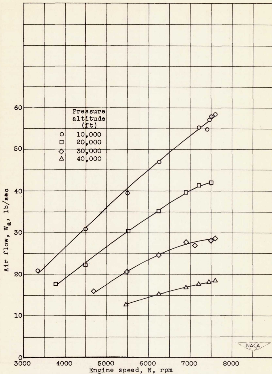
(a) Air flow determined from tail-rake survey at station 8. Figure 12.- Effect of engine speed and altitude on air flow at a ram pressure ratio of approximately 1.2.
