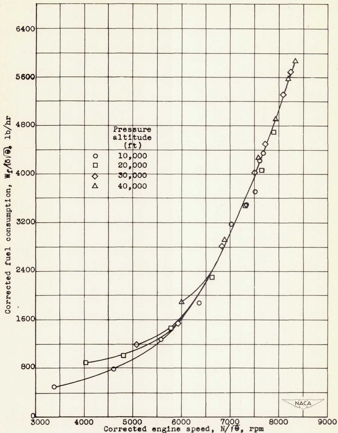
Figure 33. - Effect of corrected engine speed and pressure altitude on corrected fuel consumption at a ram pressure ratio of approximately 1.2. Engine speed and fuel consumption corrected to NACA standard atmospheric conditions at sea level.
