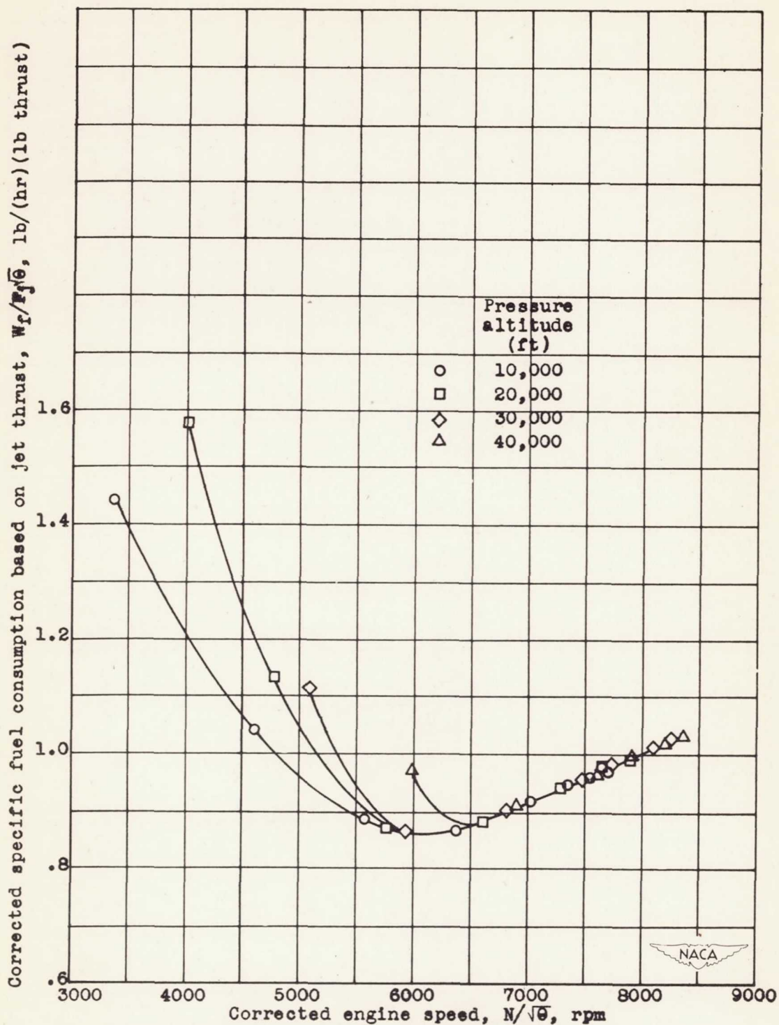
Figure 34. - Effect of corrected engine speed and pressure altitude on corrected specific fuel consumption based on jet thrust at a ram pressure ratio of approximately 1.2. Engine speed and specific fuel consumption corrected to NACA standard atmospheric conditions at sea level.
