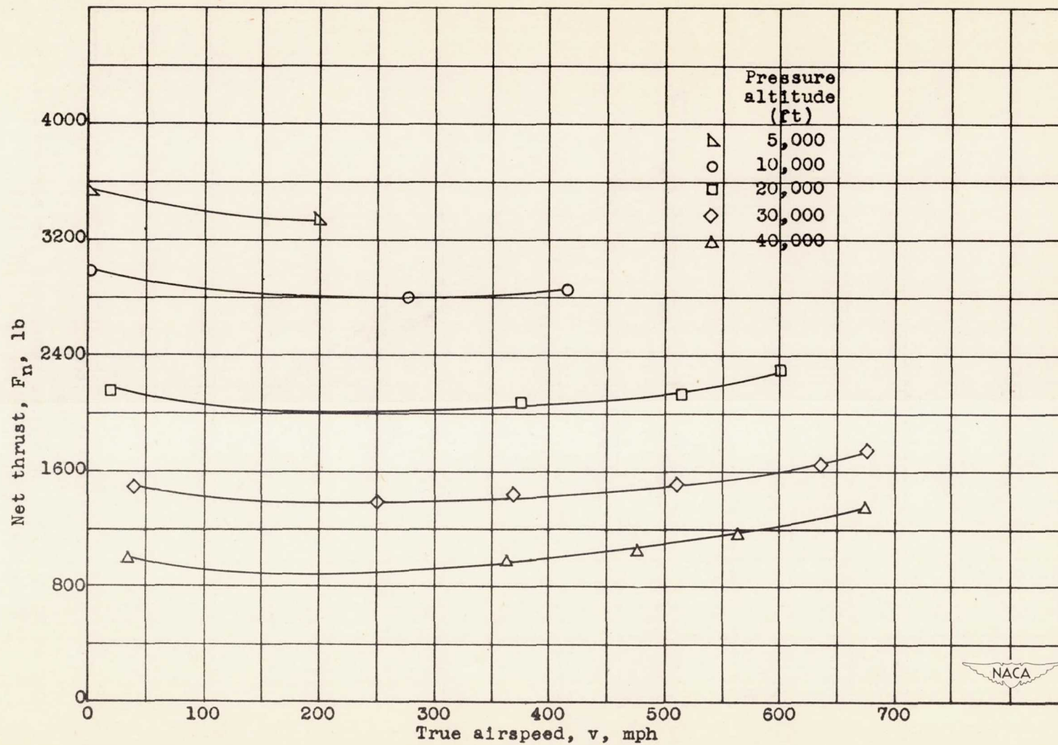
Figure 22.- Variation of net thrust with altitude and true airspeed at an engine speed of 7594 rpm.
