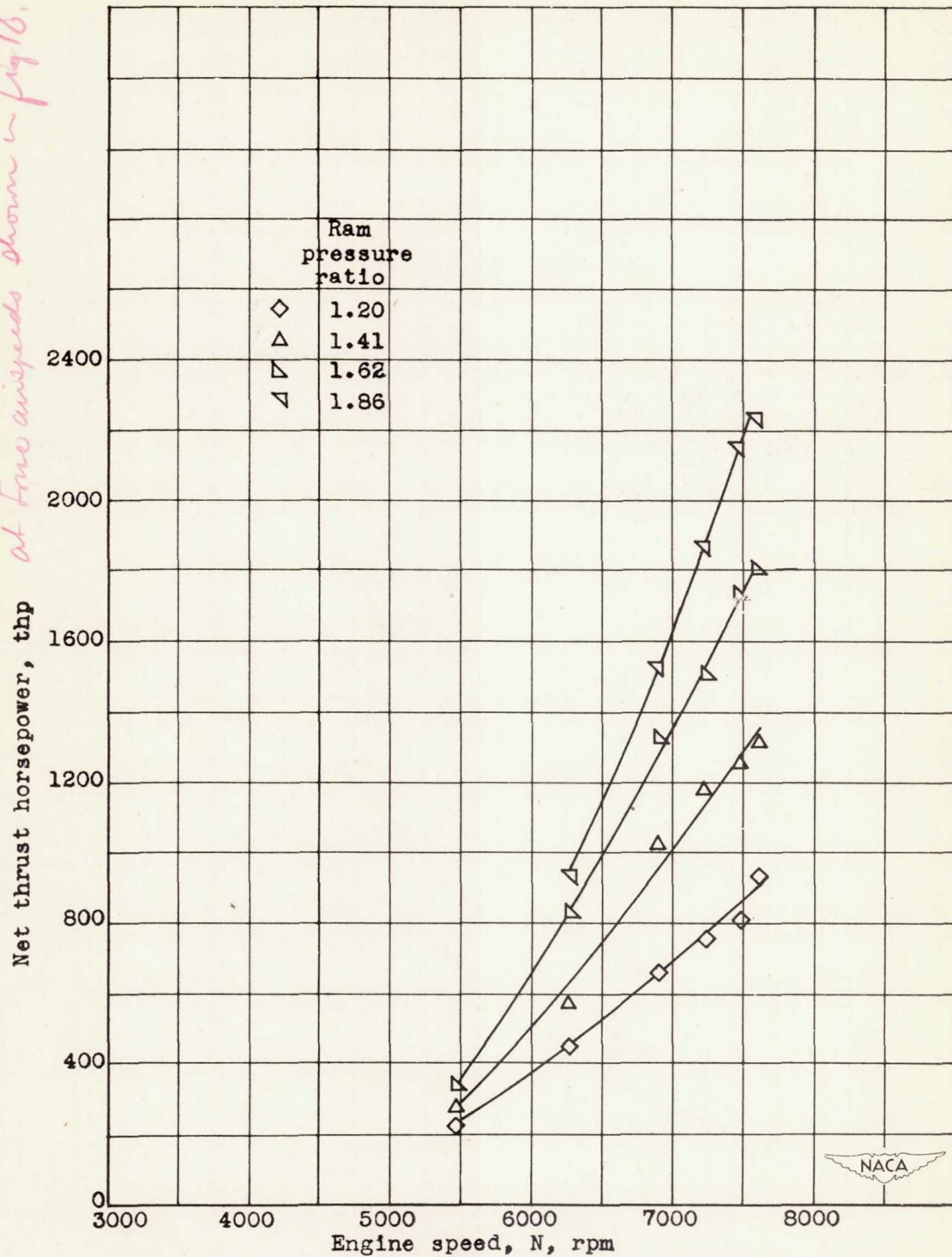
Figure 17.- Effect of engine speed and ram pressure ratio on net thrust horsepower at a pressure altitude of 40,000 feet.
