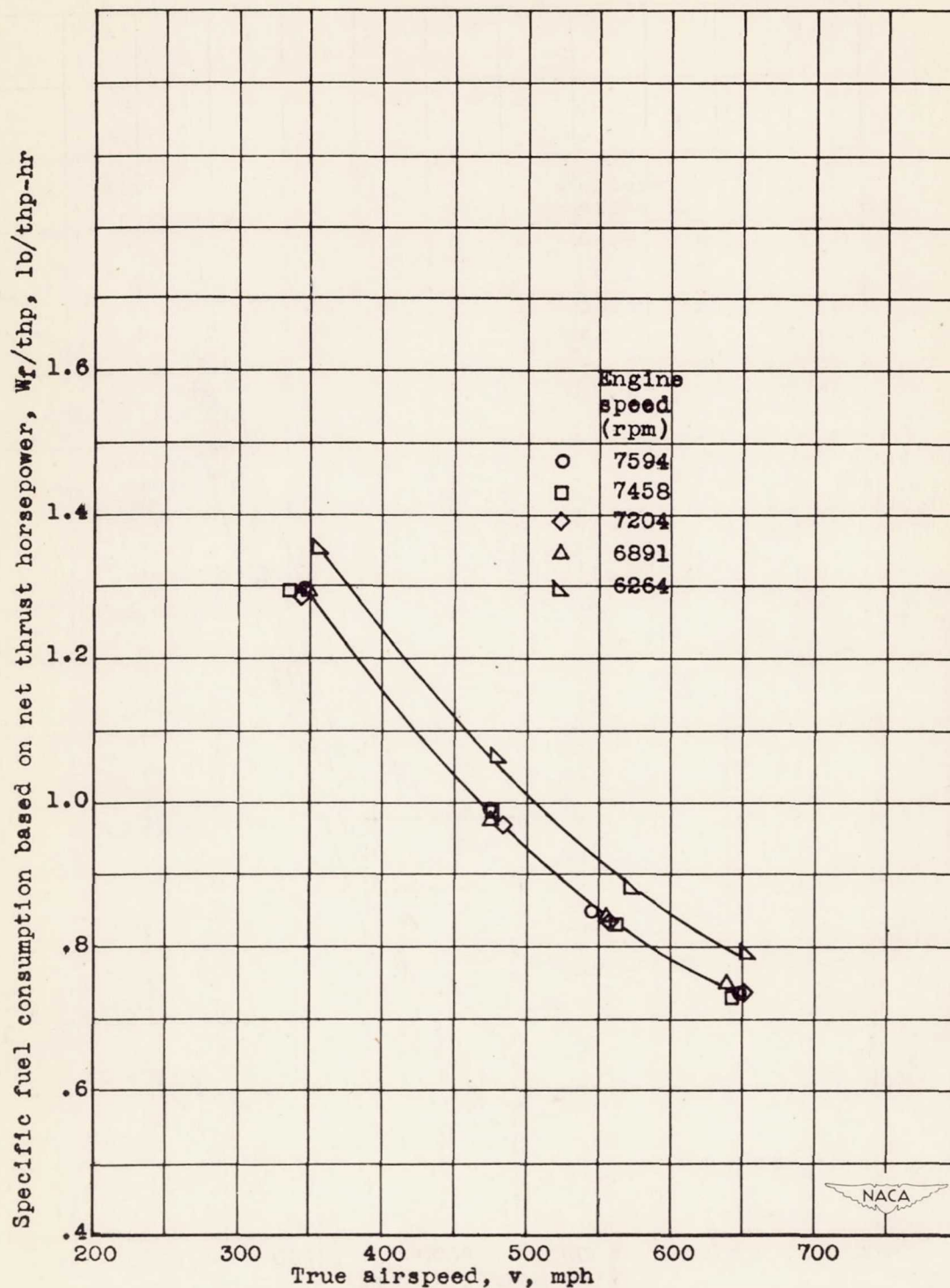
Figure 25.- Variation of specific fuel consumption based on net thrust horsepower with true airspeed for several engine speeds at a pressure altitude of 40,000 feet.
