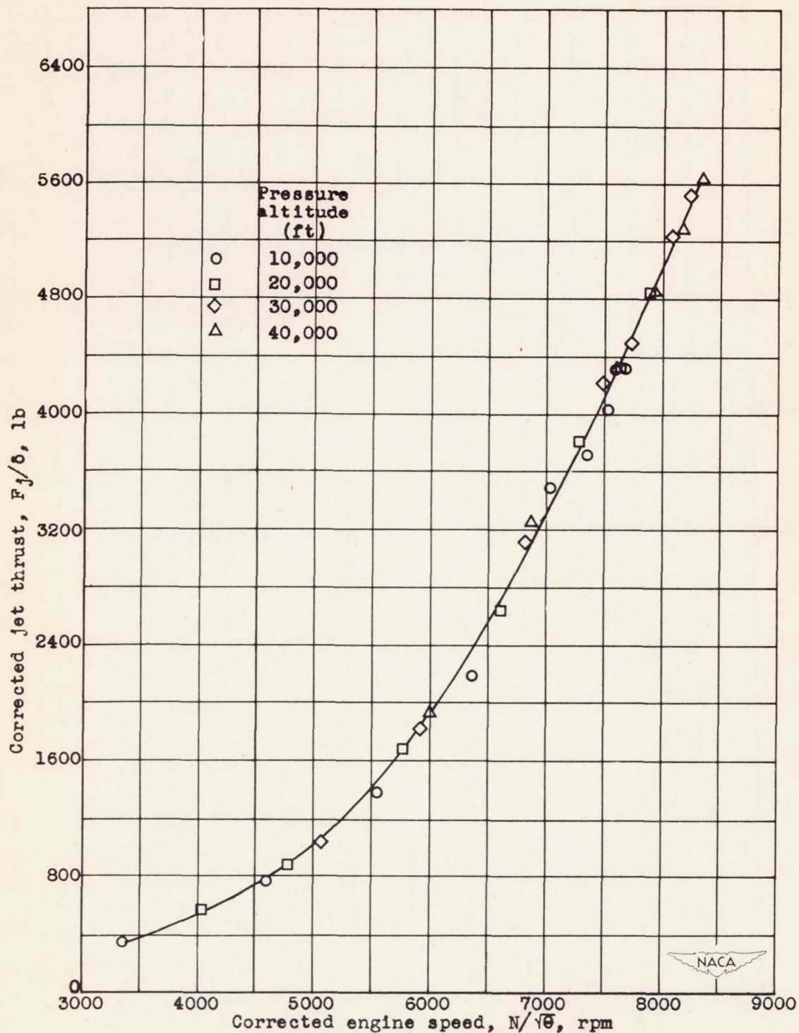
Figure 29. - Effect of corrected engine speed and altitude on corrected jet thrust at a ram pressure ratio of approximately 1.2. Engine speed and jet thrust corrected to NACA standard atmospheric conditions at sea level.
