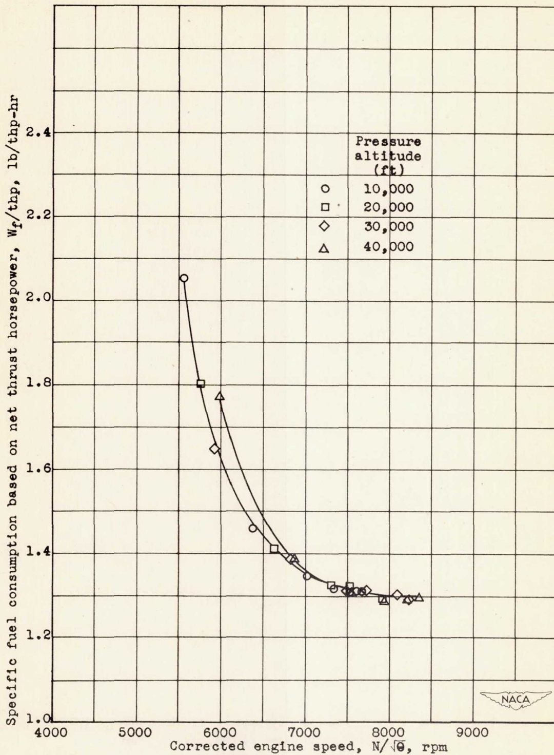
Figure 35. - Effect of corrected engine speed on specific fuel consumption based on net thrust horsepower at a ram pressure ratio of approximately 1.2. Engine speed corrected to NACA standard atmospheric conditions at sea level.
