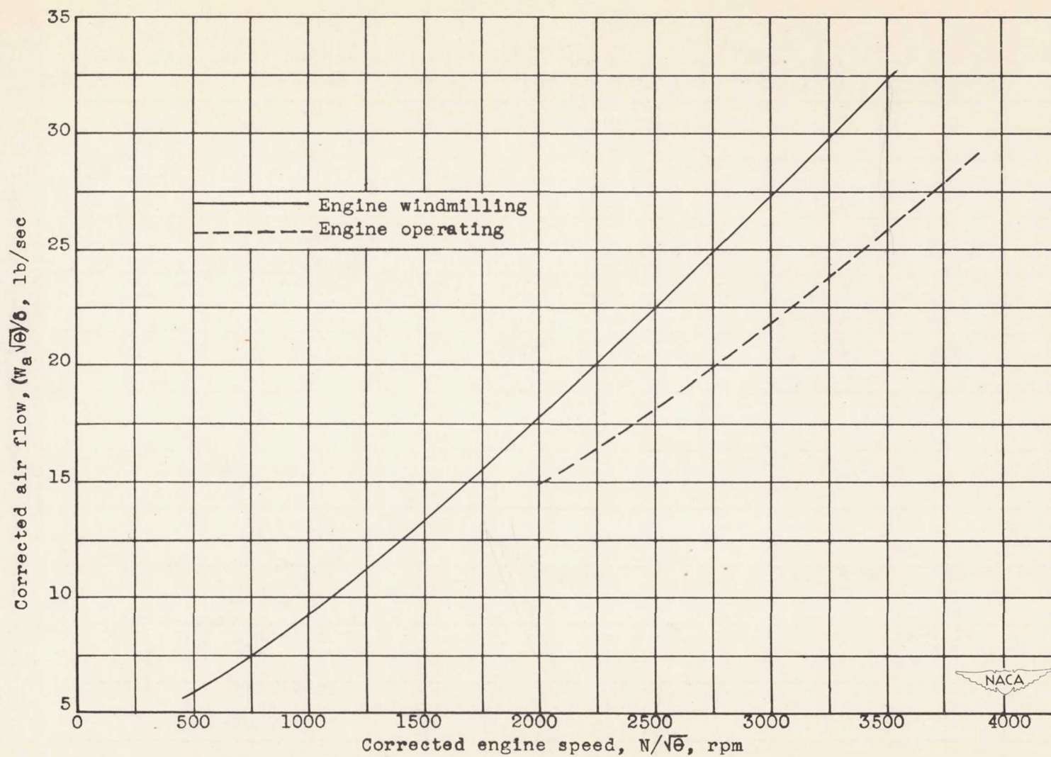
Figure 51. - Comparison of effect of corrected engine speed on corrected air flow with engine windmilling and engine operating. Air flow and engine speed corrected to NACA standard atmospheric conditions at sea level.
