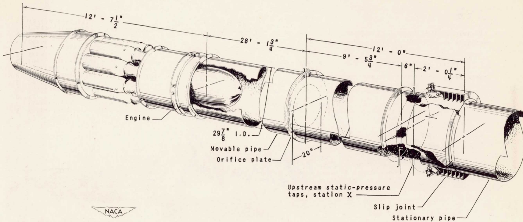
Figure 2. - Installation of closed duct from tunnel make-up air system to engine inlet for supplying air at ram pressures.
