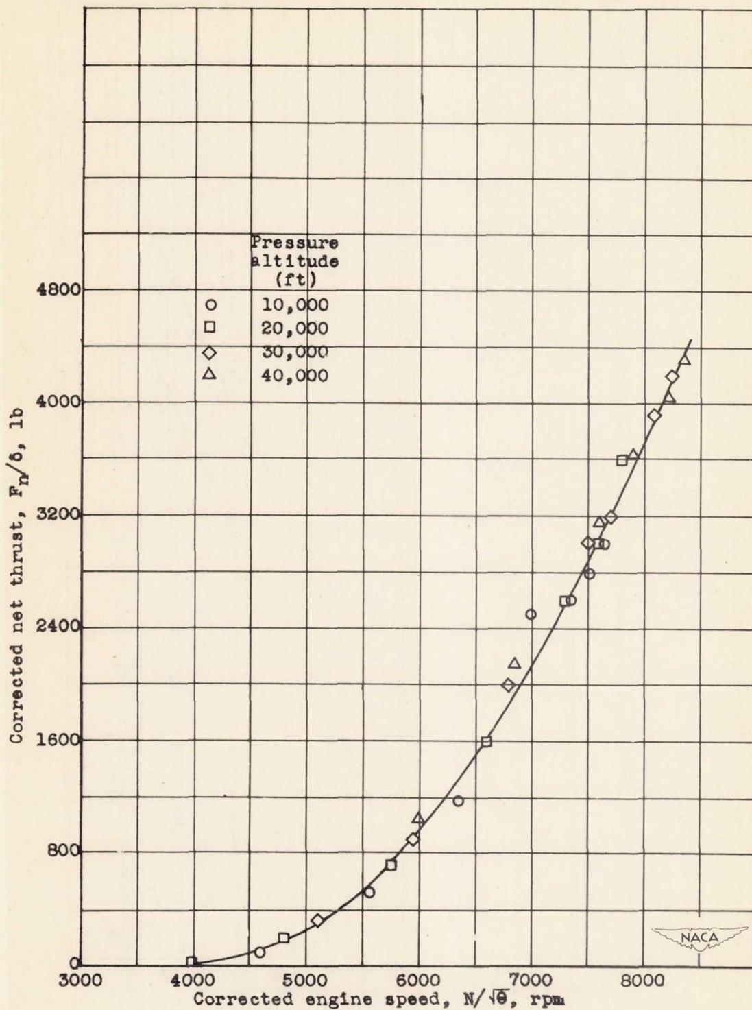
Figure 30. - Effect of corrected engine speed and pressure altitude on corrected net thrust at a ram pressure ratio of approximately 1.2. Engine speed and net thrust corrected to NACA standard atmospheric conditions at sea level.
