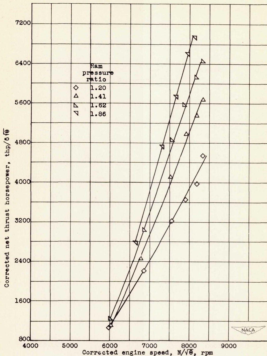
Figure 39. - Effect of corrected engine speed and ram pressure ratio on corrected net thrust horsepower at a pressure altitude of 40,000 feet. Engine speed and net thrust horsepower corrected to NACA standard atmospheric conditions at sea level.
