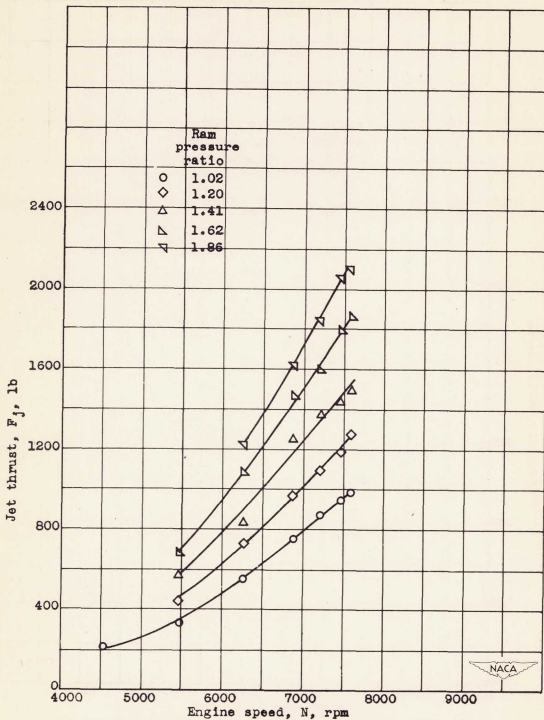
Figure 16.- Effect of engine speed and ram pressure ratio on jet thrust at a pressure altitude of 40,000 feet.
