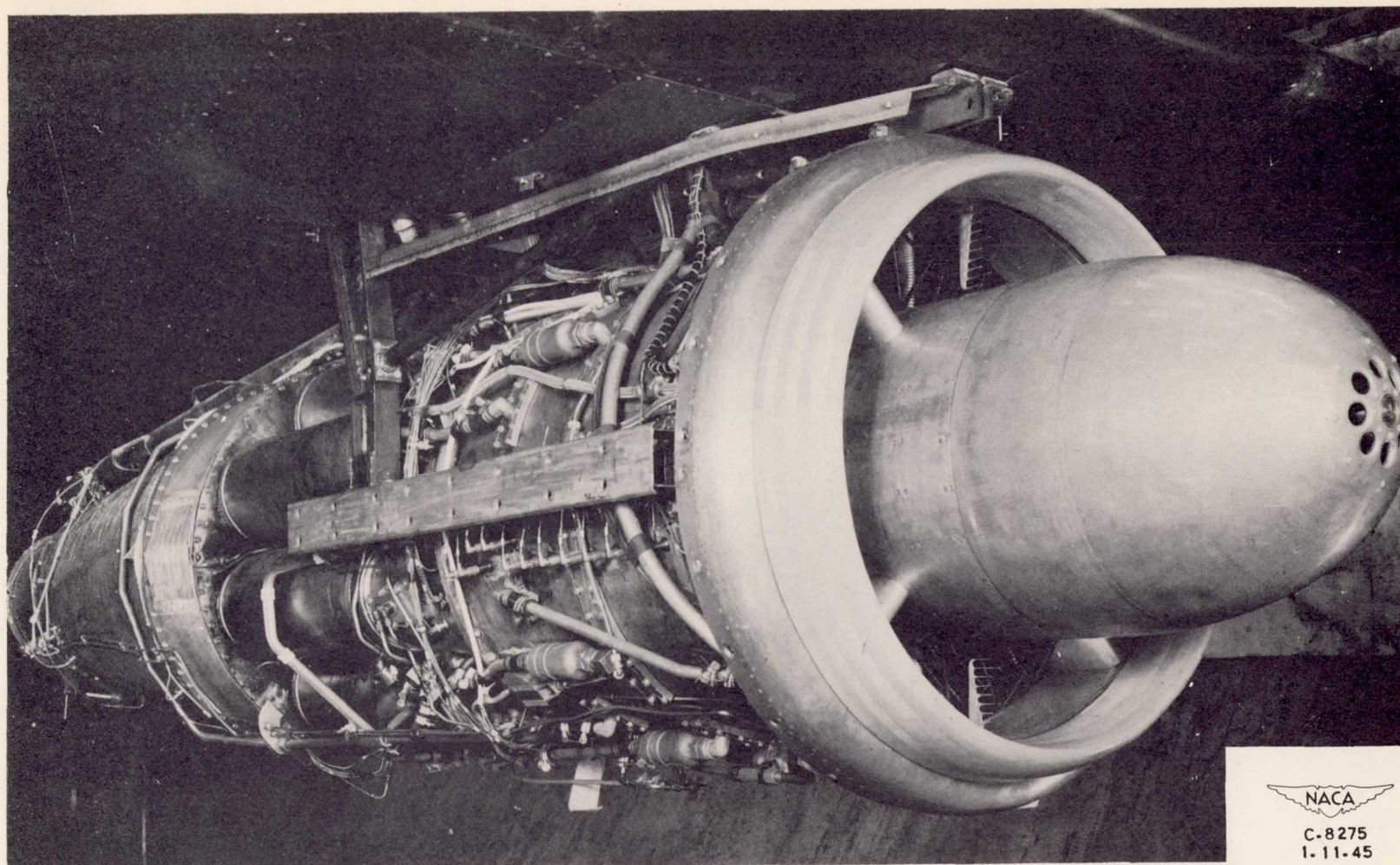
(b) Right-side view without cowling.
