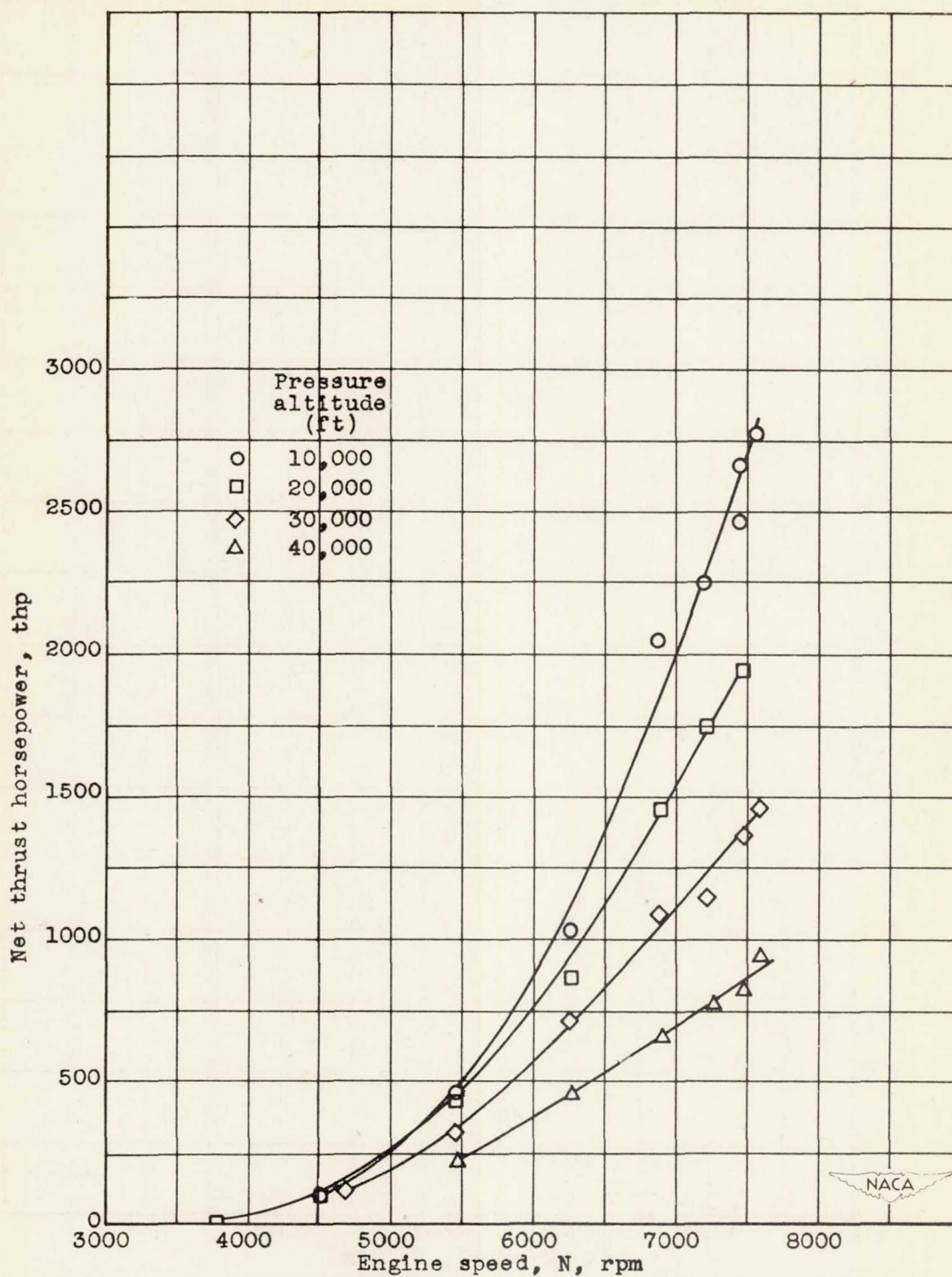
Figure 10.- Effect of engine speed and altitude on net thrust horsepower at a ram pressure ratio of approximately 1.2.
