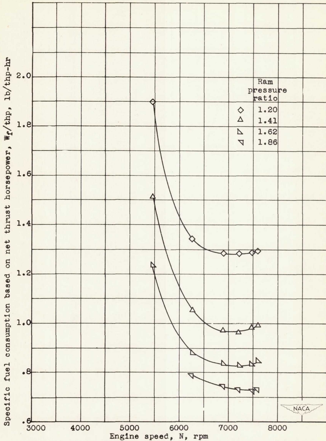
Figure 24.- Effect of engine speed and ram pressure ratio on specific fuel consumption based on net thrust horsepower at a pressure altitude of 40,000 feet.
