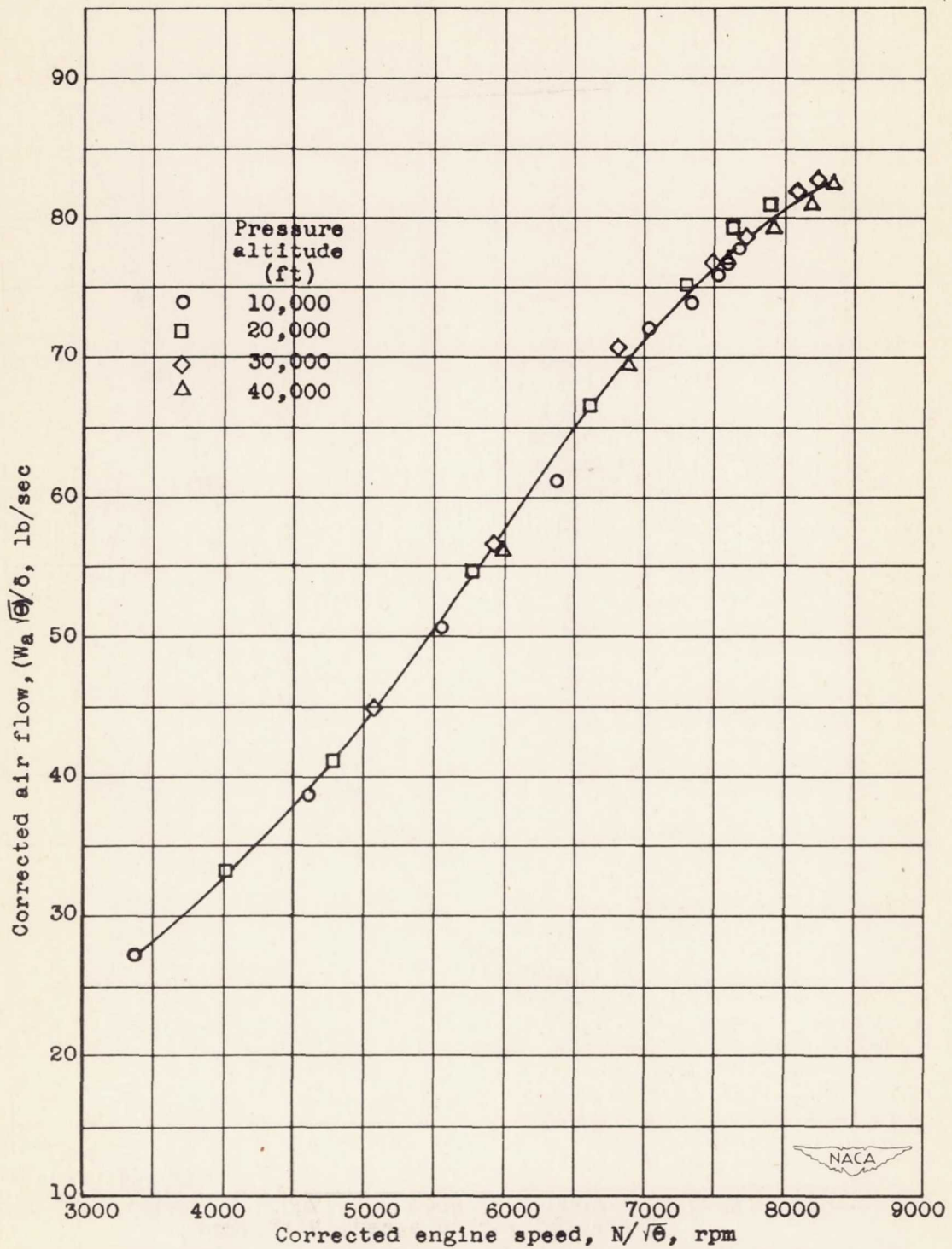
(b) Air flow determined from cowl-inlet survey at station 1. Figure 32.- Concluded.
