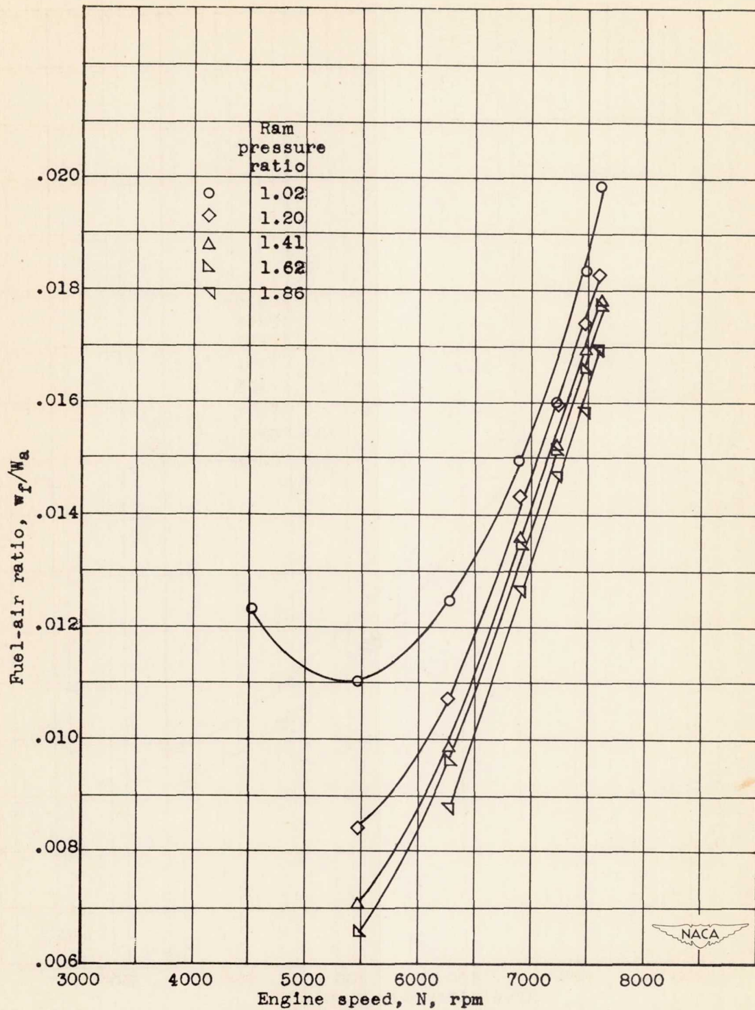
Figure 26.- Effect of engine speed and ram pressure ratio on fuel-air ratio at a pressure altitude of 40,000 feet.
