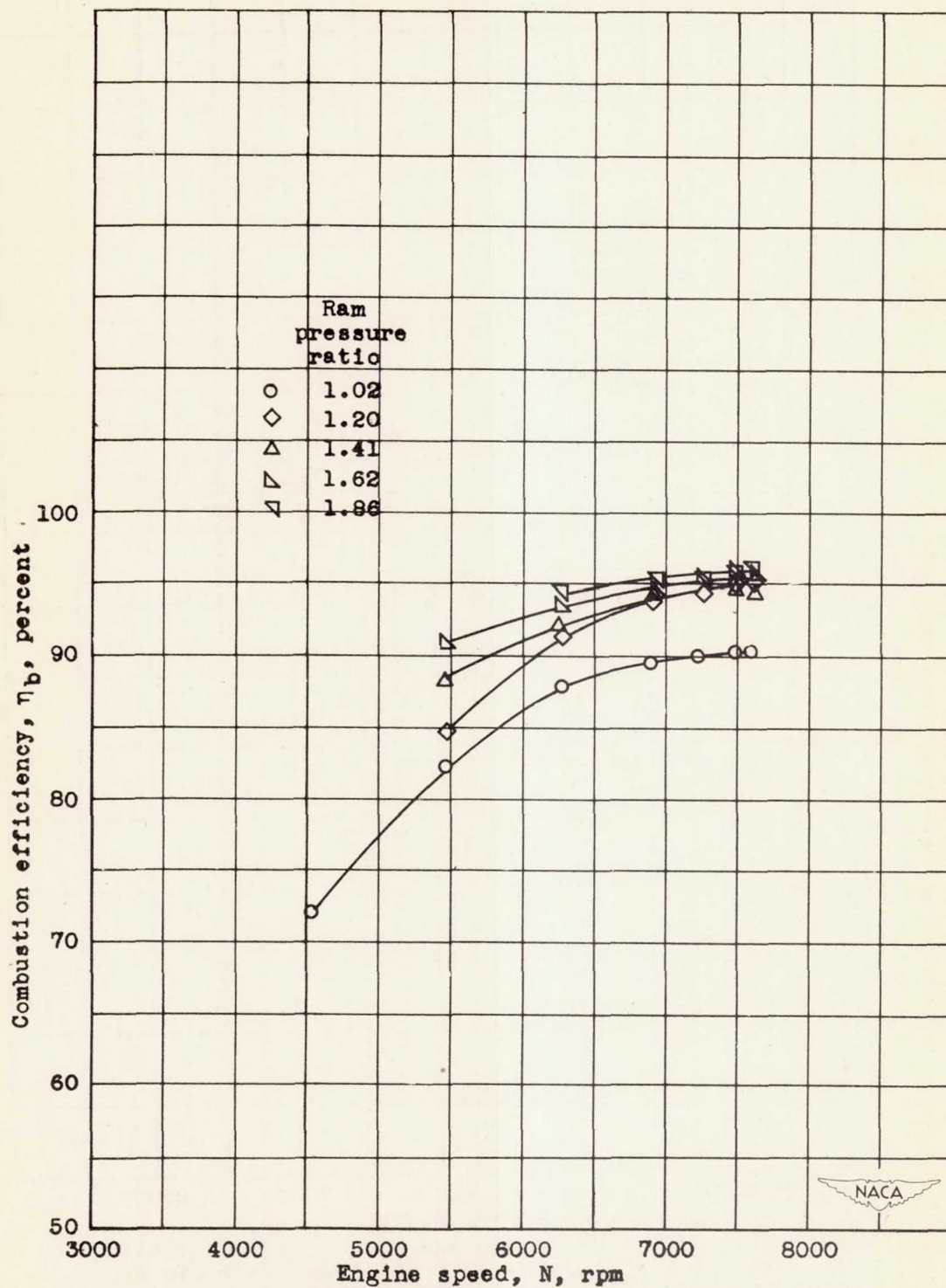
Figure 28.- Effect of engine speed and ram pressure ratio on combustion efficiency at a pressure altitude of 40,000 feet.
