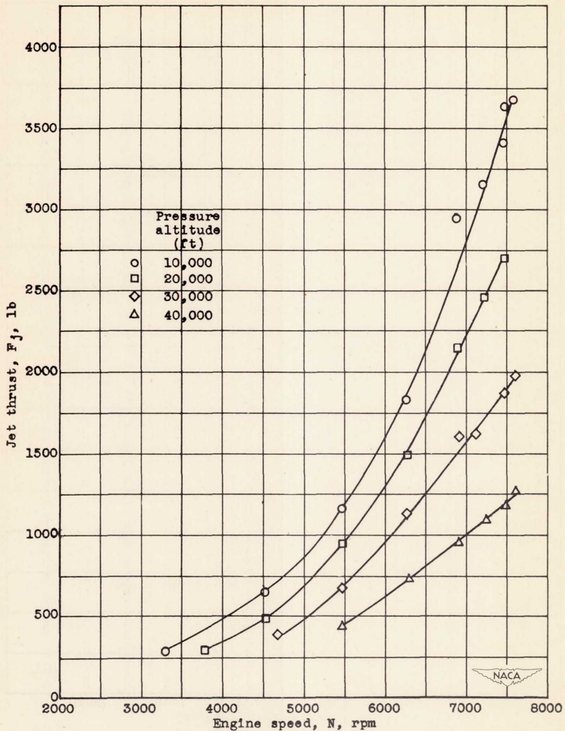
Figure 8.- Effect of engine speed and altitude on jet thrust at a ram pressure ratio of approximately 1.2.
