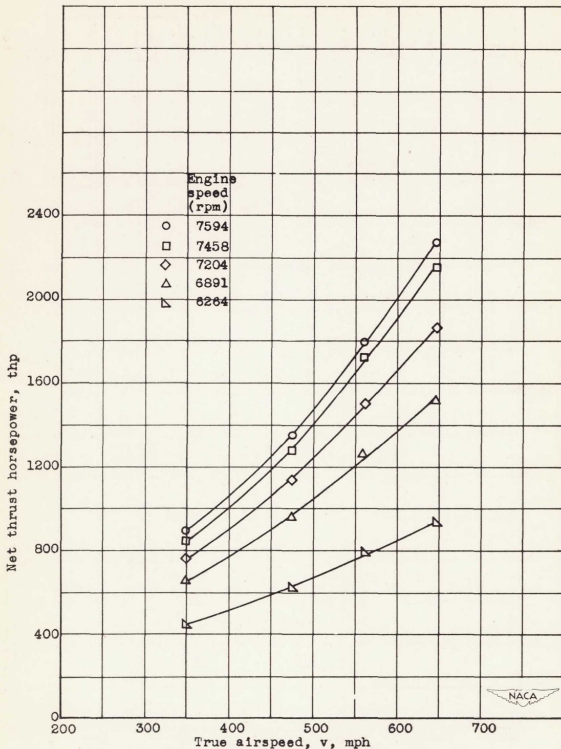
Figure 18.- Variation of net thrust horsepower with true airspeed for several engine speeds at a pressure altitude of 40,000 feet.
