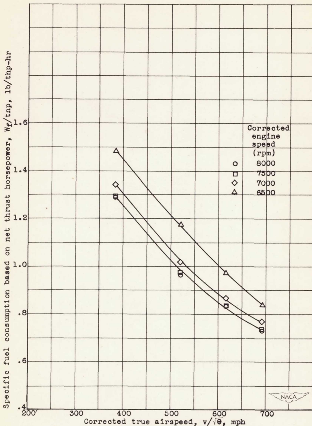
Figure 44. - Variation of specific fuel consumption based on net thrust horsepower with corrected true airspeed at various corrected engine speeds and a pressure altitude of 40,000 feet. True airspeed corrected to NACA standard atmospheric conditions at sea level.
