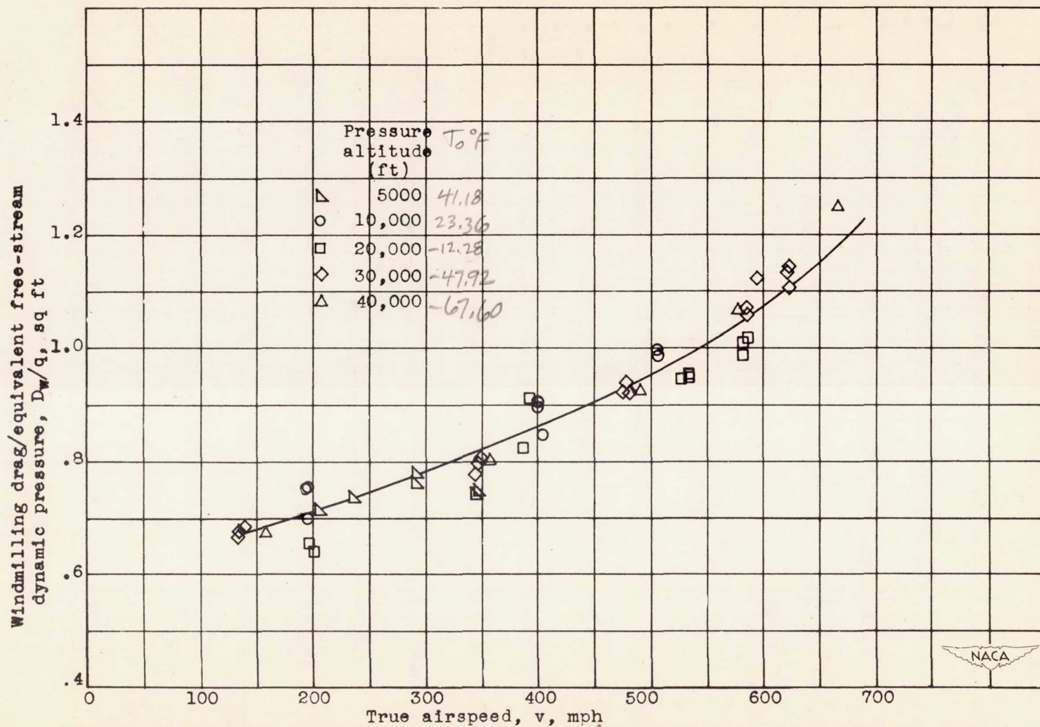
Figure 50.- Effect of altitude and true airspeed on the ratio of windmilling drag to equivalent free-stream dynamic pressure.
