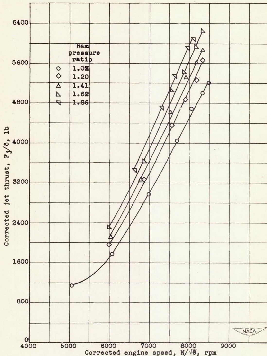
Figure 37. - Effect of corrected engine speed and ram pressure ratio on corrected jet thrust at a pressure altitude of 40,000 feet. Engine speed and jet thrust corrected to NACA standard atmospheric conditions at sea level.
