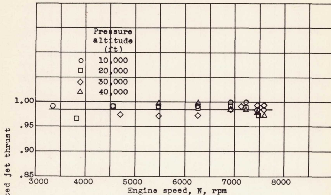
Figure 6.- Ratio of measured jet thrust to calculated jet thrust for various engine speeds and altitudes at a ram pressure ratio of 1.2.
