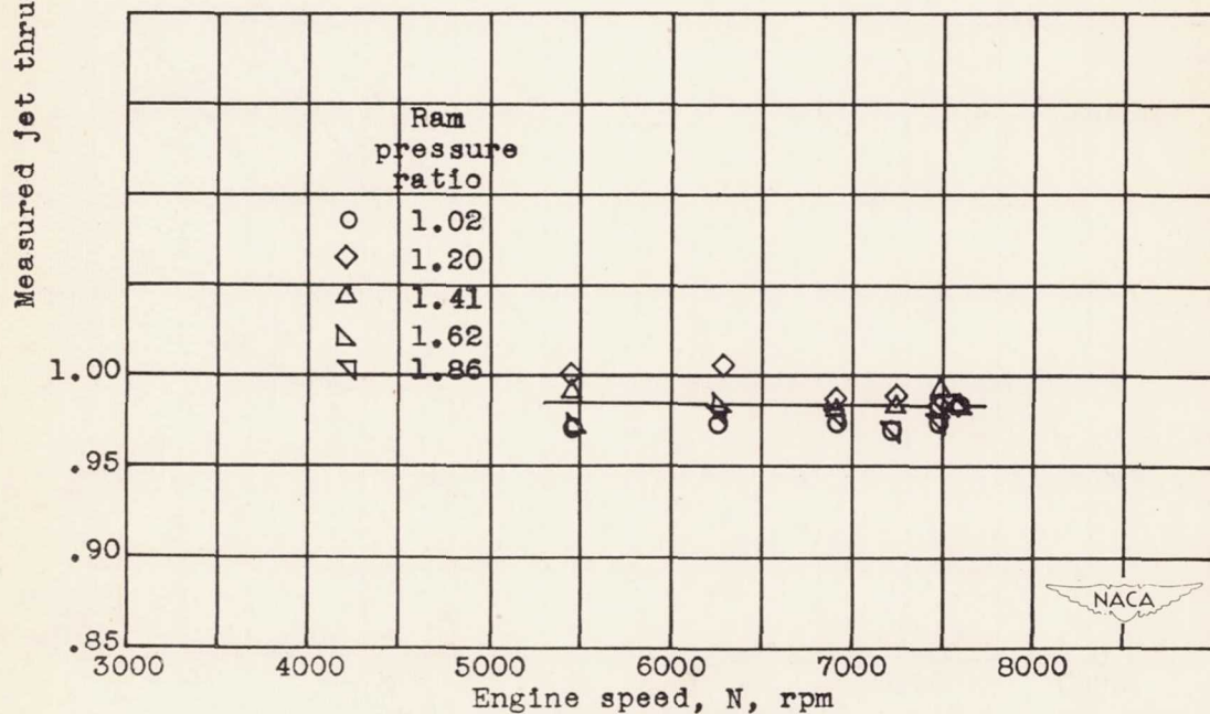
Figure 7.- Ratio of measured jet thrust to calculated jet thrust for various engine speeds and ram pressure ratios at an altitude of 40,000 feet.
