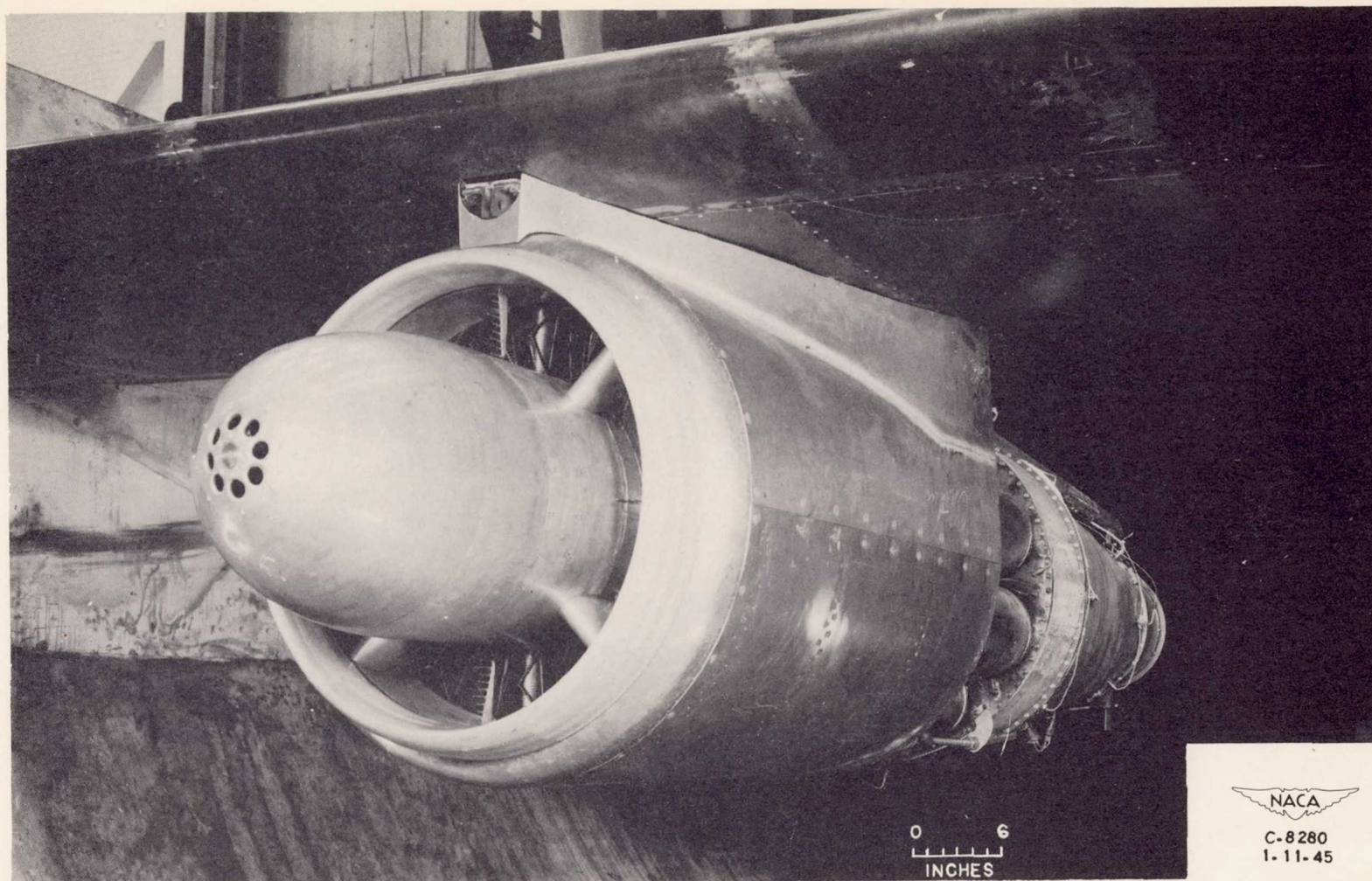
(a) Left-side view with cowling.
