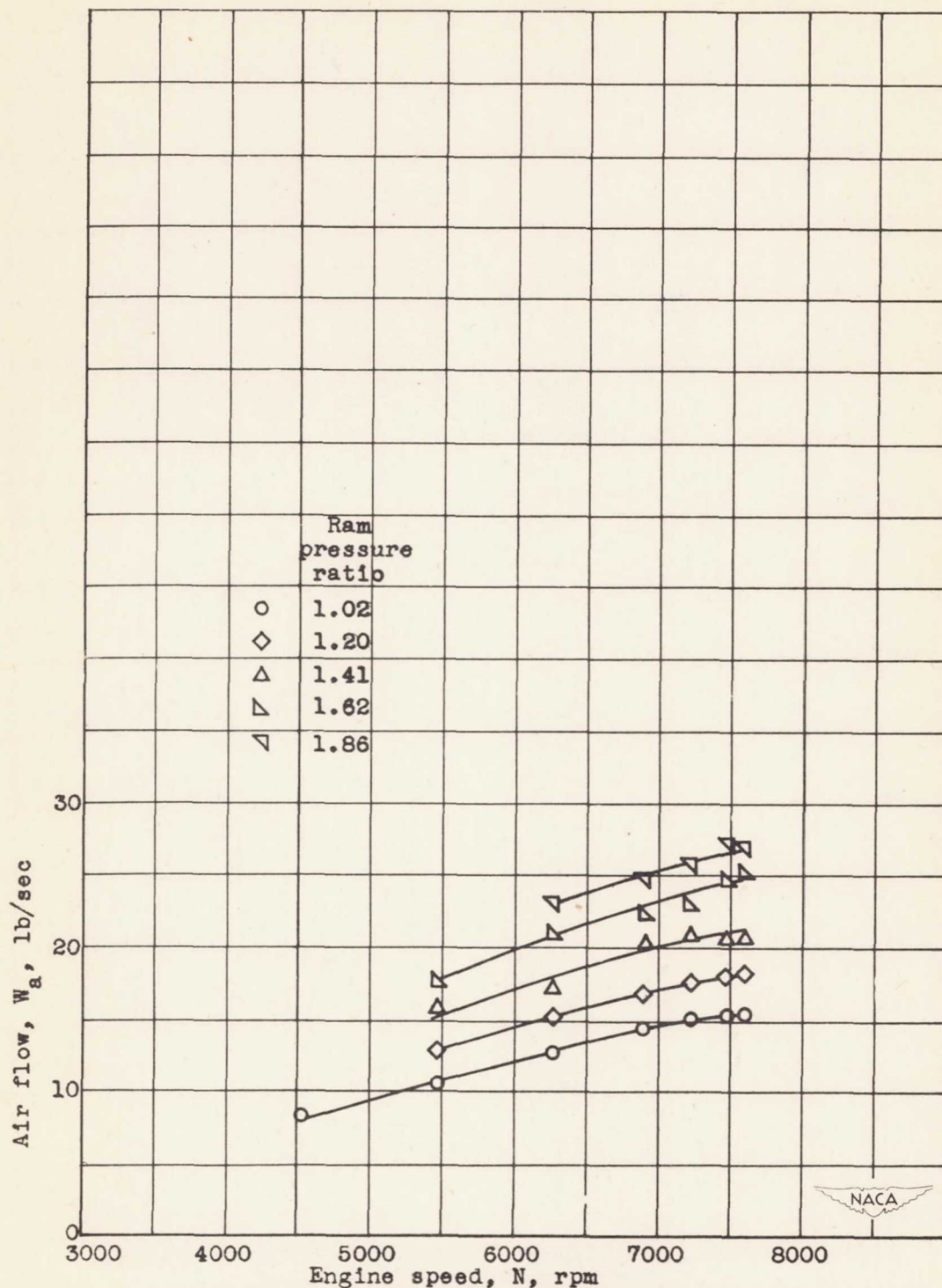
(a) Air flow determined from tail-rake survey at station 8. Figure 20.- Effect of engine speed and ram pressure ratio on air flow at a pressure altitude of 40,000 feet.
