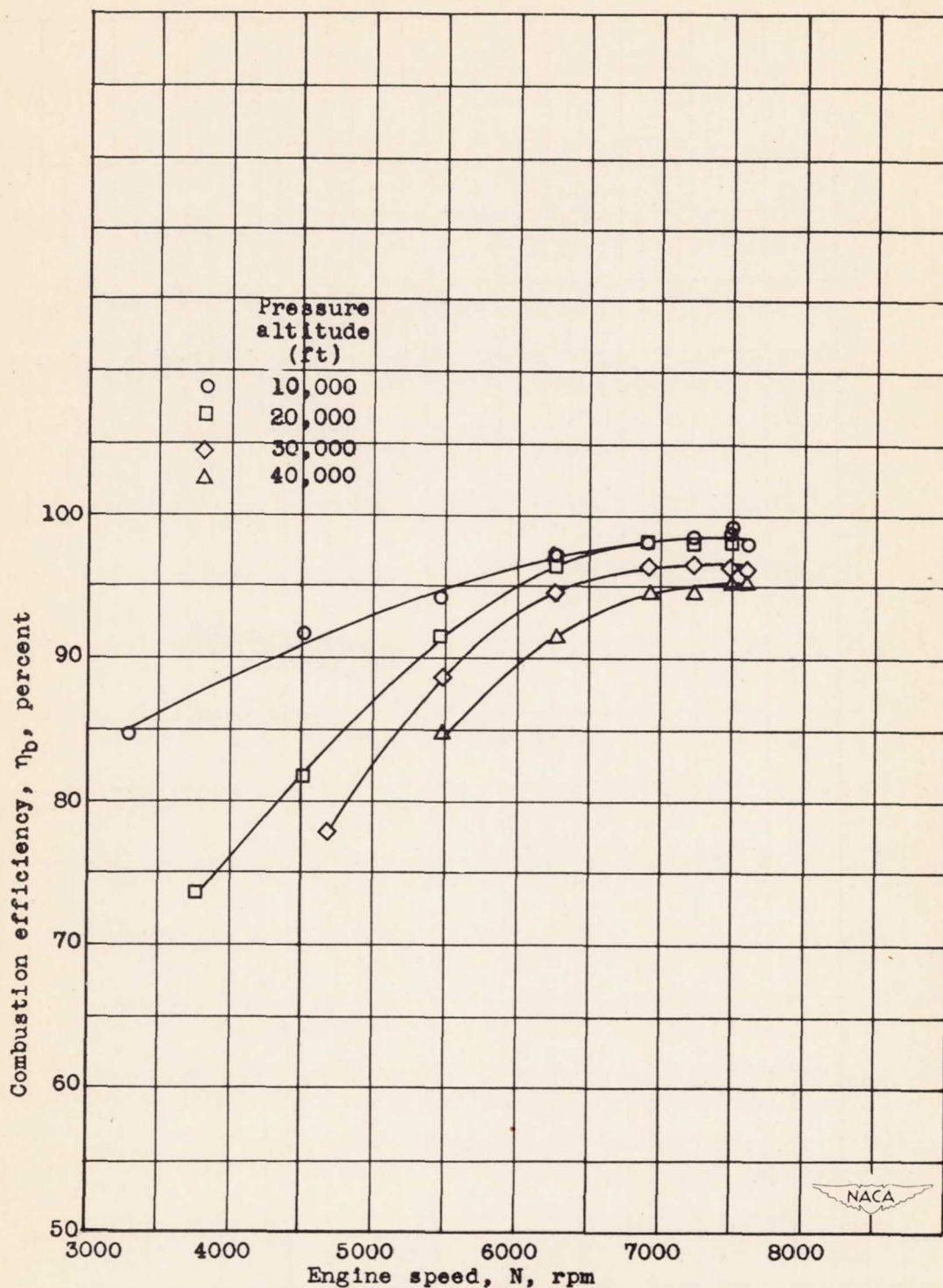
Figure 27.- Effect of engine speed and pressure altitude on combustion efficiency at a ram pressure ratio of approximately 1.2.
