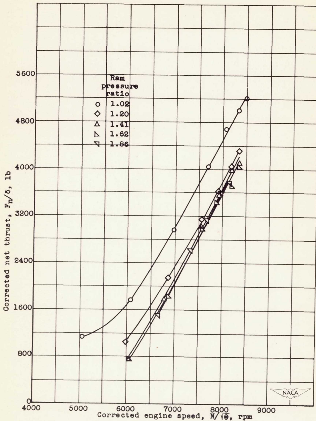
Figure 38. - Effect of corrected engine speed and ram pressure ratio on corrected net thrust at a pressure altitude of 40,000 feet. Engine speed and net thrust corrected to NACA standard atmospheric conditions at sea level.
