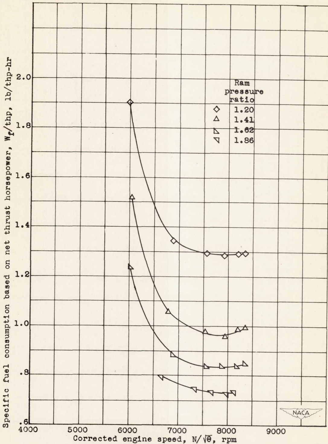
Figure 43. - Effect of corrected engine speed and ram pressure ratio on specific fuel consumption based on net thrust horsepower at a pressure altitude of 40,000 feet. Engine speed corrected to NACA standard atmospheric conditions at sea level.
