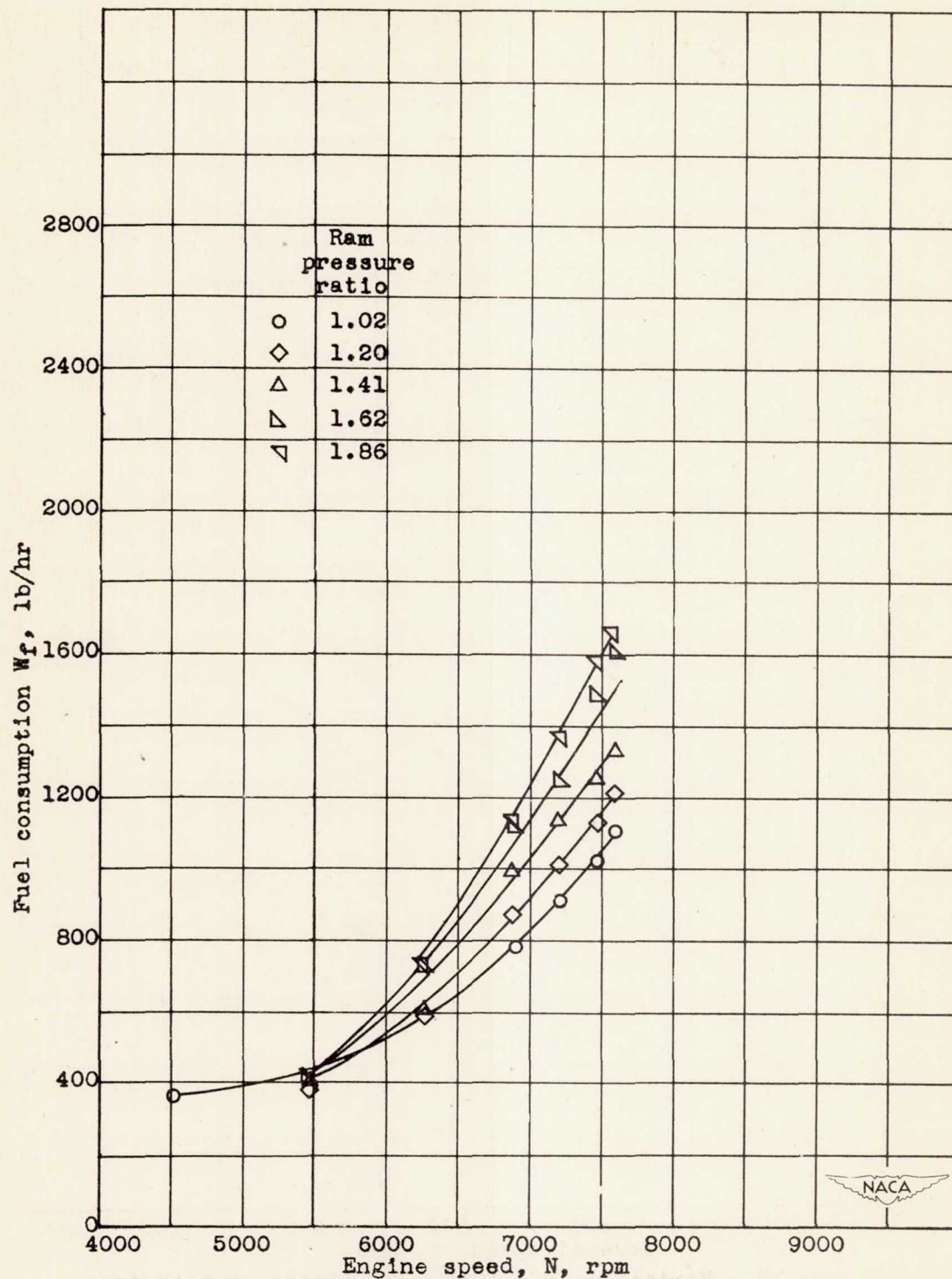
Figure 19.- Effect of engine speed and ram pressure ratio on fuel consumption at a pressure altitude of 40,000 feet.
