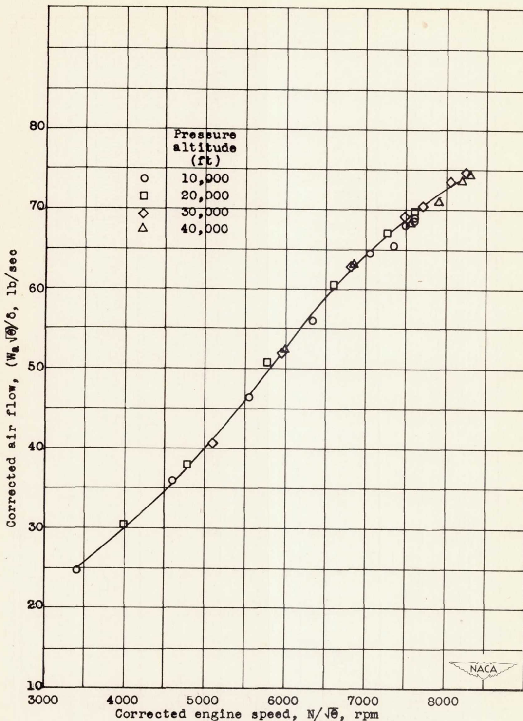
(a) Air flow determined from tail-rake survey at station 8.
