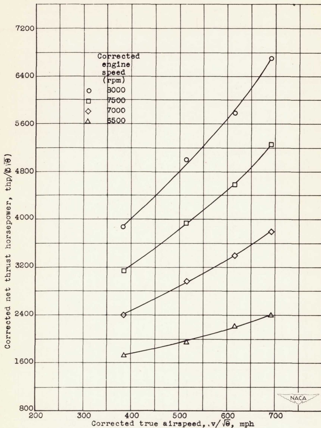
Figure 40. - Variation of corrected net thrust horsepower with corrected true airspeed at various corrected engine speeds and a pressure altitude of 40,000 feet. Net thrust horsepower, engine speed, and true airspeed corrected to NACA standard atmospheric conditions at sea level.
