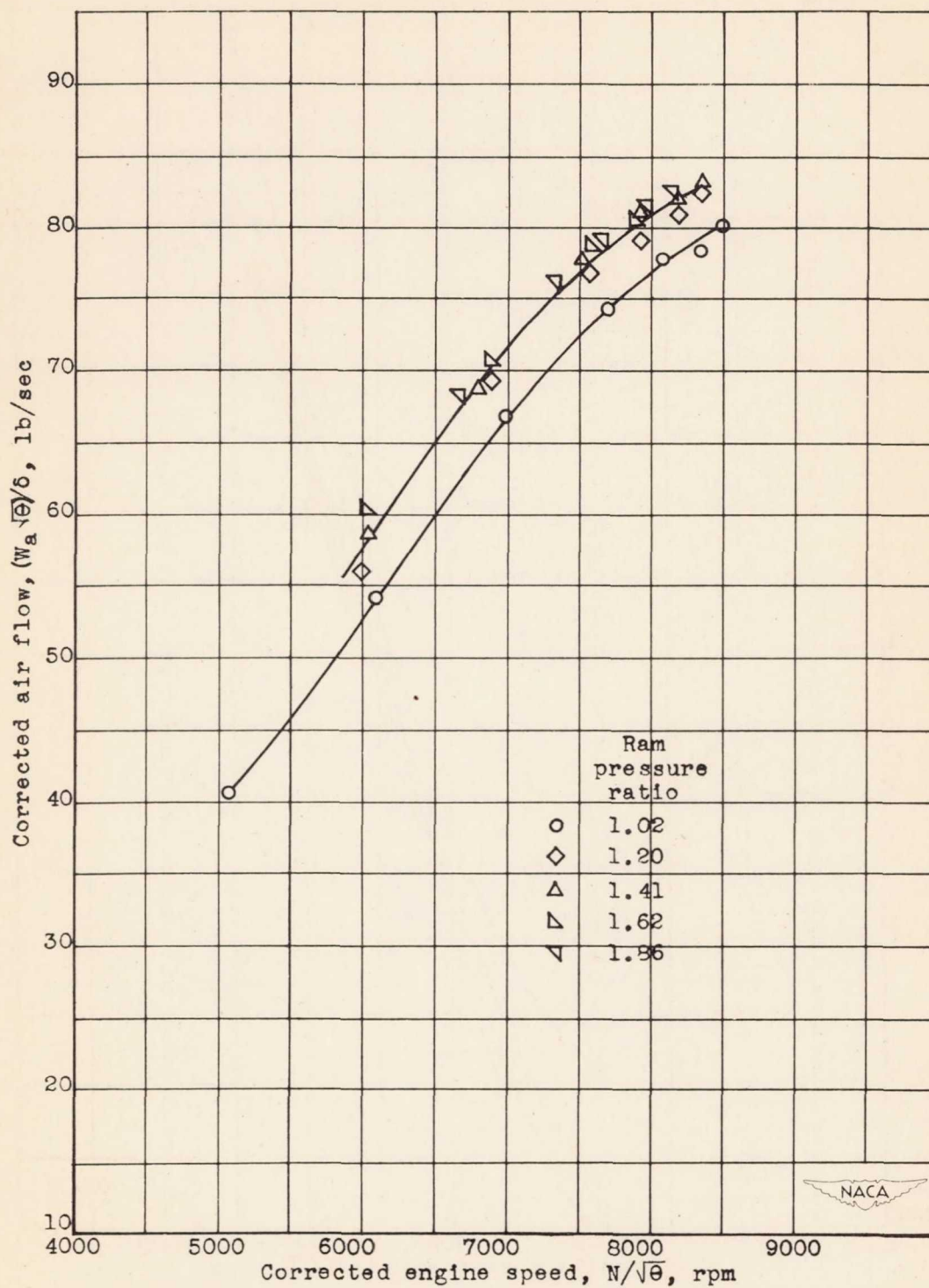
(b) Air flow determined from cowl-inlet survey at station 1. Figure 45.- Concluded.
