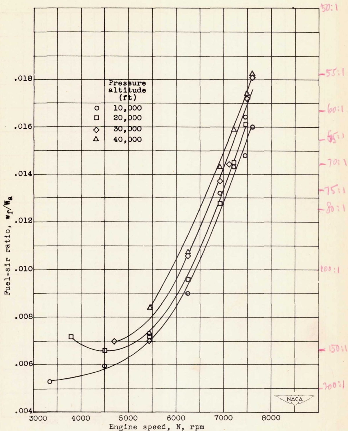
Figure 15.- Effect of engine speed and pressure altitude on fuel-air ratio at a ram pressure ratio of approximately 1.2.
