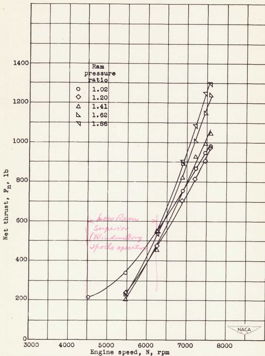
Figure 21.- Effect of engine speed and ram pressure ratio on net thrust at an altitude of 40,000 feet.
