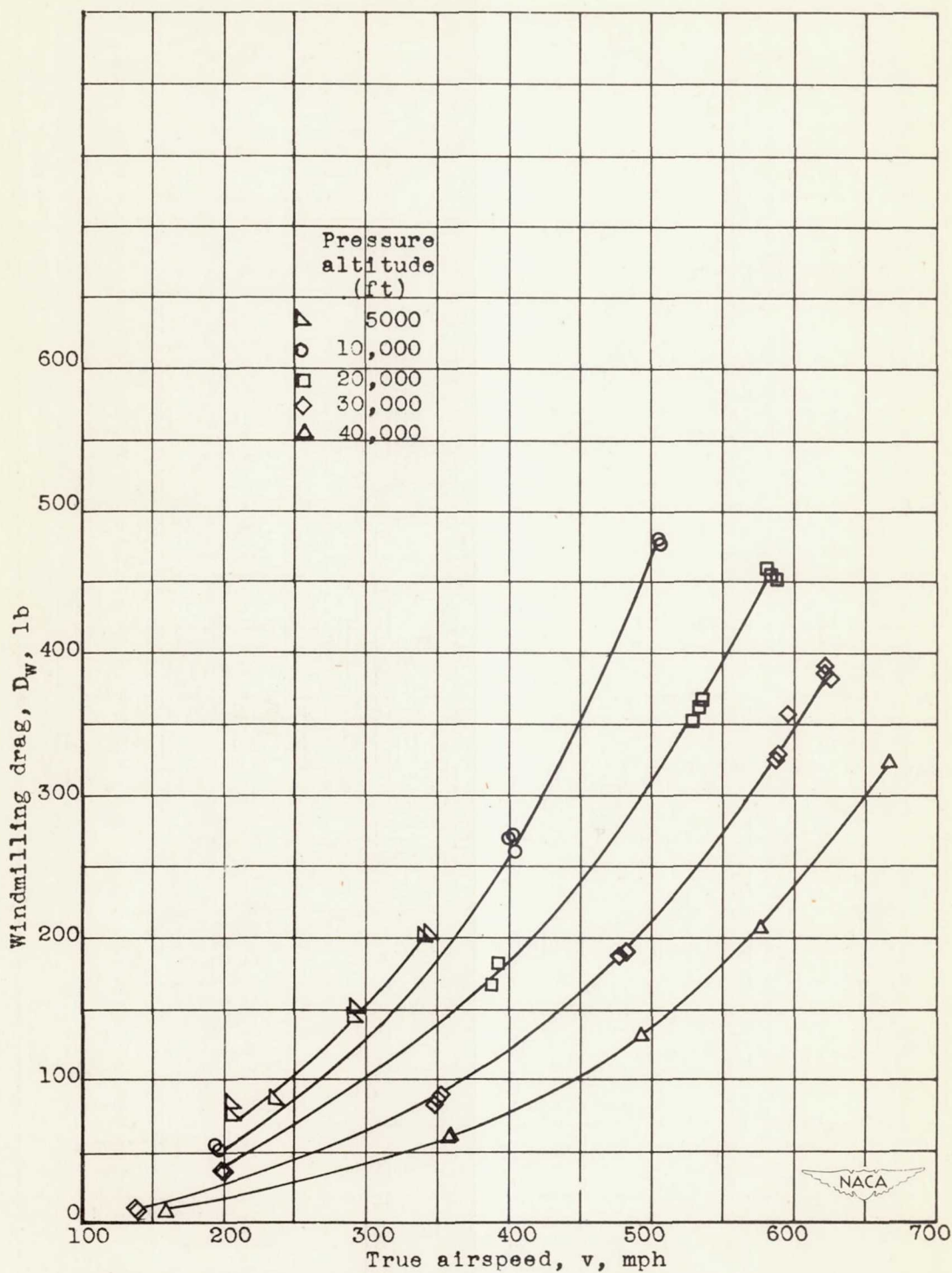
Figure 48.- Effect of altitude and airspeed on windmilling drag.
