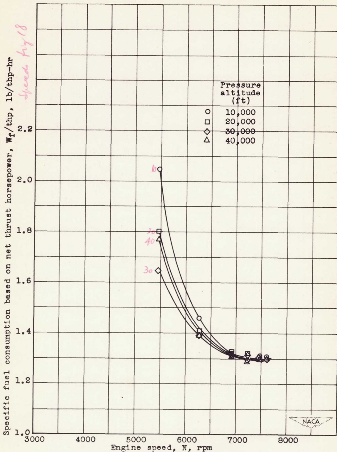
Figure 14.- Variation of specific fuel consumption based on net thrust horsepower with engine speed and pressure altitude at a ram pressure ratio of approximately 1.2.
