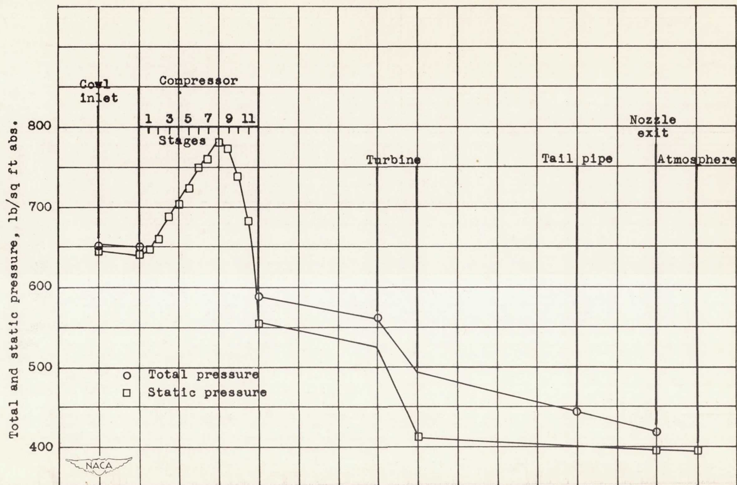
Figure 52. - Total and static pressure survey with engine windmilling. Windmilling speed, 2933 rpm; pressure altitude, 40,000 feet; true airspeed, 575 miles per hour.
