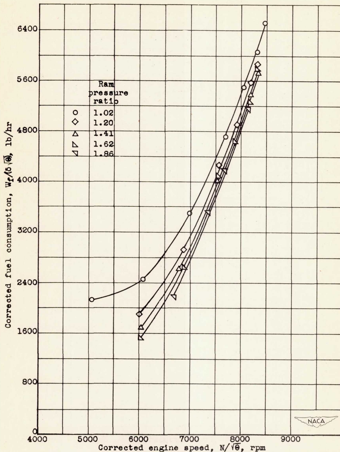
Figure 41. - Effect of corrected engine speed and ram pressure ratio on corrected fuel consumption at a pressure altitude of 40,000 feet. Engine speed and fuel consumption corrected to NACA standard atmospheric conditions at sea level.
