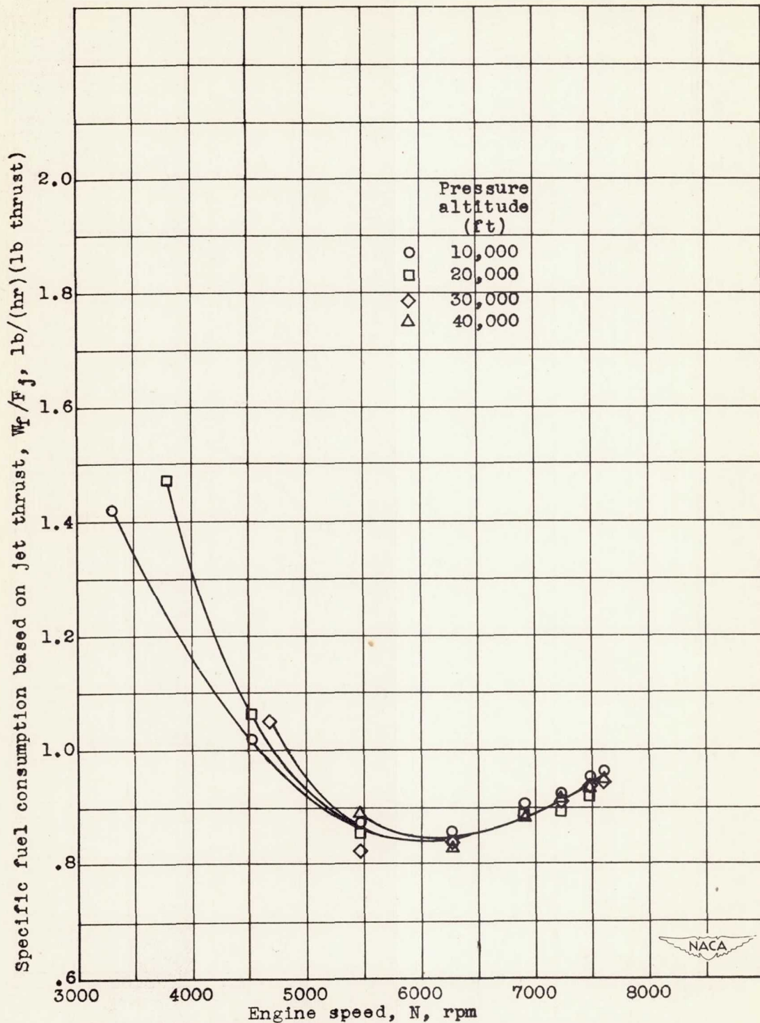
Figure 13.- Variation of specific fuel consumption based on jet thrust with engine speed and pressure altitude at a ram pressure ratio of approximately 1.2.
