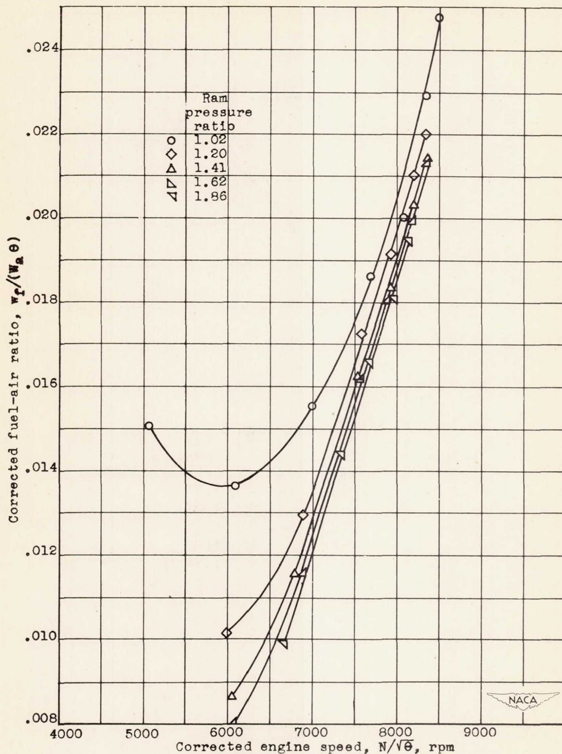
Figure 46. - Effect of corrected engine speed and ram pressure ratio on corrected fuel-air ratio at a pressure altitude of 40,000 feet. Engine speed and fuel-air ratio corrected to NACA standard atmospheric conditions at sea level.
