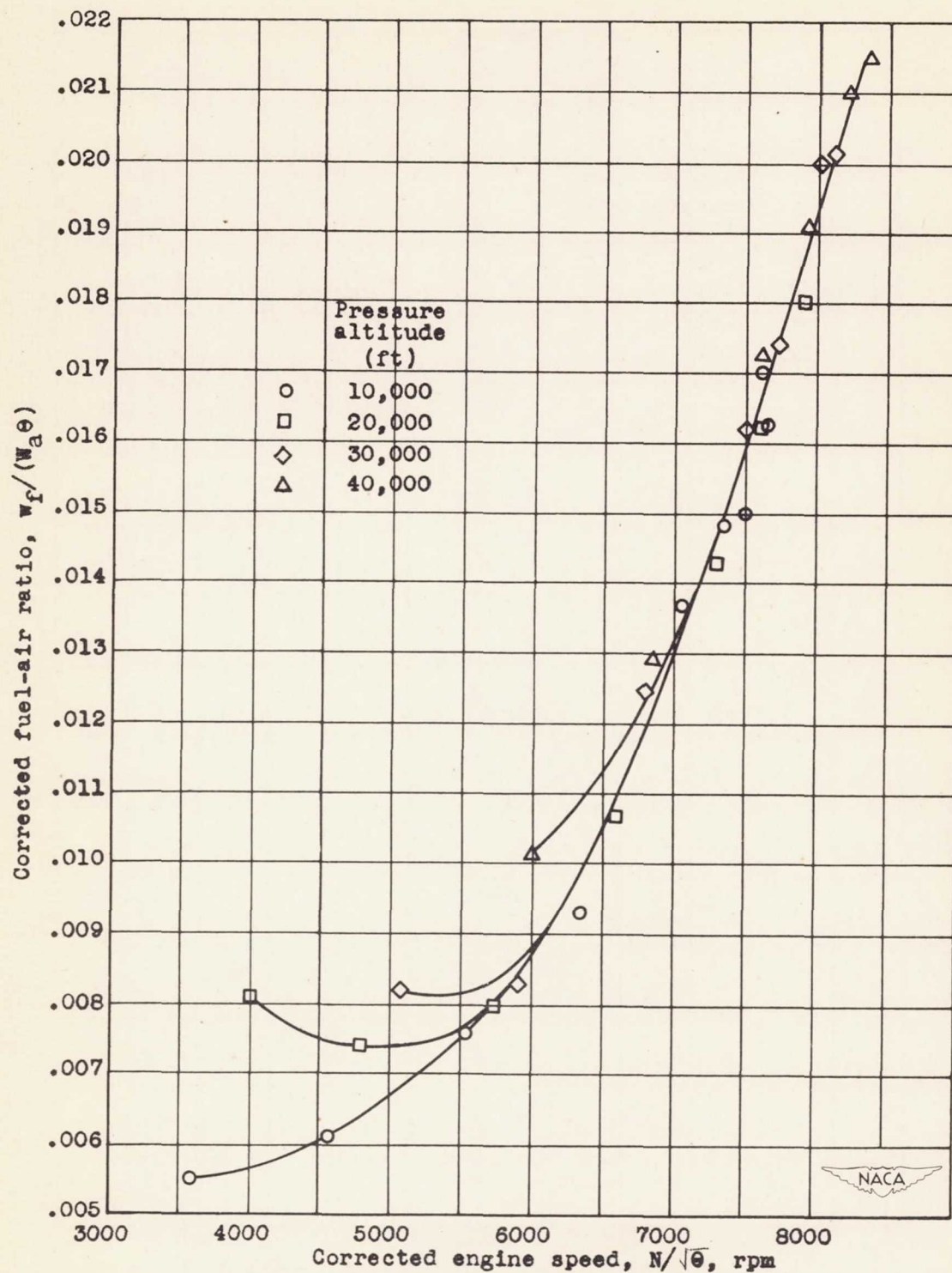
Figure 36. - Effect of corrected engine speed and altitude on corrected fuel-air ratio at a ram pressure ratio of approximately 1.2. Engine speed and fuel-air ratio corrected to NACA standard atmospheric conditions at sea level.
