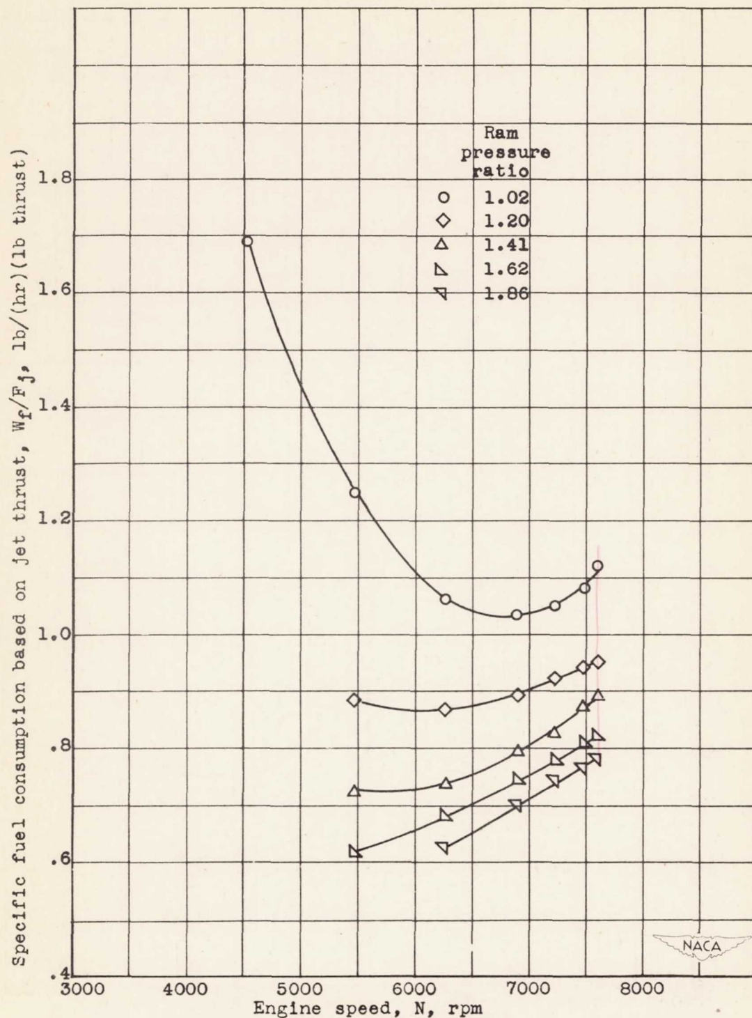
Figure 23.- Effect of engine speed and ram pressure ratio on specific fuel consumption based on jet thrust at a pressure altitude of 40,000 feet.
