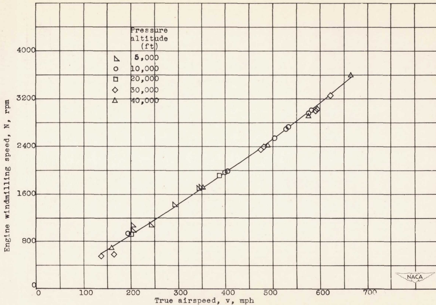
Figure 47.- Variation of engine windmilling speed with true airspeed and pressure altitude.
