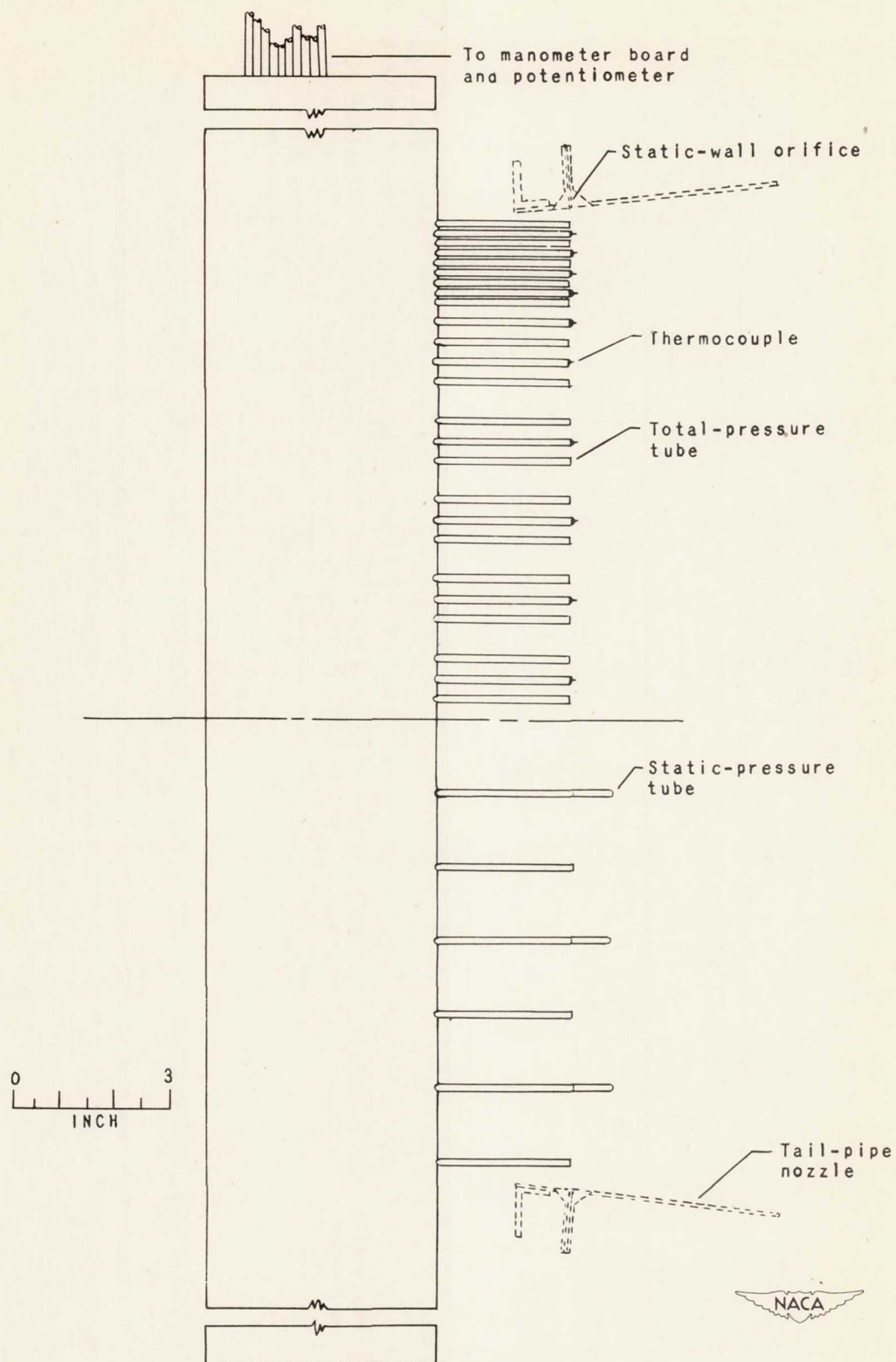
Figure 5. - Details of total- and static-pressure-tube and thermocouple installation at nozzle outlet.
