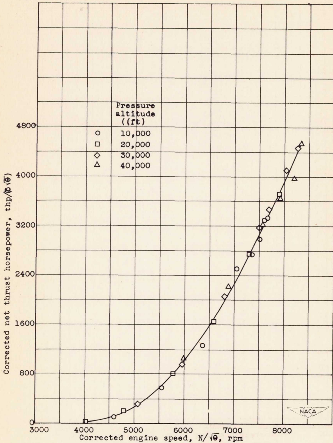
Figure 31. - Effect of corrected engine speed and pressure altitude on corrected net thrust horsepower at a ram pressure ratio of approximately 1.2. Engine speed and net thrust horsepower corrected to NACA standard atmospheric conditions at sea level.
