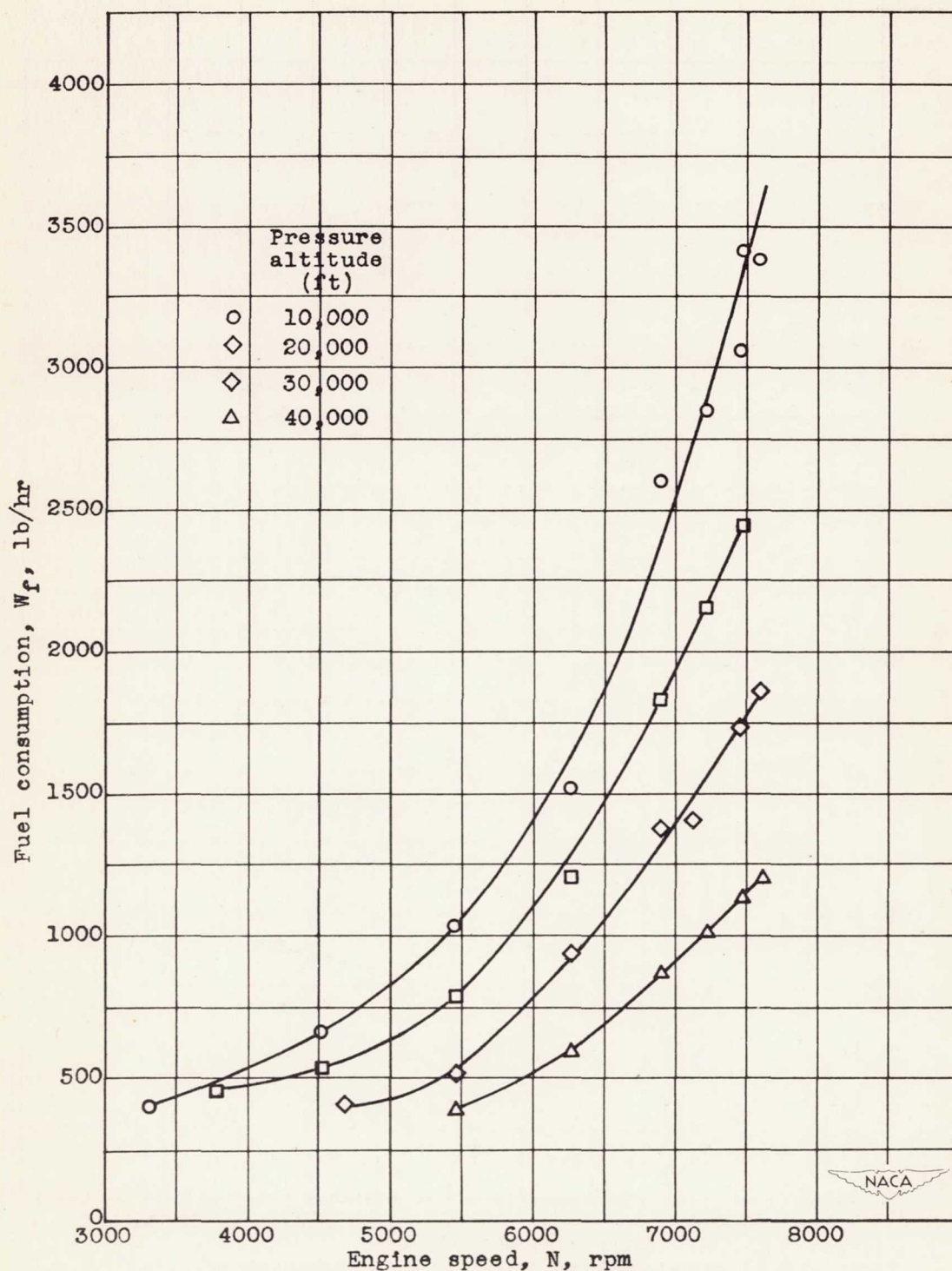
Figure 11.- Effect of engine speed and altitude on fuel consumption at a ram pressure ratio of approximately 1.2.
