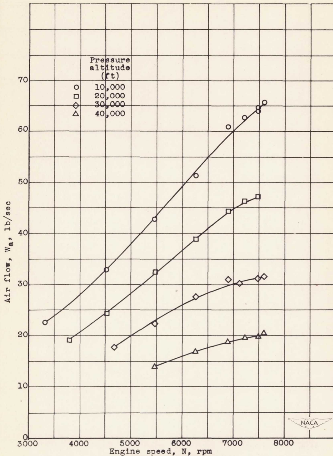
(b) Air flow determined from cowl-inlet survey at station 1. Figure 12.- Concluded.
