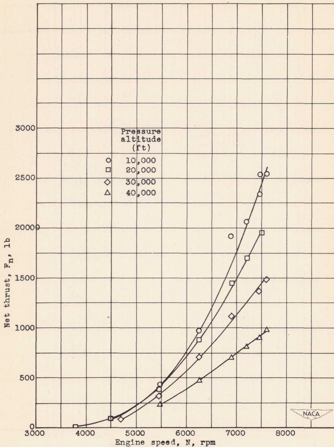
Figure 9.- Effect of engine speed and altitude on net thrust at a ram pressure ratio of approximately 1.2.
