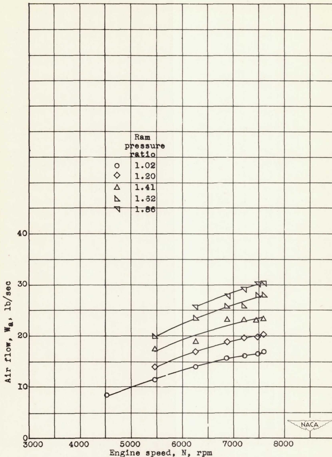
(b) Air flow determined from cowl-inlet survey at station 1. Figure 20.- Concluded.
