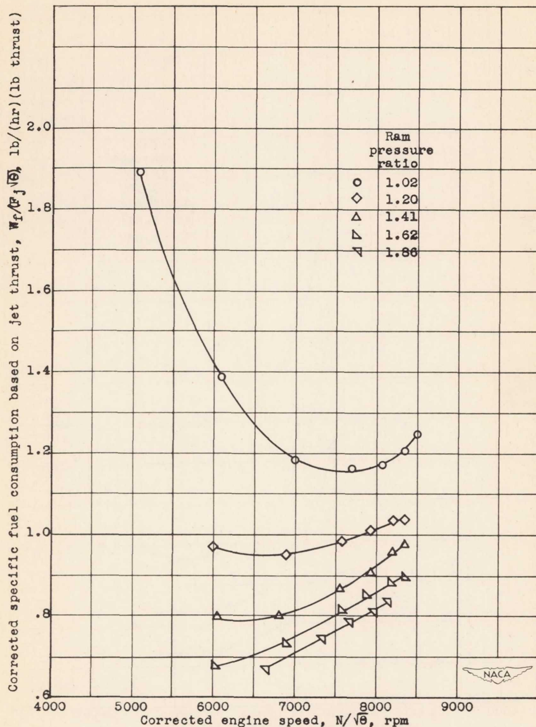
Figure 42. - Effect of corrected engine speed and ram pressure ratio on corrected specific fuel consumption based on jet thrust at a pressure altitude of 40,000 feet. Engine speed and specific fuel consumption corrected to NACA standard atmospheric conditions at sea level.
