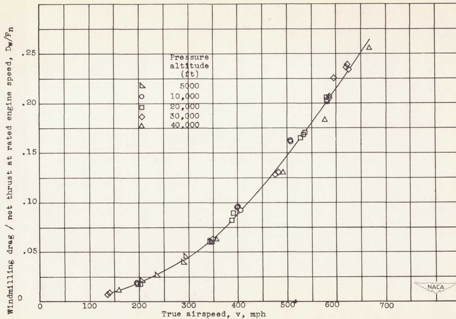
Figure 49.- Effect of altitude and true airspeed on the ratio of windmilling drag to net thrust at rated engine speed.
