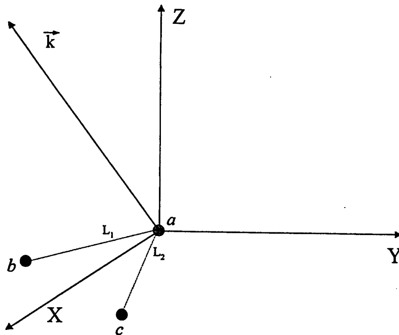
Figure 2. Coherent laser light is transmitted simultaneously from spacecraft a to spacecraft b and c , and coherently transponded back to a . The X axis is along the bisector of the angle enclosed between the two arms of the interferometer. The Y axis is orthogonal to the X axis in the plane of the interferometer, and the Z axis is chosen in such a way to form together with (X, Y) a right-handed set of axes. The gravitational wave train propagates along the \vec{k} direction.
