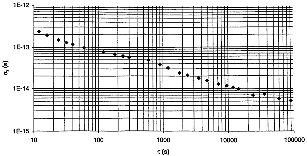
FIGURE 3: frequency stability of CH1-76 passive hydrogen maser (serial no. 84065) expressed in terms of the root Allan variance ( \sigma_y )
