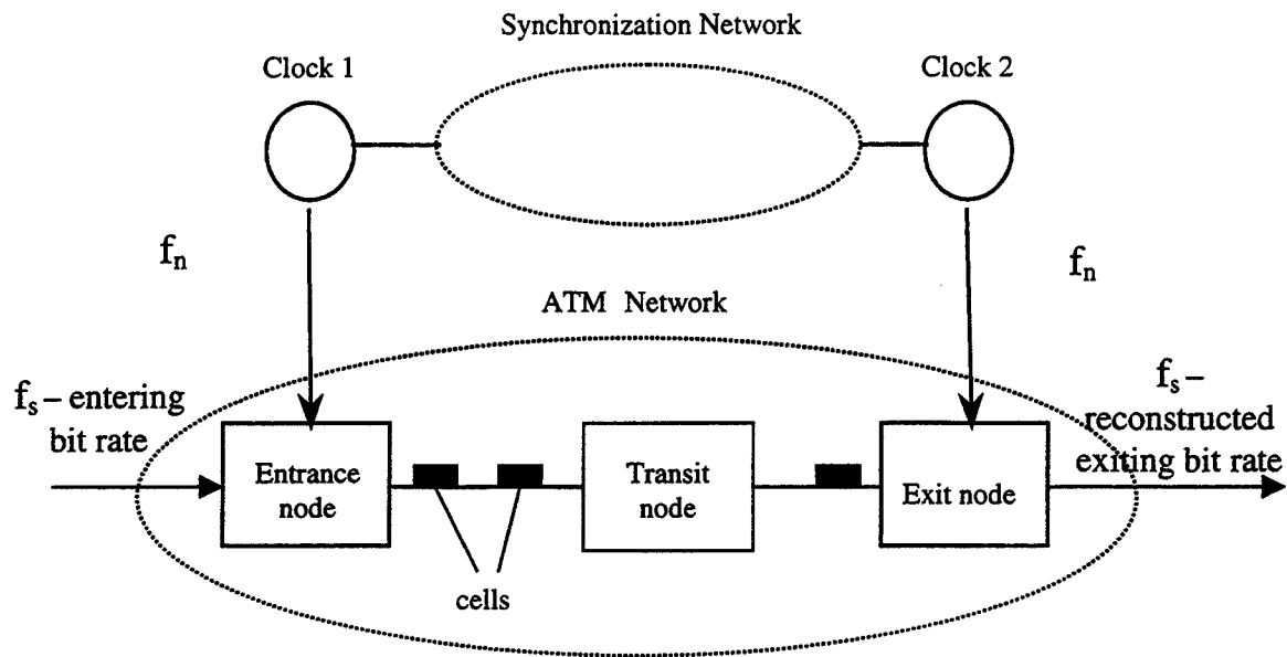
Figure 1. SRTS method for transporting CBR traffic over an ATM network.
