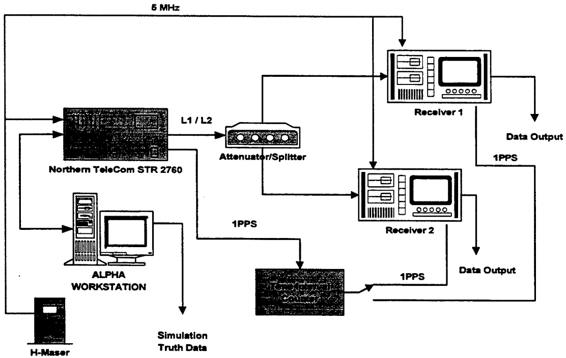
Figure 1. Simulation Configuration
