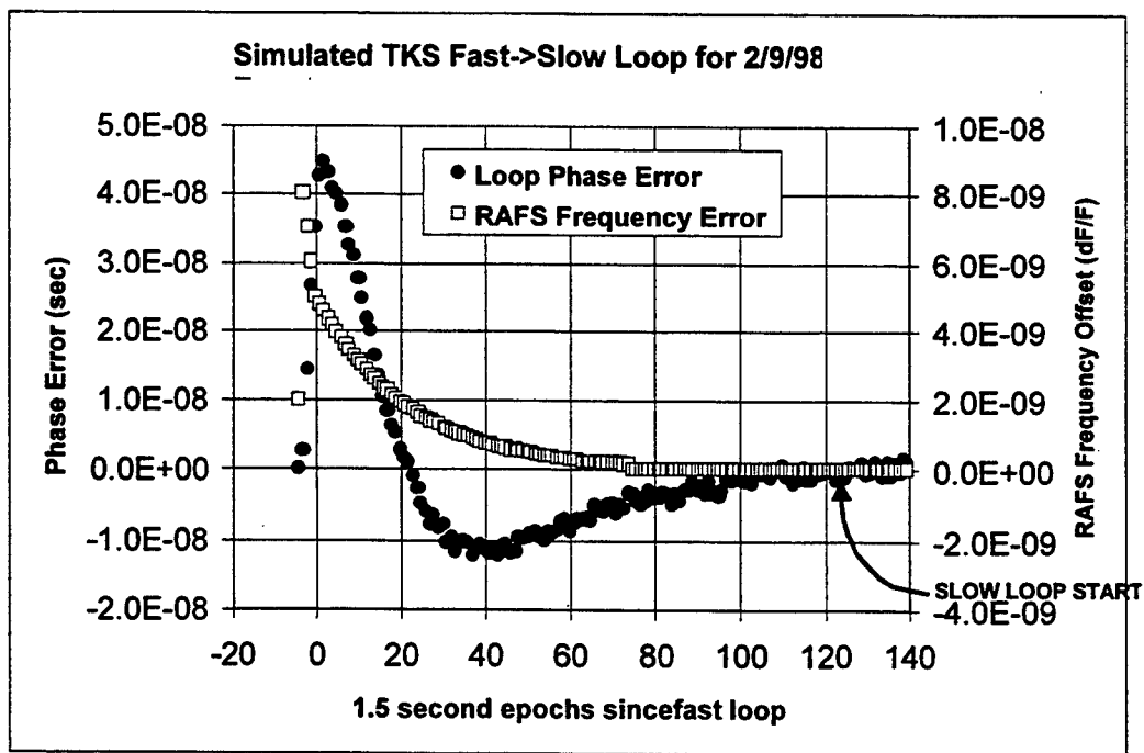
Figure 5. Feb. 9 Event Simulated Transient Profile
