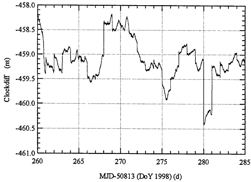
Figure 3: Delay between USNB and USNO as measured by GeTT. Discontinuities discussed in the text are clearly visible
