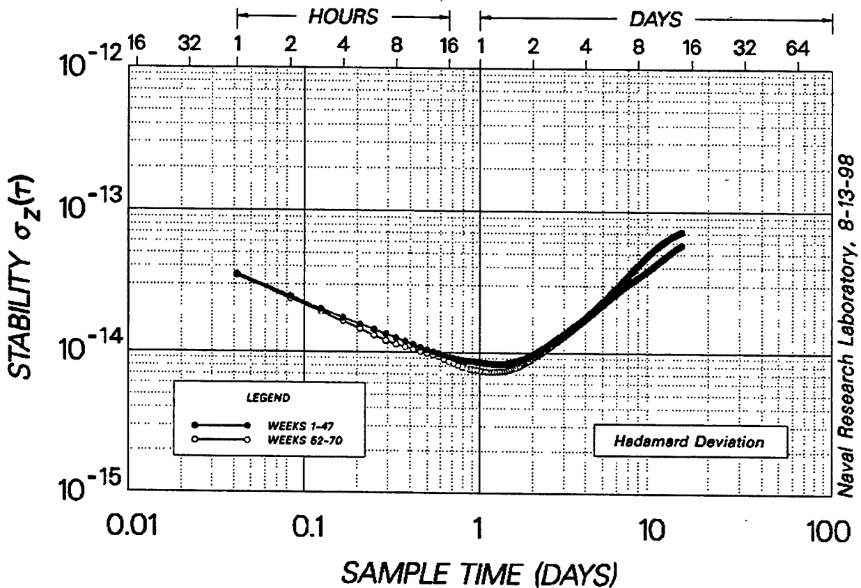
Fig. 12. RAFS No. 30 Frequency Stability 31 March 1997 to 11 August 1998
