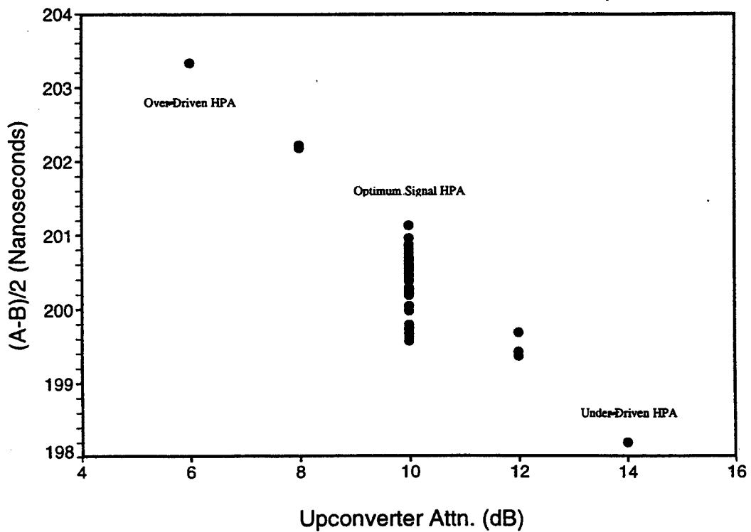
X-Band (FX2) Baseline TWSTT Experiment Mean Behaviour w/Signal Varied into HPA
