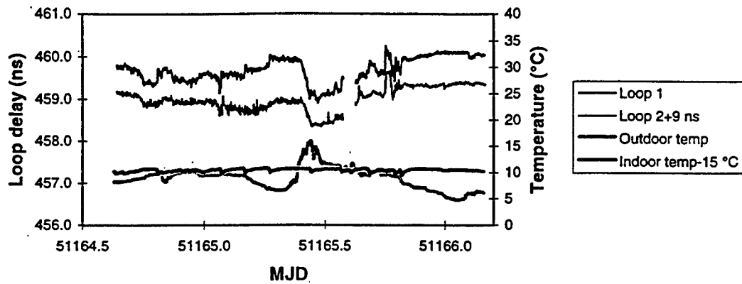
Figure 4. Measurements for two downlink characterization loops taken using the Satre modem. Indoor and outdoor temperature data are also shown.
