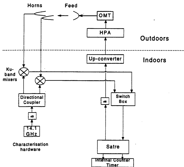
Figure 2. Uplink characterization test configuration.
