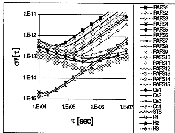
Fig. 2: Allan Deviation (ADEV) of the STS together with that of the 22 simulated clocks in Case 1
