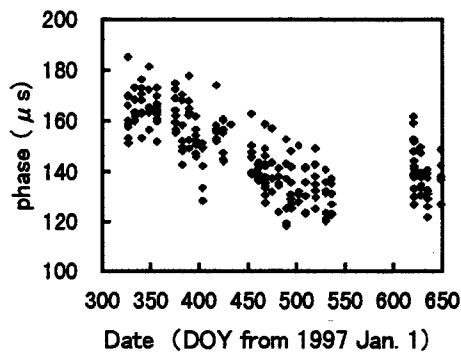
Figure 6. Timing residuals of PSR1937+21. (Nov. 21, 1997~Oct. 9, 1998) Predicted phases are calculated by Tempo program ver. 10.010. Each observed phase is obtained from the observations with 50MHzBW in the 2GHz and 27 minutes integration.
