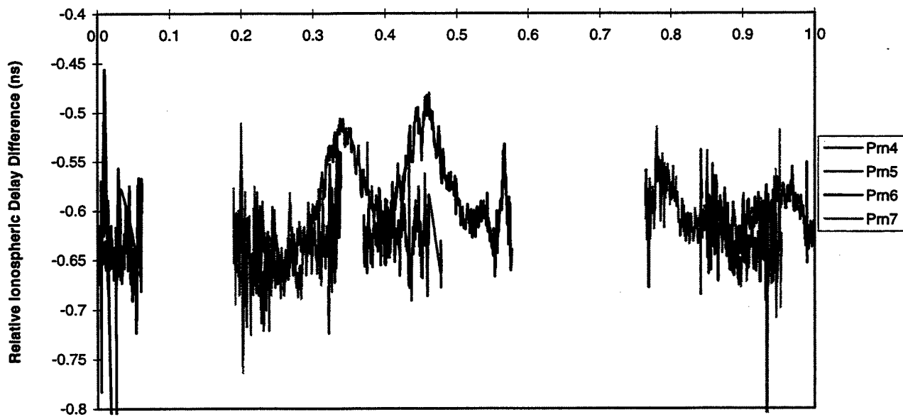
Figure 10: Phase ionospheric delay measurements, individual satellite tracks, (AOA TTR-4P - Ashtech Z12-T) phase differences.
