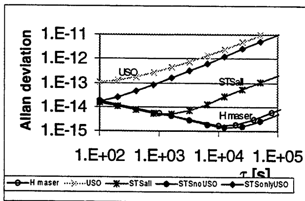
Fig. 5: Instability of the STS in Case 2 obtained with different ensembles of clocks & typical ADEV pattern of USO and H-maser
