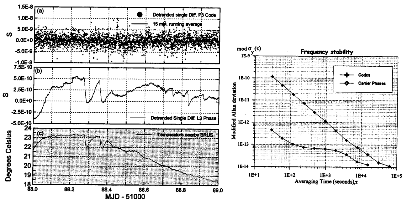
Figure 7: Time differences (H-maser BRUSSEL - H-Maser WETZELL) and frequency stability analysis for a medium-length (640 km) baseline experiment.
