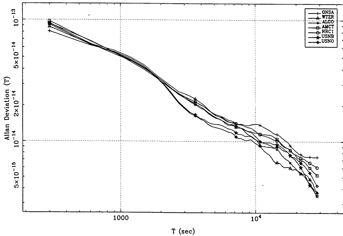
Figure 5: Allan deviations for a set of clocks in the mentioned subnet. The maser at PTB was (arbitrarily) chosen as a reference.
