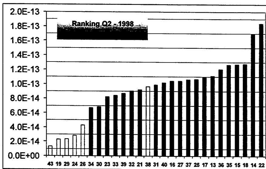
Figure 1. Ranking by 1-Day Hadamard Deviation
