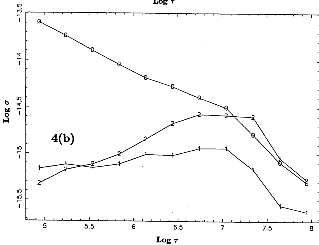
Figure 4. Frequency stabilities for timescales derived using temporal Nth-order data differences and cesium-dominated weight scheme "2." (a) is for cesium-only timescales using data since MJD 49400. (b) is for maser-only timescales derived using data since MJD 50079. Plot characters correspond to order of pre-fit differencing.
