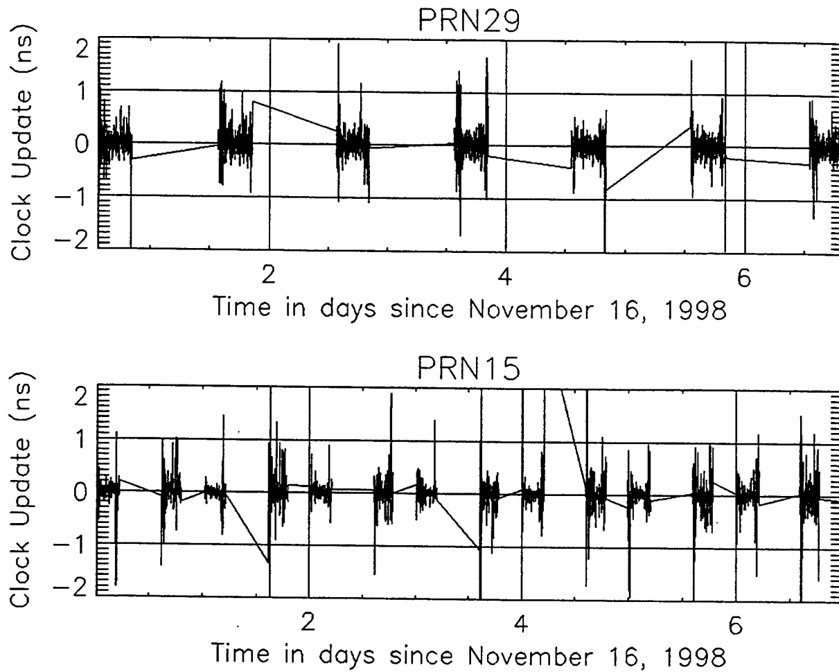
Figure 3: Real-time updates to short-term GPS satellite clock models for a satellite with SA (PRN29) and a satellite without SA (PRN15).
