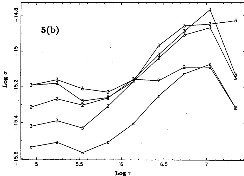
Figure 5. Frequency stabilities for mean timescales generated using only one type of clock and three independent subsets, derived from a 3-cornered-hat analysis of timescales that allowed for covariances. (a) is for an HP5071-only timescale and is based upon data since MJD 49400. (b) is for a Sigma Tau/Datum maser-only timescale and is based on data since MJD 50079. The curve indicated by "2" is for a mean timescale of one-half of the clocks relative to a mean timescale of the other half, and the curve indicated by "c" is for the complete USNO HP5071 ensemble (in both, covariances were neglected).
