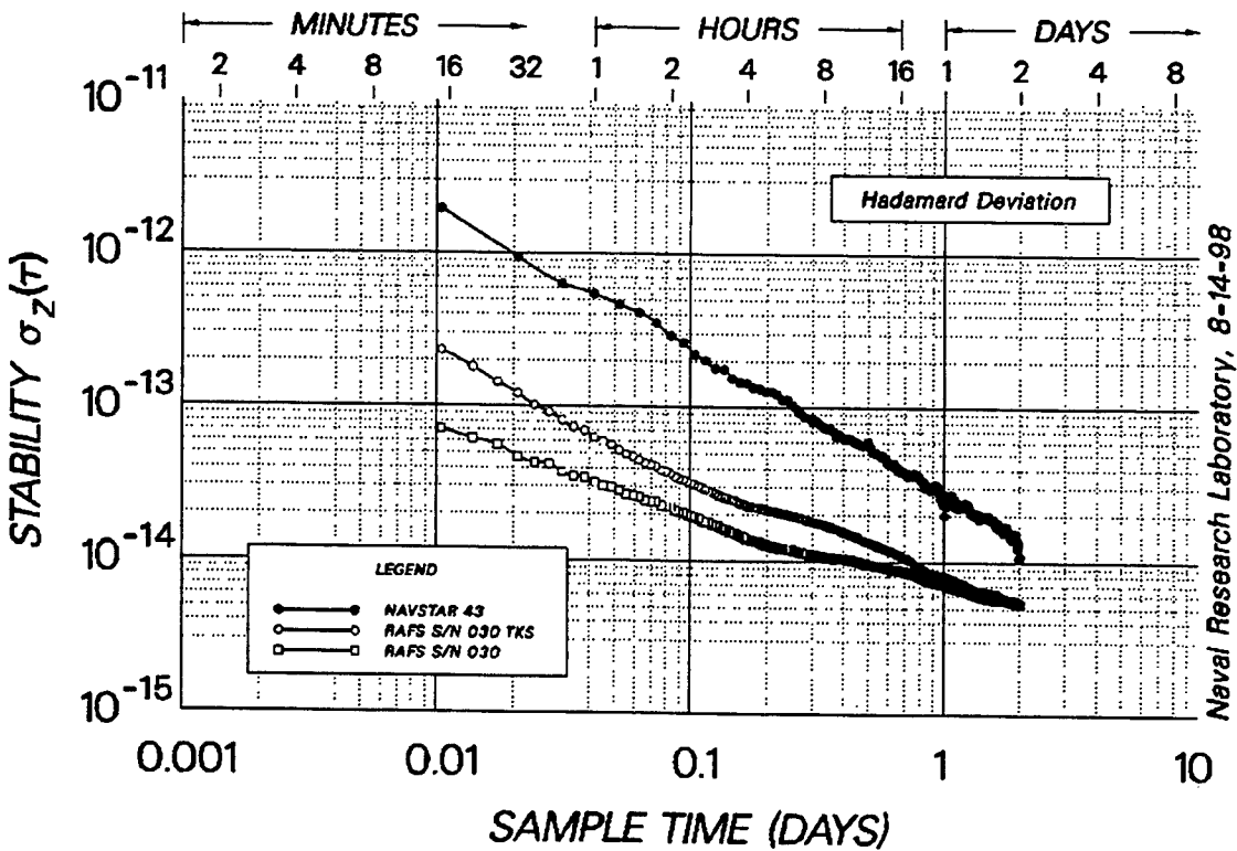
Fig. 16. Frequency Stability Comparison 10 July 1998 to 5 August 1998
