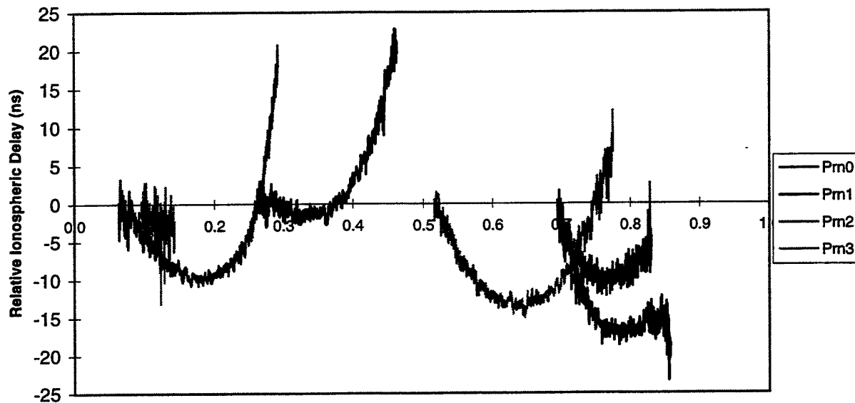
Figure 9: L1 single frequency ionospheric delay measurements, individual satellite tracks. Ashtech Z12-T receiver.
