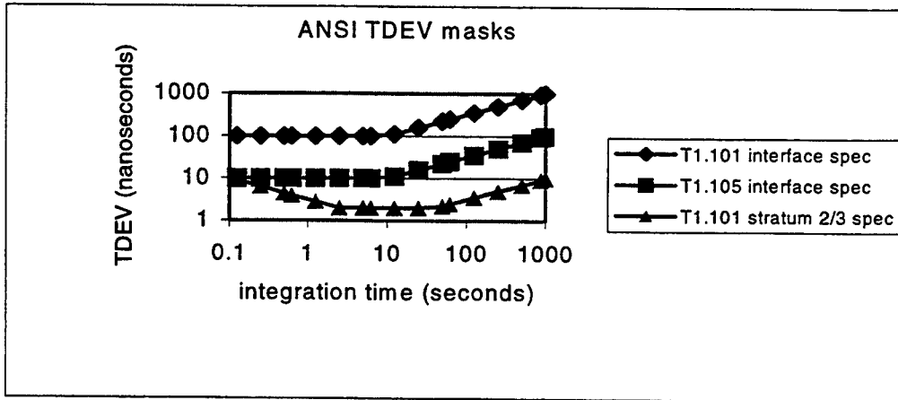
Figure 3. ANSI TDEV masks used to simulate clock noise.
