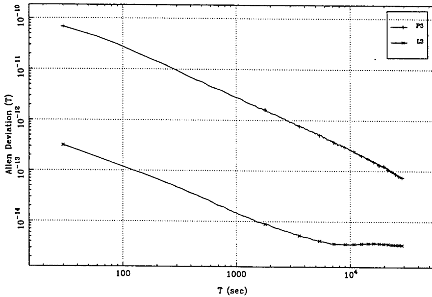
Figure 2: Allan deviation for the data given in Figure (1) using 24 hrs of data. Both Figures (1) and (2) reflect the difference in the intrinsic precision of the two observables.
