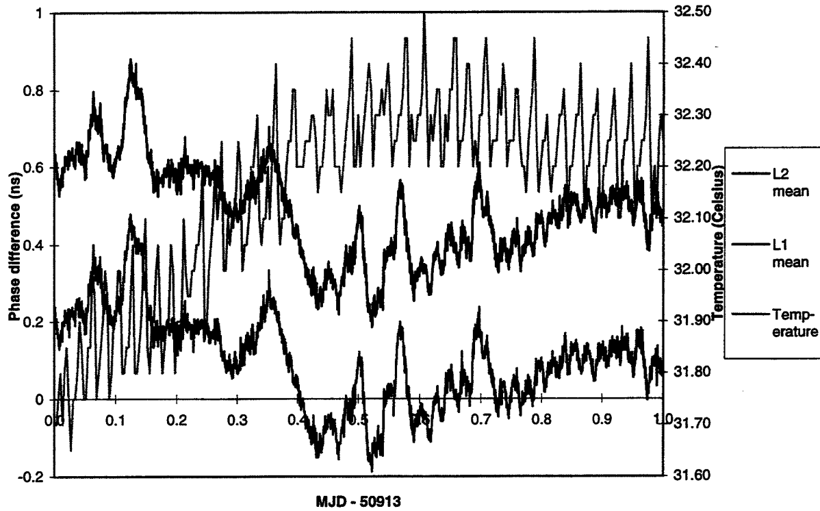
Figure 5: L1 and L2 phase comparisons (AOA TTR-4P - Ashtech Z12-T), mean values.
