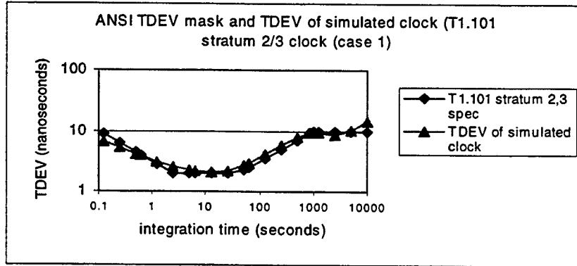
Figure 7. TDEV mask used to simulate the clock noise and TDEV of simulated clock (T1.101 stratum 2 or stratum 3 clock ).
