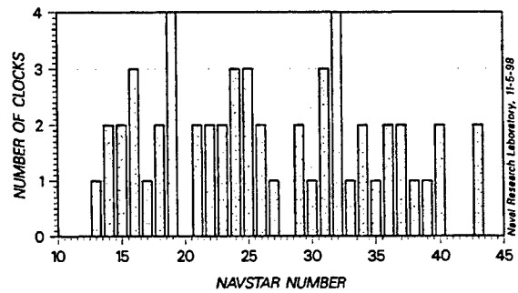
Figure 4. Number of Clocks Operated Since Insertion 30 September 1998
