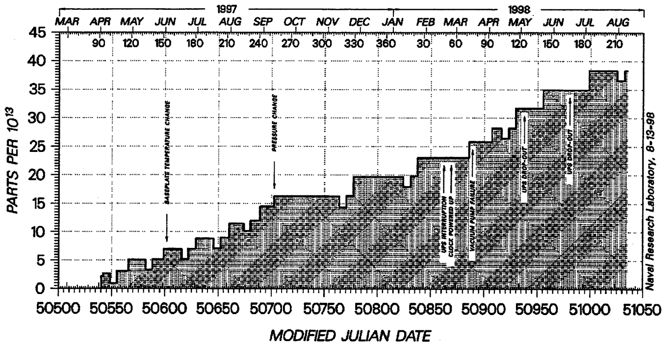
Fig. 9. RA FS No. 28 Cumulative Frequency Corrections Weeks 1 - 70
