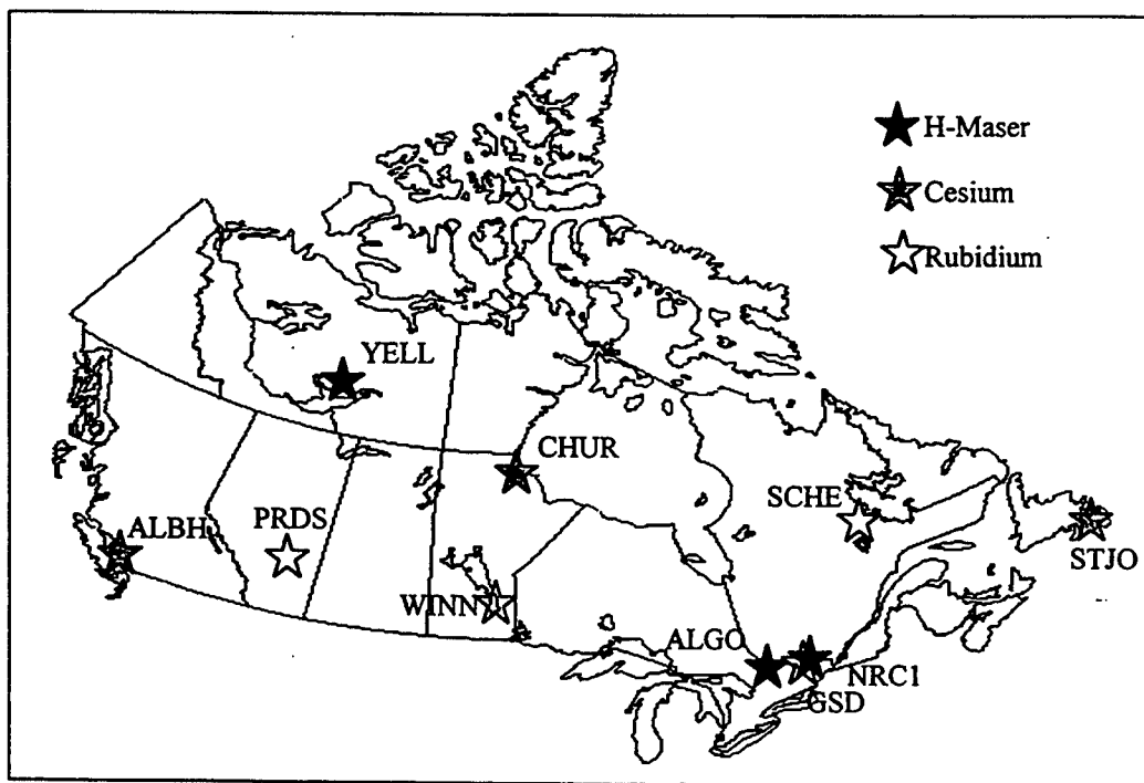
Figure 1: Real-Time Canadian Active Control System network.
