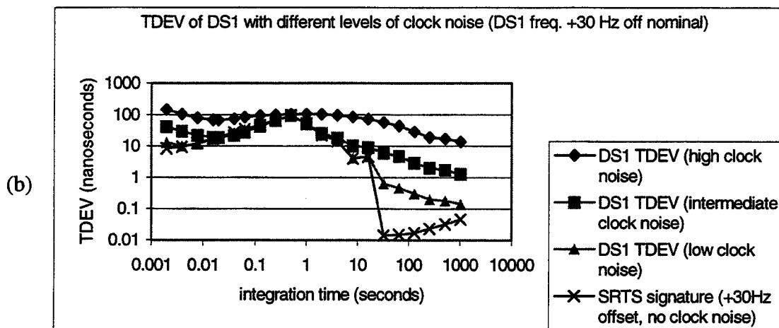
Figure 6. TDEV of DS1 phase resulting from different levels of clock noise (a) Entering DS1 has nominal frequency (b) Entering DS1 has +30 Hz offset from nominal frequency.
