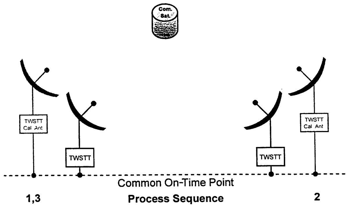
Fig. 8 TWSTT Link Calibrated by Co-Located TWSTT Method
