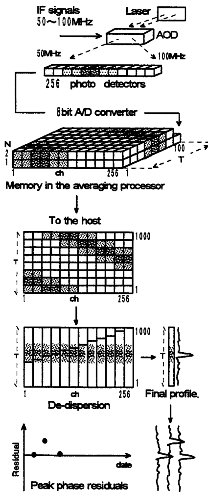
Figure 4. Data flow.
