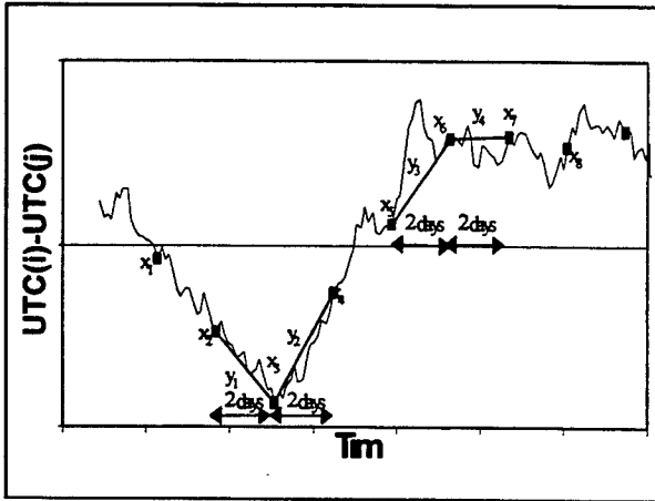
Figure 1. Estimation of ADEV(2 Days). Measures are executed on Monday, Wednesday and Friday. For any \Delta 2x estimation, the three consecutive measures are considered for each week.
