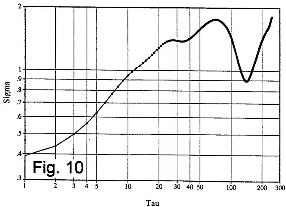
Time Deviation (TDEV) of White FM For All Tau from Stable Software
