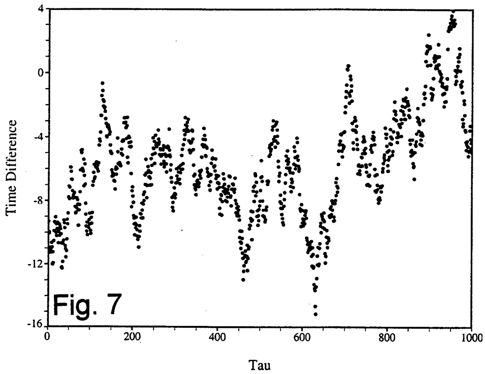
Time-Domain White FM
