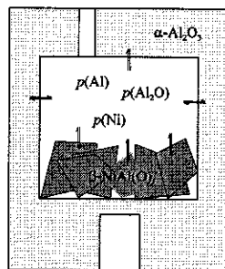
Figure 3. Schematic of an \text{Al}_2\text{O}_3 effusion-cell containing a \beta -NiAl(O) f sample.
