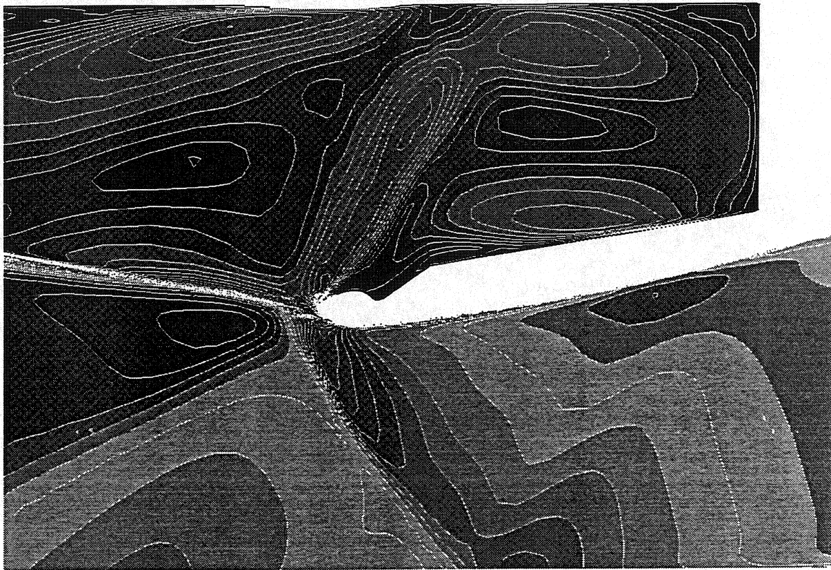
Figure 12 – 3D Mach Contour Close-Up Aft Lip.
