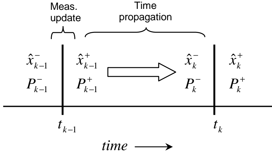
Fig. 2–1: Kalman Filter Process
