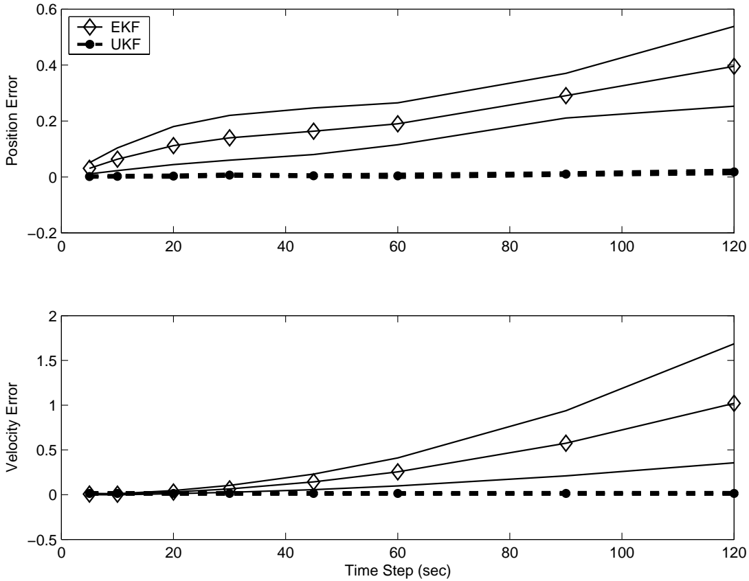
Fig. 4–8: FreeFlyer™, baseline 100 km
