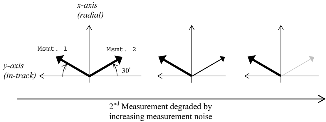
Fig. 3–2: LPM Example #1 – Filter performance as second measurement is degraded.
