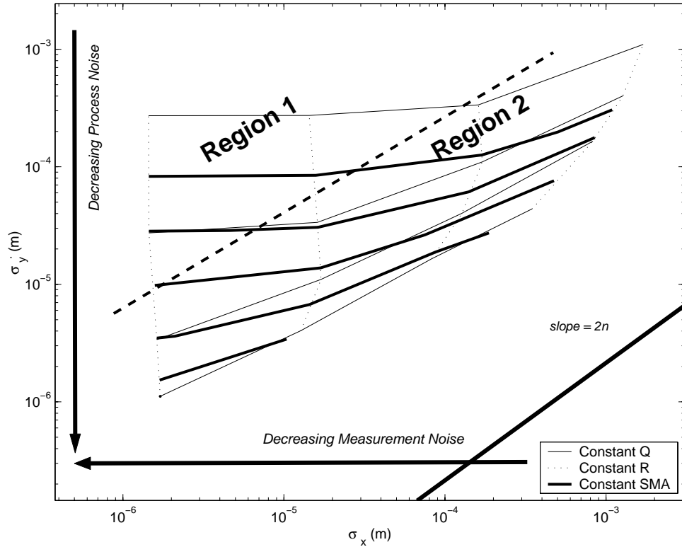
Fig. 3–14: Contours of constant Q , R and semimajor axis are shown for NPM results. Nonlinear effects were minimized for this simulation, which was run with a 0.1 second time step.
