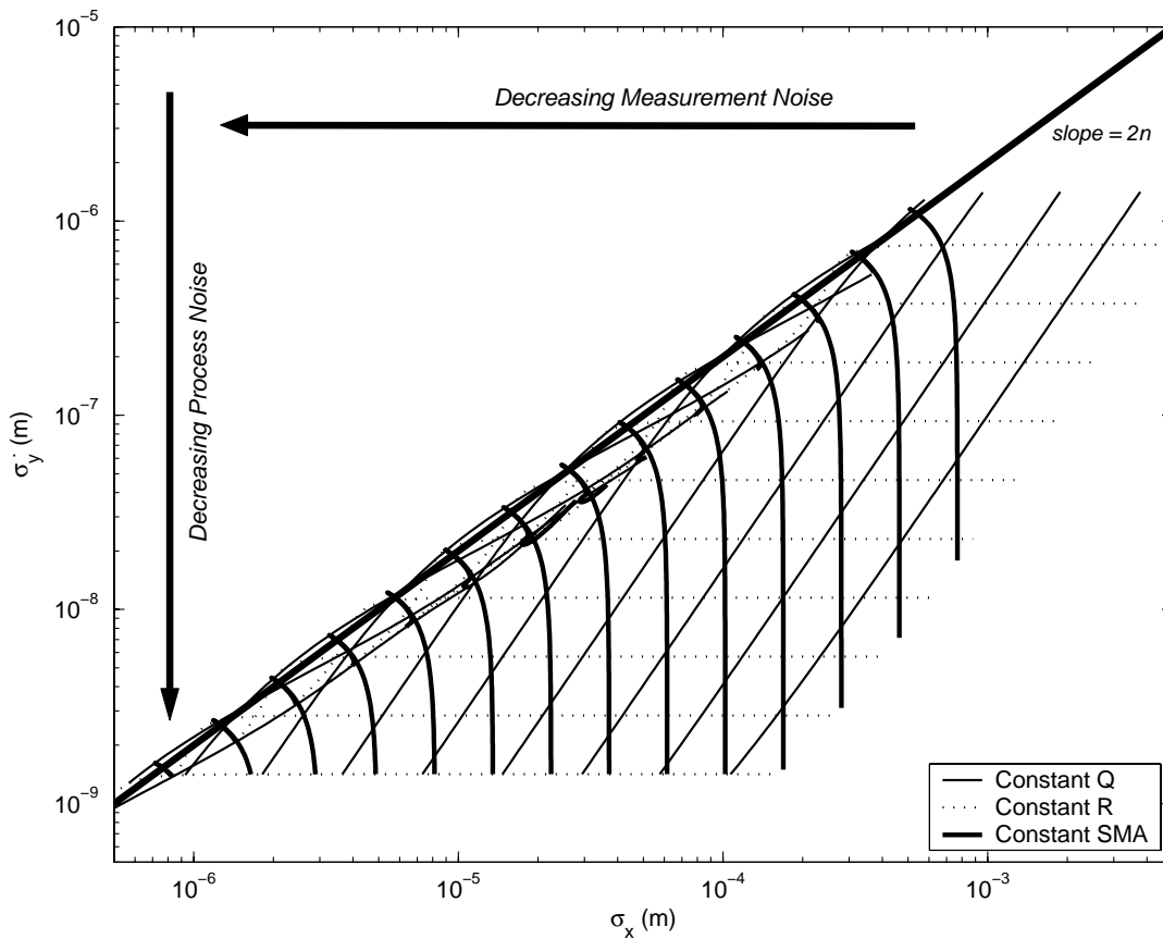
Fig. 3–12: Contours of constant Q , R , and semimajor axis are shown on axes of position and velocity error. Here, the LPM has been given extremely good velocity measurements, and the position measurements have been severely degraded. This was done to show what is required to occupy the space under the diagonal balance line
