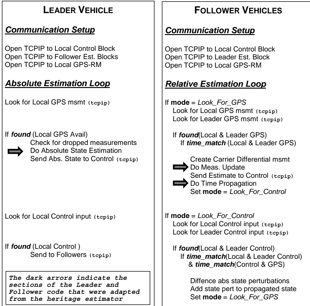
Fig. 5–4: Pseudocode for the Leader and Follower blocks of the Navigation Executive
