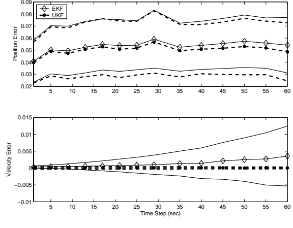
Fig. 4-7: GSFC, baseline 10 km
