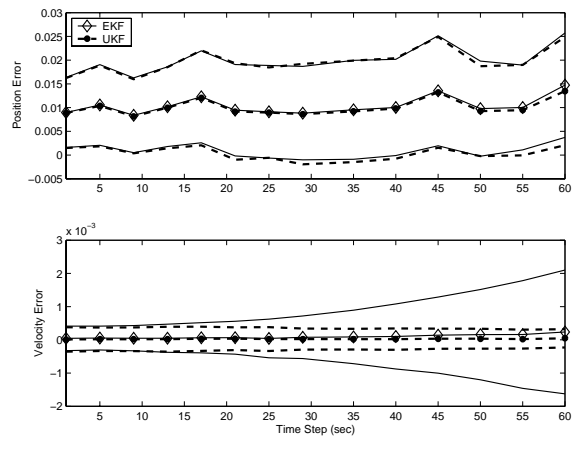
Fig. 4-6: GSFC, baseline 1 km
