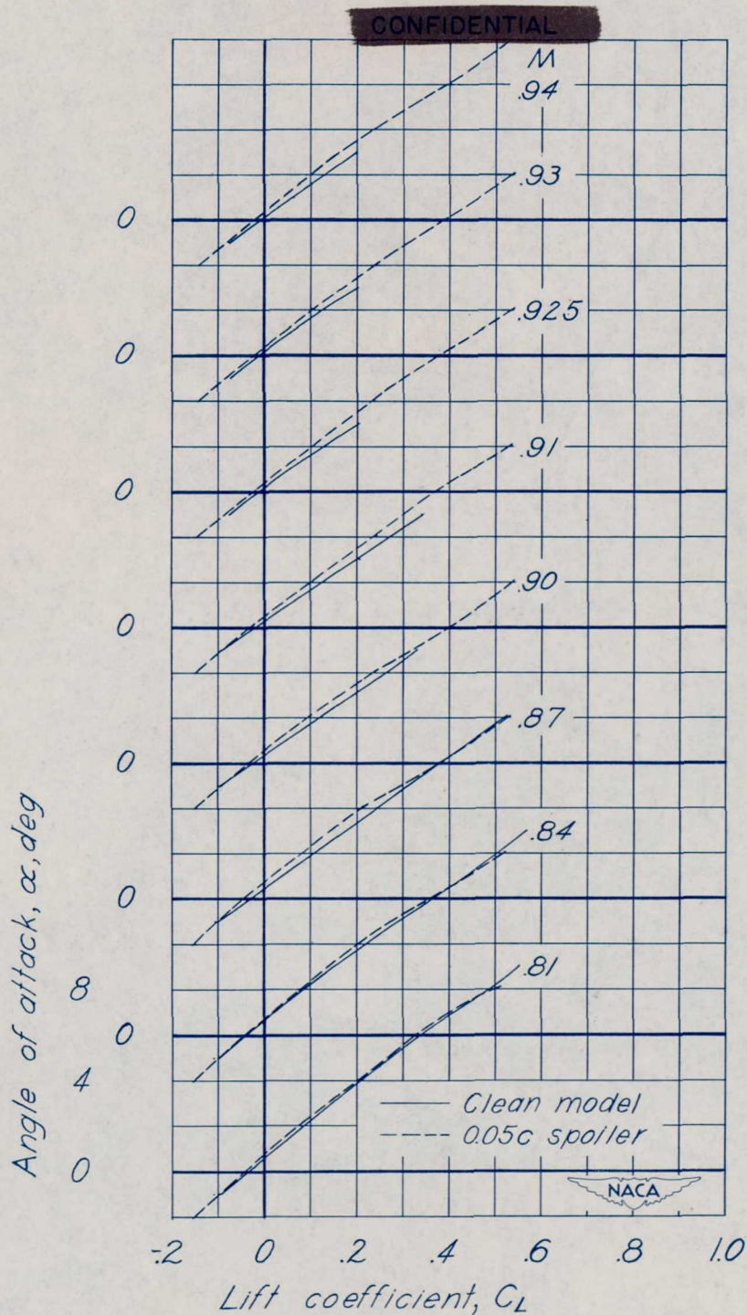
Figure 10.— Effect of spoiler on aerodynamic characteristics for various Mach numbers of the 0.08-scale semispan model of the XF7U-1 airplane. Fins on; \delta_a = 0^\circ .
