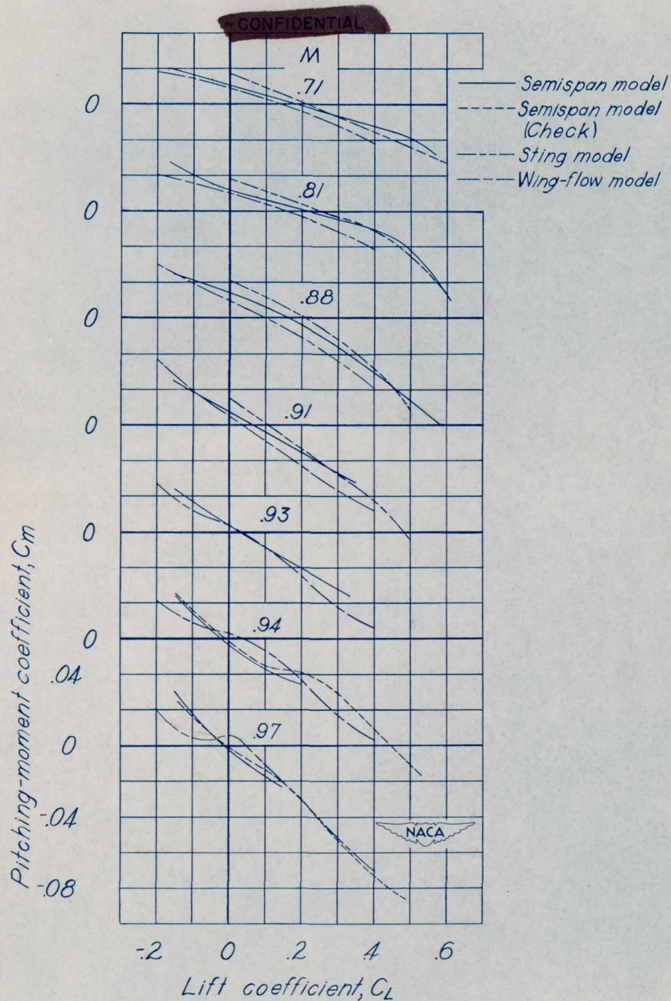
Figure 20.— A comparison of pitching-moment coefficients obtained by three different test methods on models of the XF7U-1 airplane. Vertical fins on; \delta_a = 0^\circ .
