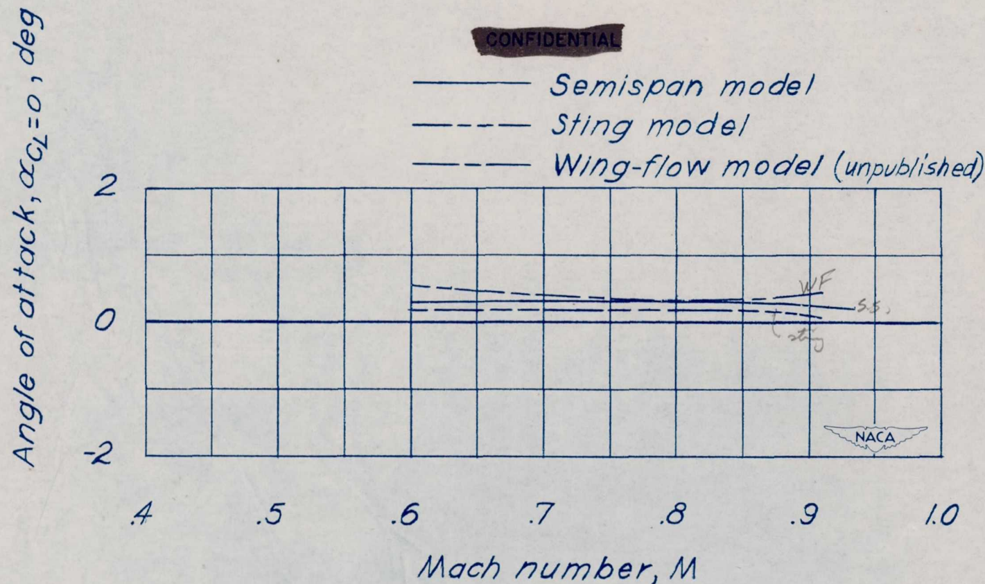
Figure 14.— A comparison of angle of attack at zero lift coefficient through the Mach number range as obtained by three different test methods on models of the XF7U-1 airplane. Vertical fins off, \delta_a = 0^\circ .
