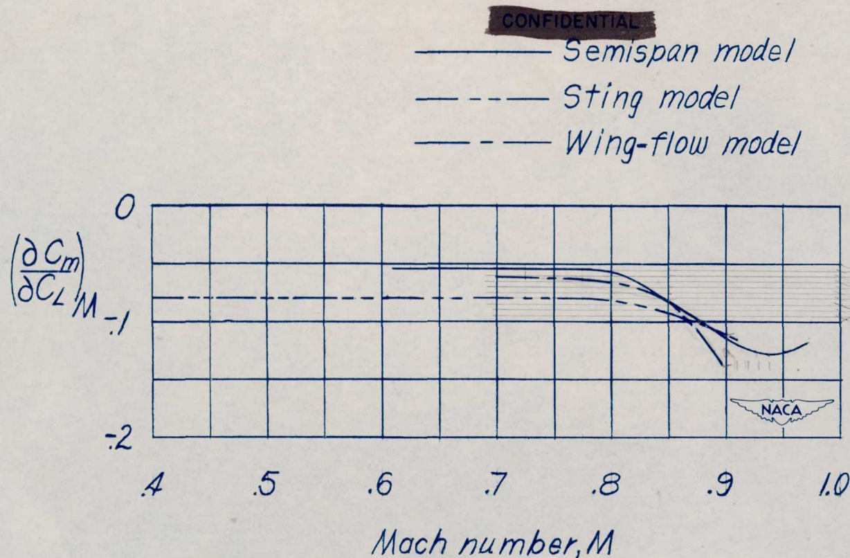
Figure 18.— A comparison of \left(\frac{\partial C_m}{\partial C_L}\right)_M variation with Mach number for the low-lift-coefficient range as obtained by three different test methods on models of the XF7U-1 airplane. Vertical fins off; \delta_a = 0^\circ . CONFIDENTIAL
