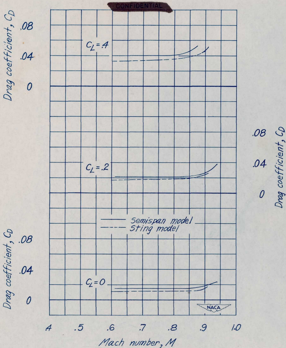
Figure 15.— A comparison of drag coefficient through the Mach number range as measured by the semispan and sting test methods on models of the XF7U-1 airplane. Vertical fins on, \delta_a = 0^\circ .
