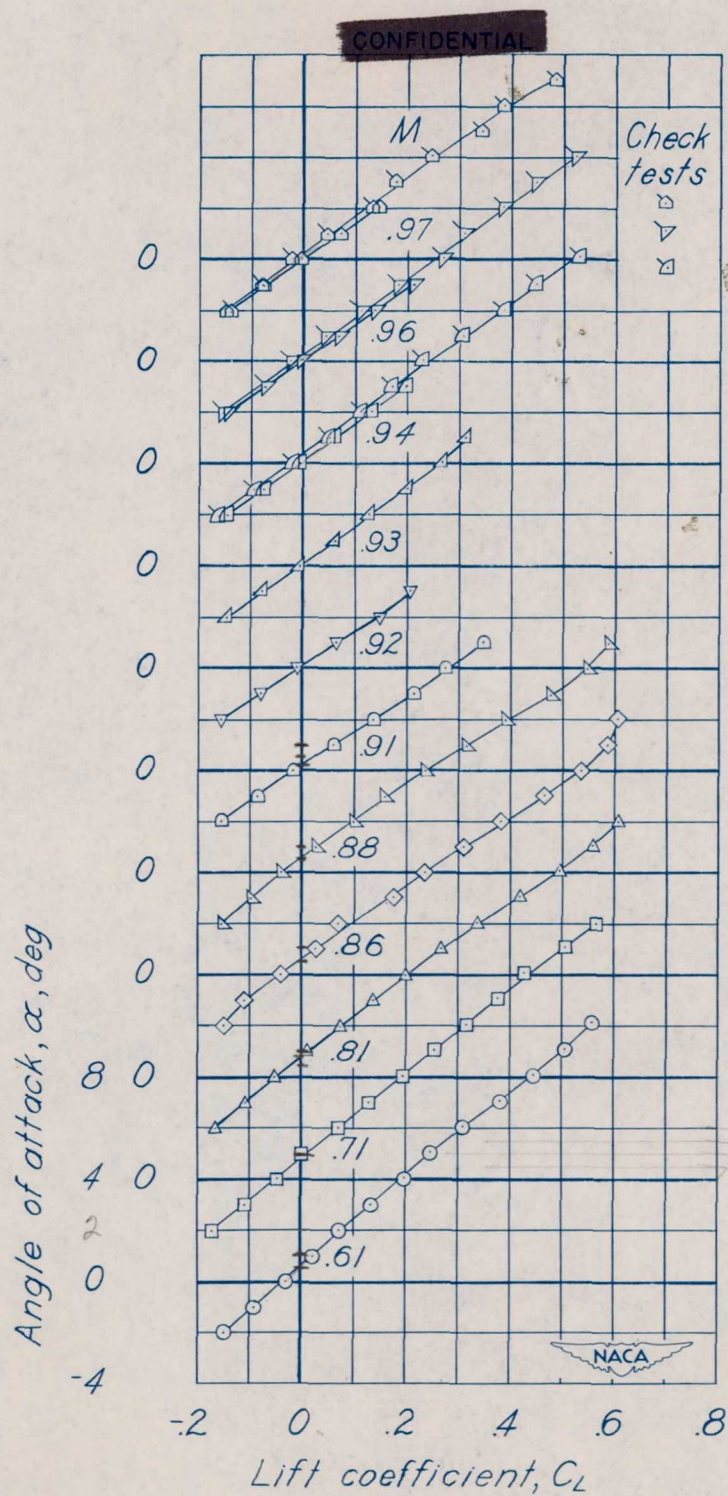
Figure 8.— Aerodynamic characteristics in pitch for various Mach numbers of the 0.08-scale semispan model of the XF7U-1 airplane. Fins on; \delta_a = 0^\circ .
