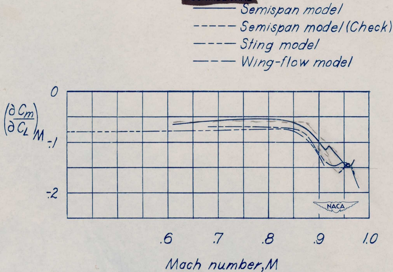
Figure 17.— A comparison of \left(\frac{\partial C_m}{\partial C_L}\right)_M variation with Mach number for the low-lift-coefficient range as obtained by three different test methods on models of the XF7U-1 airplane. Vertical fins on; \delta_a = 0^\circ .
