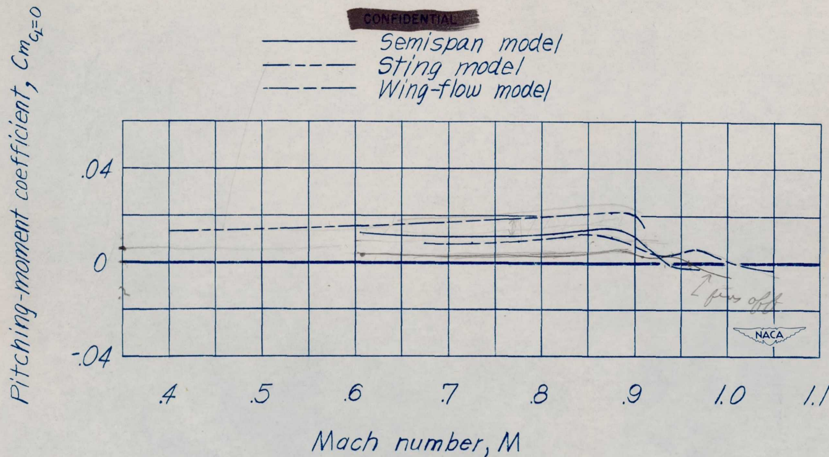
Figure 19.— A comparison of pitching-moment coefficient through the Mach number range at zero lift coefficient as obtained by three different test methods on models of the XF7U-1 airplane. Vertical fins on; \delta_a = 0^\circ .
