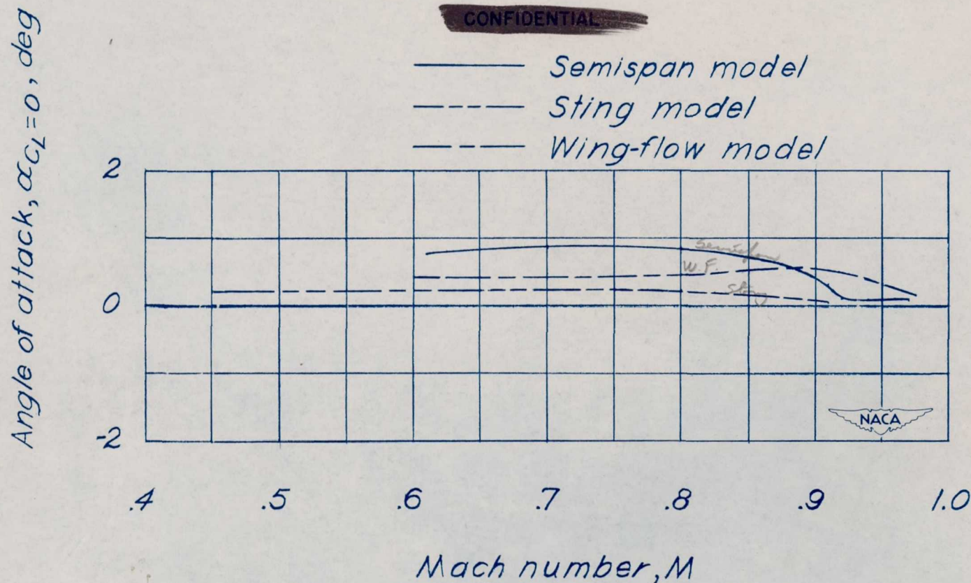
Figure 13.— A comparison of angle of attack at zero lift coefficient through the Mach number range as obtained by three different test methods on models of the XF7U-1 airplane. Vertical fins on, \delta_a = 0^\circ .
