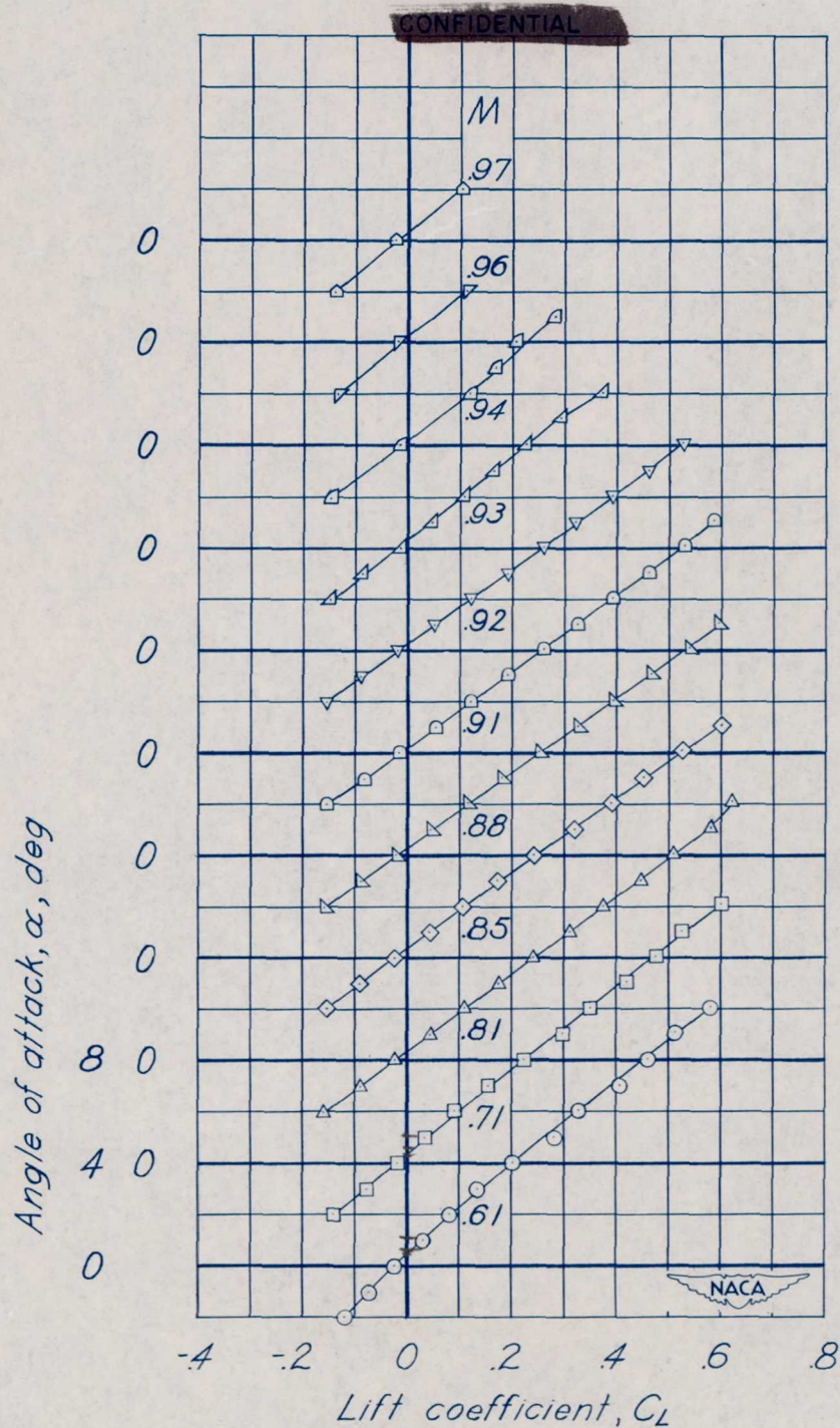
Figure 9.- Aerodynamic characteristics in pitch for various Mach numbers of the 0.08-scale semispan model of the XF7U-1 airplane. Fins off; \delta_a = 0^\circ .
