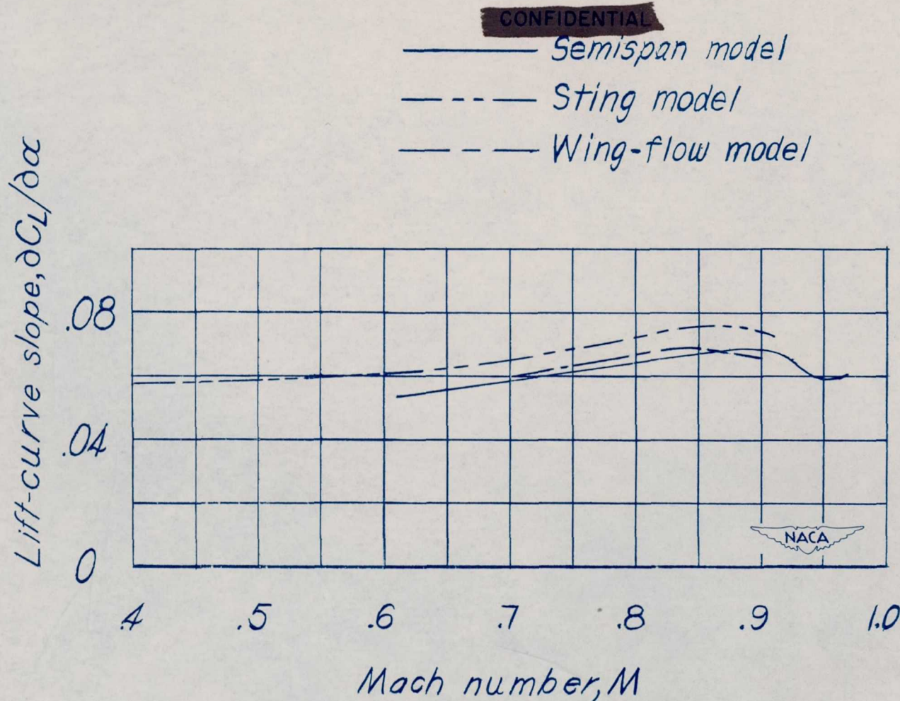
Figure 12.— A comparison of lift-curve slope variation with Mach number in the low-lift-coefficient range as obtained by three different test methods on models of the XF7U-1 airplane. Vertical fins off, \delta_a = 0^\circ .
