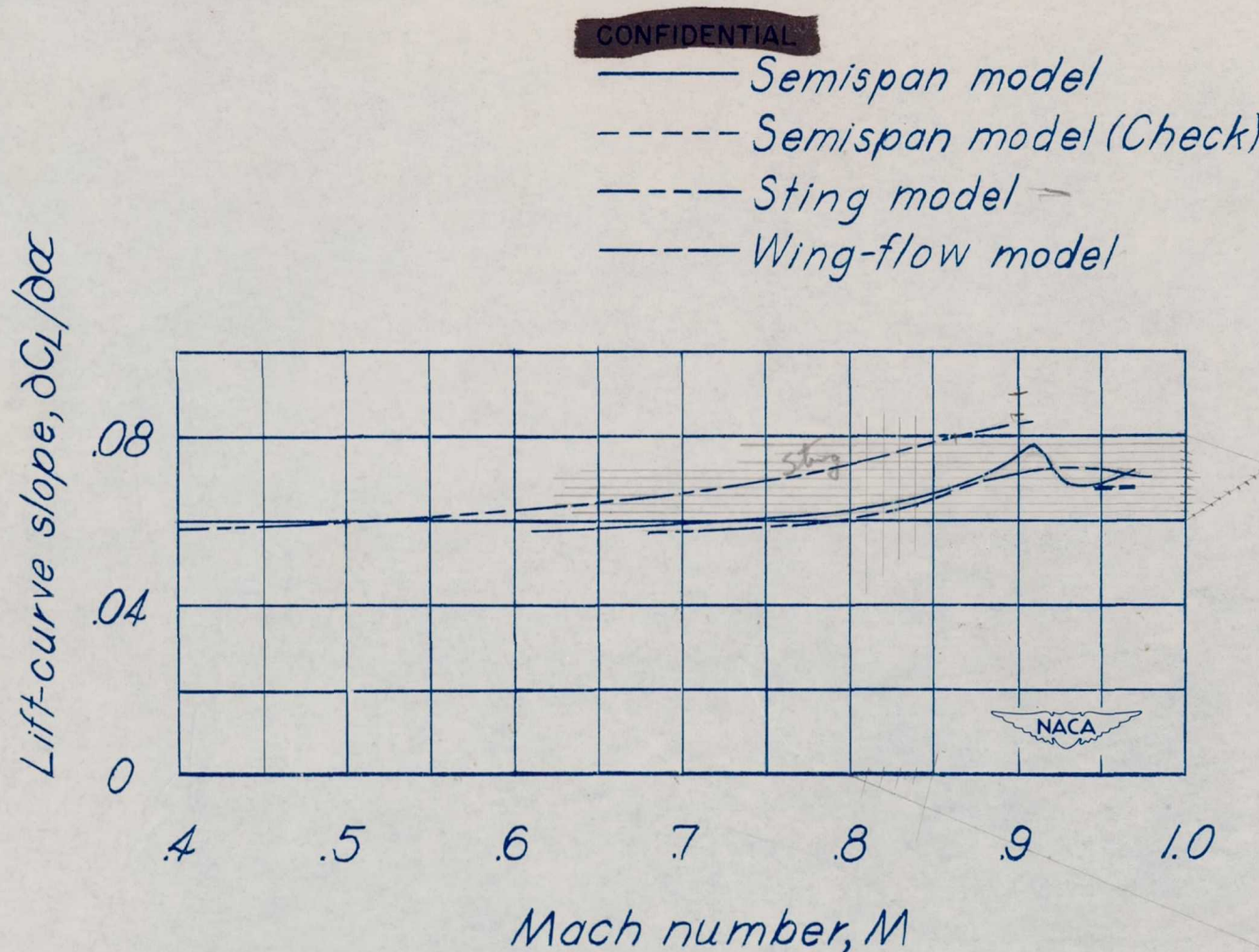
Figure 11.— A comparison of lift-curve slope variation with Mach number for the low-lift-coefficient range as obtained by three different test methods on models of the XF7U-1 airplane. Vertical fins on; \delta_a = 0^\circ .
