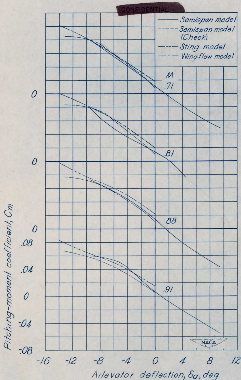
Figure 21.— A comparison of ailavator effectiveness for several Mach numbers as obtained by three different test methods on models of the XF7U-1 airplane. Vertical fins on; C_L = 0 .
