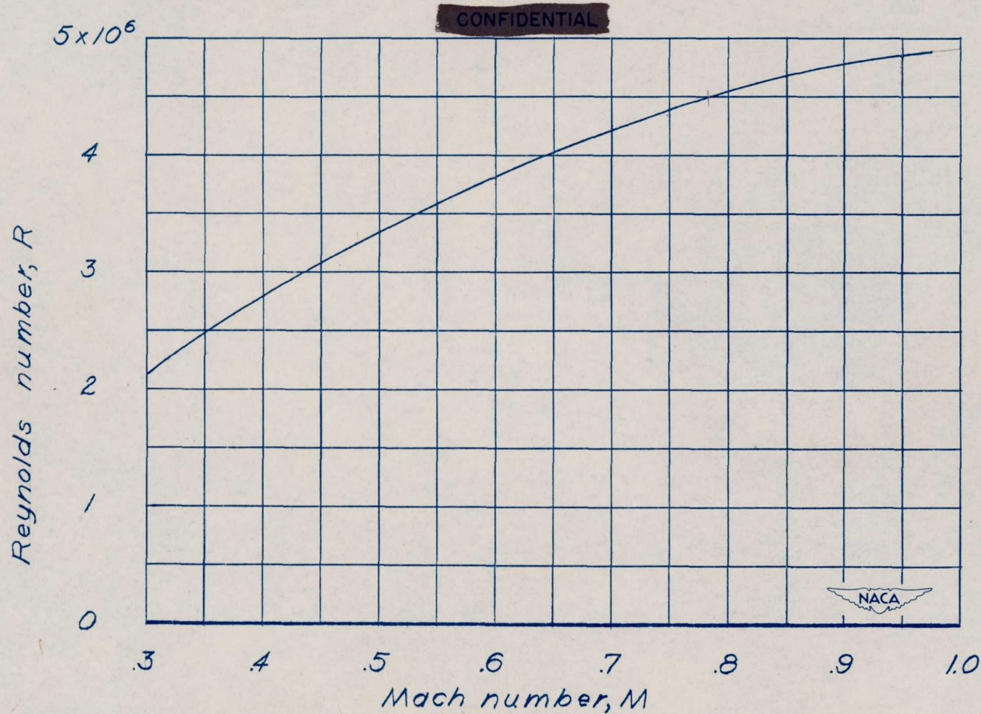
Figure 6.— Variation of test Reynolds number with Mach number for the 0.08-scale model of the XF7U-1 airplane.
