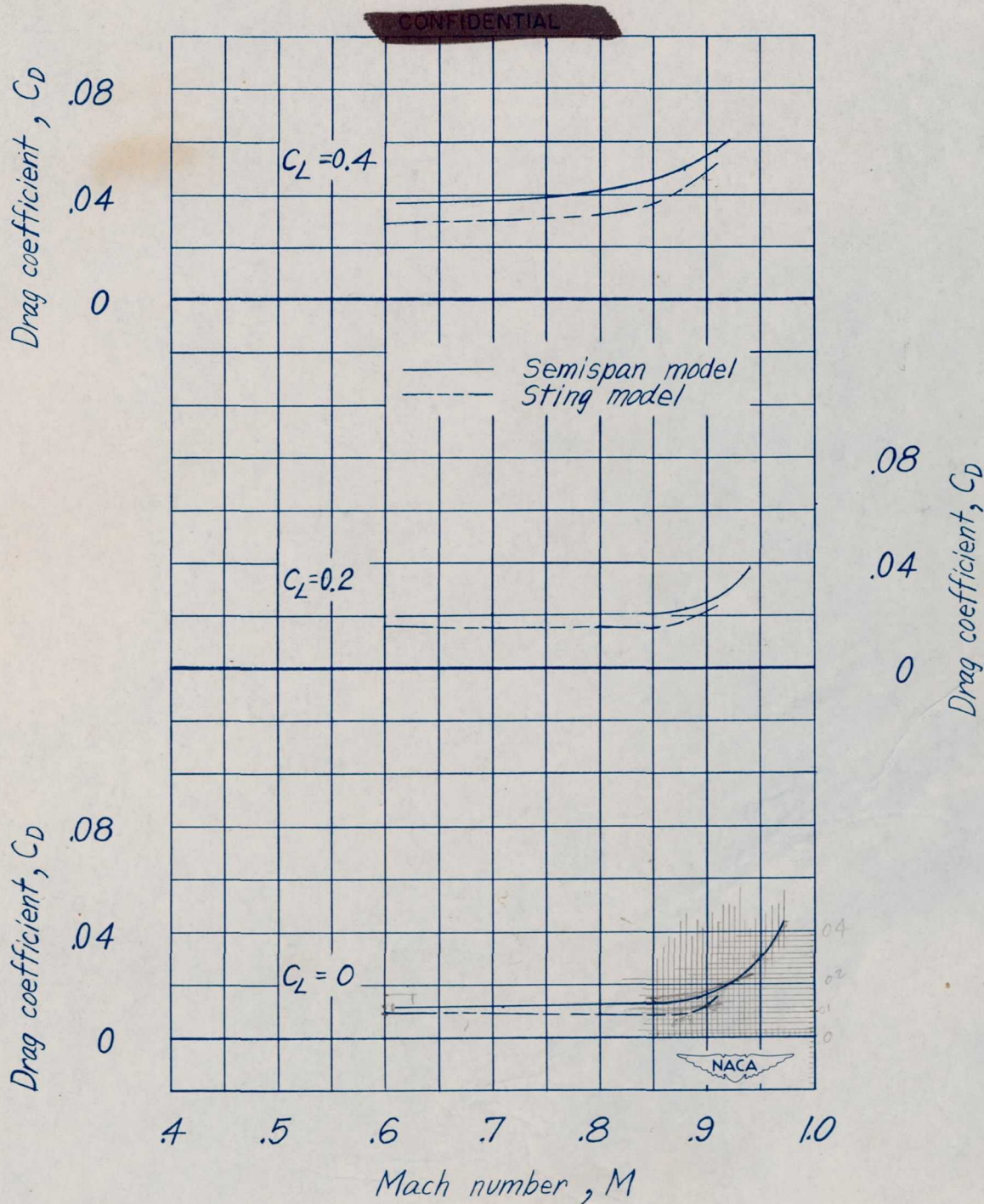
Figure 16.— A comparison of drag coefficient through the Mach number range as measured by the semispan and sting test methods on models of the XF7U-1 airplane. Vertical fins off, \delta_a = 0^\circ .
