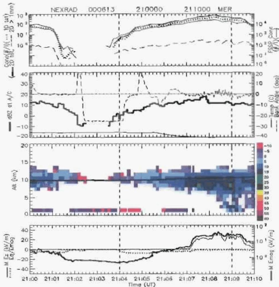
Figure 2.3 Top Panel: Particle concentrations measured by: The PMS FSSP (1 to 48 \mu\text{m} ), light, solid line = total conc. on right scale; The PMS 2D-C (30 \mu\text{m} to \sim 3 mm), bold = total conc., dashed = conc. >1 mm on left; The PMS ID-C (15 to 960 \mu\text{m} ), dotted line = total conc. on left. Second panel: Reflectivity at the location of the aircraft, bank angle of the aircraft and ambient temperature. Third Panel: The curtain of radar reflectivity in the 1x1 km column above and below the aircraft, in this case from the NEXRAD radar; bold line = aircraft altitude. Bottom panel: Vertical component of the electric field, M Ez, light line on left on a linear scale; Eq/Emag dotted on left scale (Eq = apparent field due to charge on the aircraft; Eq/Emag is an indicator of the reliability of the electric field measurement); M Emag, the resultant vector field determined from the M matrix solution, bold line on the right on a log scale. The dashed vertical lines running from top to bottom are time boundaries of individual radar volume scans used to produce the vertical section. For the 10 min period of this plot 3 separate volume scans were used.
