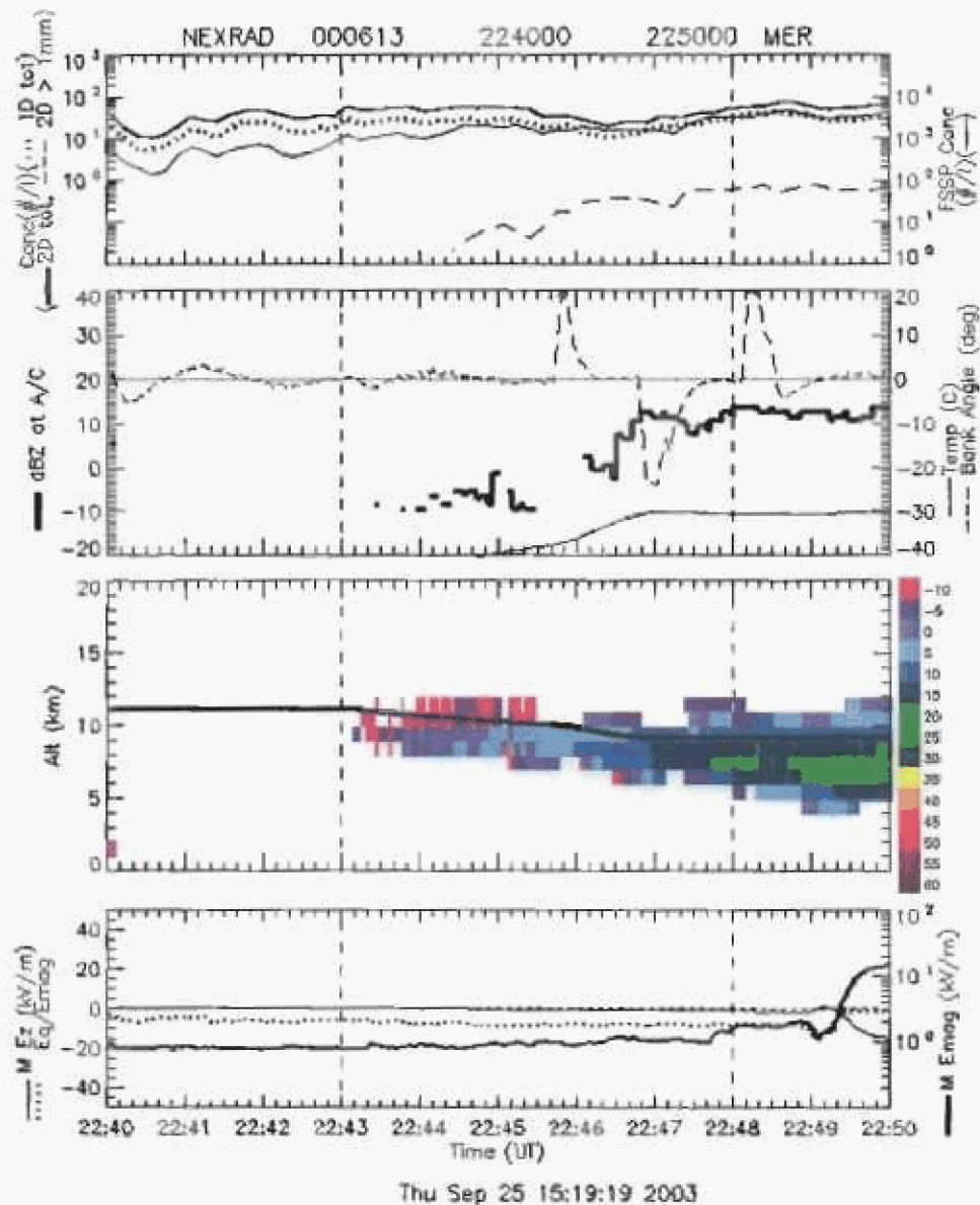
Figure 5.2 As in Figure 2.3 except for the time period 2240 to 2250.
