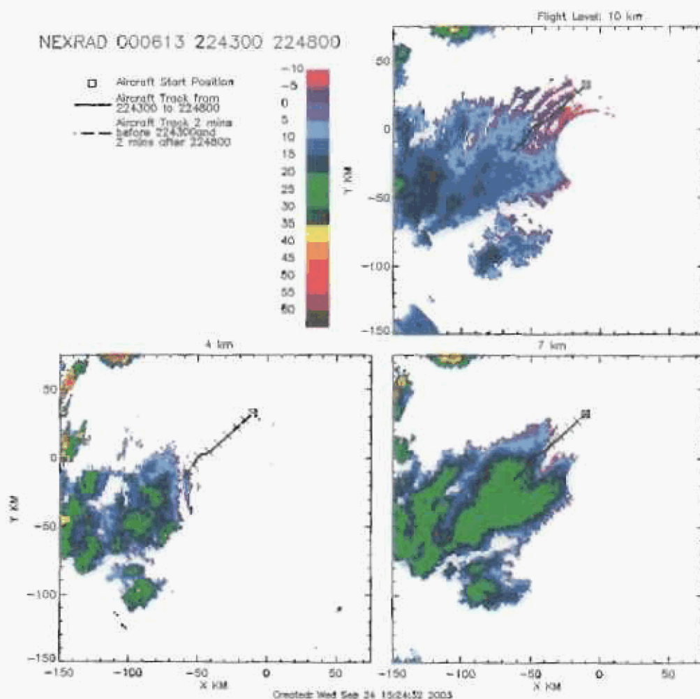
Figure 5.1 As in Figure 2.1 except for the period 2243 to 2248.
