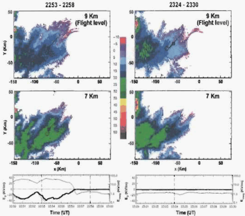
Figure 2.9 CAPPIS at 7 and 9 km for periods as indicated with 9 min of aircraft track overlaid (left: 2251 to 2300 and right: 2332 to 2341). Squares show start of track. Lower Panels: E_z , (bold line, left scale) and magnitude of total field, E_{mag} , (light line, logarithmic right scale) for the periods 2250 - 2300 and 2320 - 2330. In this plot E_{mag} is a light solid line, not the bold line used in MER plots.
