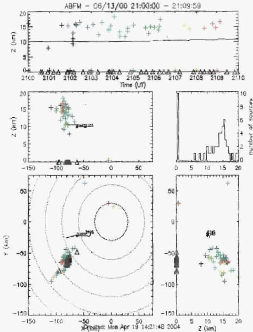
Figure 2.2 Top panel: Display of VHF sources detected by LDAR at the given time (color coded) and altitude. The triangles at the base shows the time of occurrence of CG flashes detected by the KSC CGLSS. The panel on the lower left shows the X,Y location relative to the WSR74C radar of LDAR sources and CG flashes detected during this 10 min time period. The panels above and to the right of the XY display show VHF sources and CG flashes in a XZ and YZ presentation. Track of the aircraft during the 10 min time period is overlaid. For more information on the LDAR and CGLSS systems see Appendices F and G, respectively.
