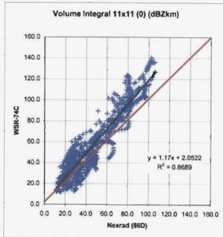
Figure 5.15 Comparison of the 11x11Volume Integral determined by 74C and NEXRAD.
