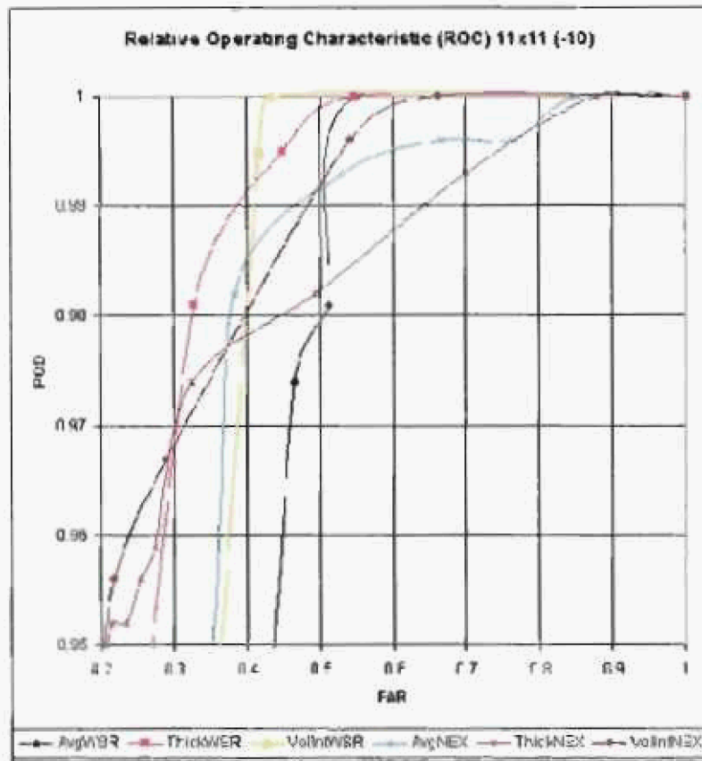
Figure 5.16 ROC curve for 74C and NEXRAD for 11x11ColumnAverage, 11x11 Average anvil thickness, and 11x11VolumeIntegral. Copied from Merceret (2004).
