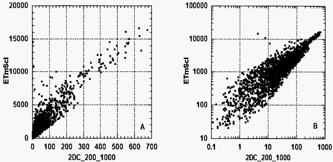
Figure 4.1 EtmScl (sec) as a function of particle concentration for 200 to 1000 \mu measured by the 2DC. (A) EtmScl plotted on a linear scale. (B) Plotted on a log scale.
