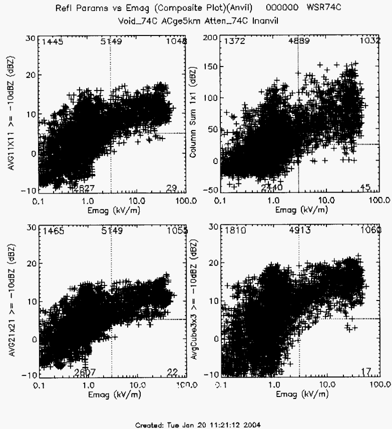
Figure 5.7 Same as figure 5.6 but only for periods “In-Anvil”. The number at the top, middle of each plot shows the total number of points in the plot with the four numbers in each corner indicating the number of points in each quadrant defined by the dotted horizontal and vertical line.
