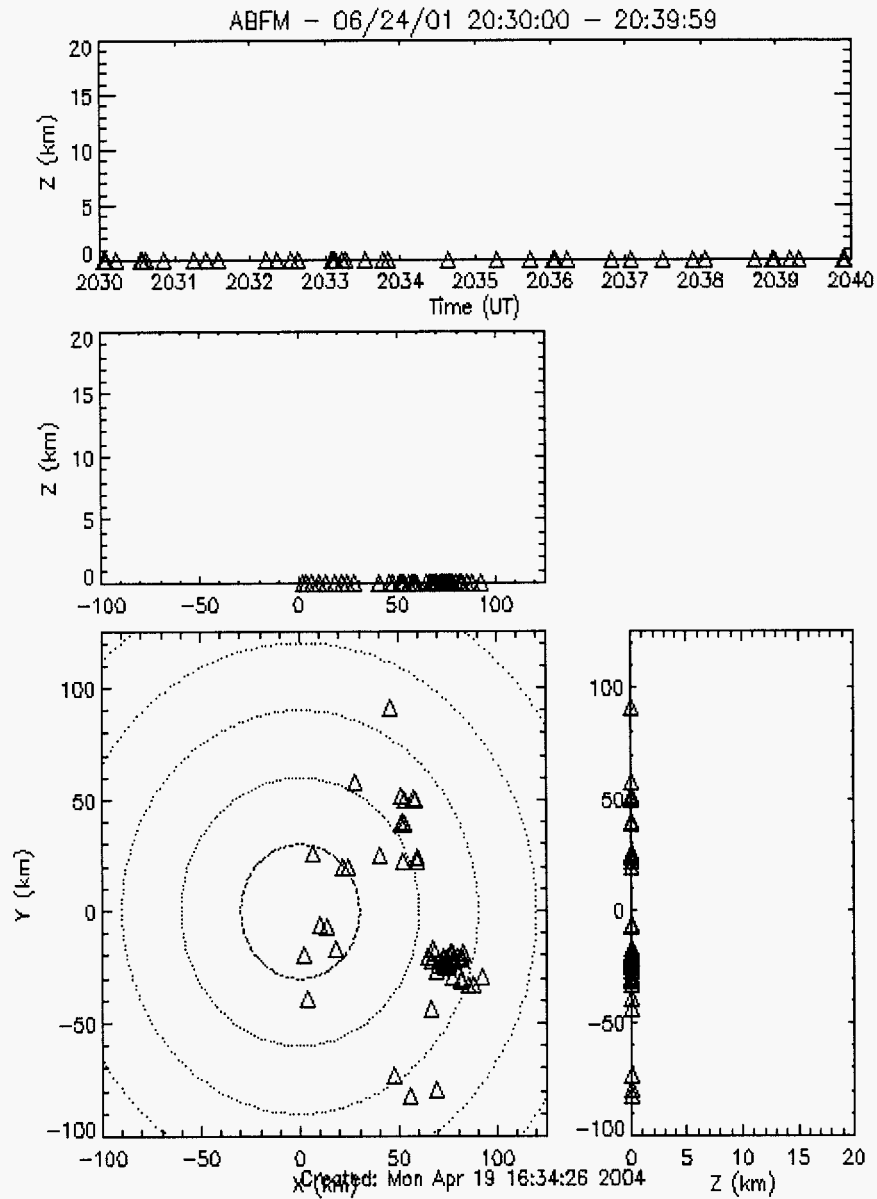
Figure F.3 Lightning plots from 010624 showing no LDAR sources, but plenty of CGs.
