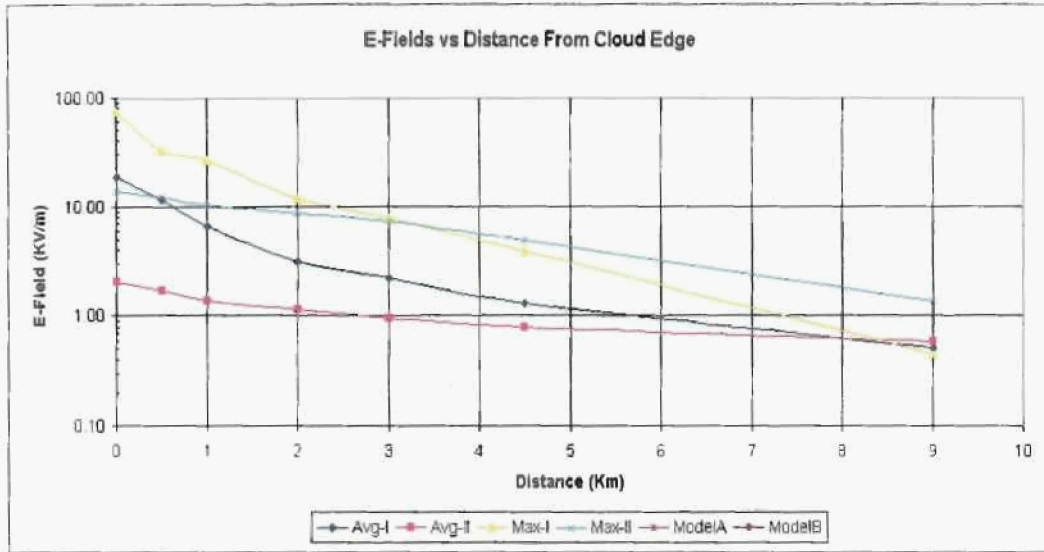
Figure 6.1 Electric field plotted as a function of distance from cloud edge. Avg I and Max I are average and maximum measurements from ABFMI, respectively and Avg II and Max II are from ABFM II.
