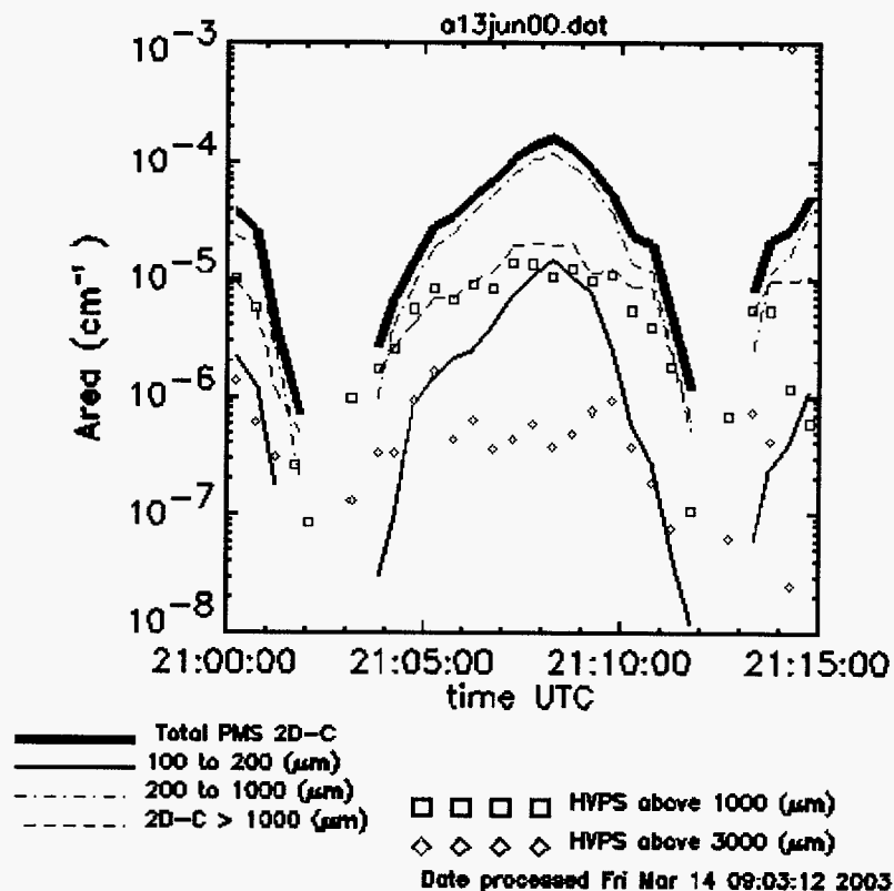
Figure 2.8 Time series plot of 30 second average values of particle cross sectional area for different probes and size intervals as indicated.
