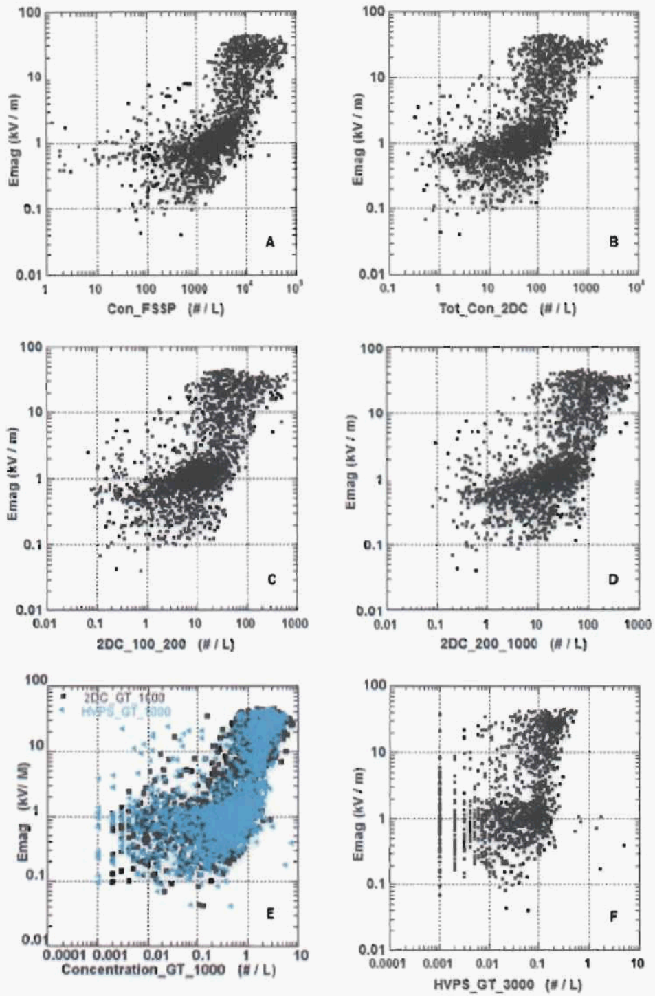
Figure 3.2 Plots of Emag as a function of concentrations measured by different sensors in different size ranges as labeled.
