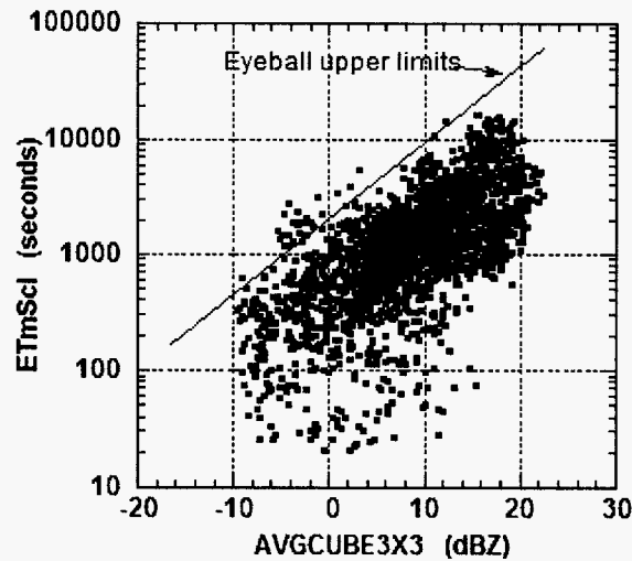
Figure 4.2 Electrical decay time scale (ETmScl in seconds) versus the average reflectivity in a 3km cube centered on the aircraft location and altitude. The diagonal line is an “eyeball” fit of the upper envelope of most points.
