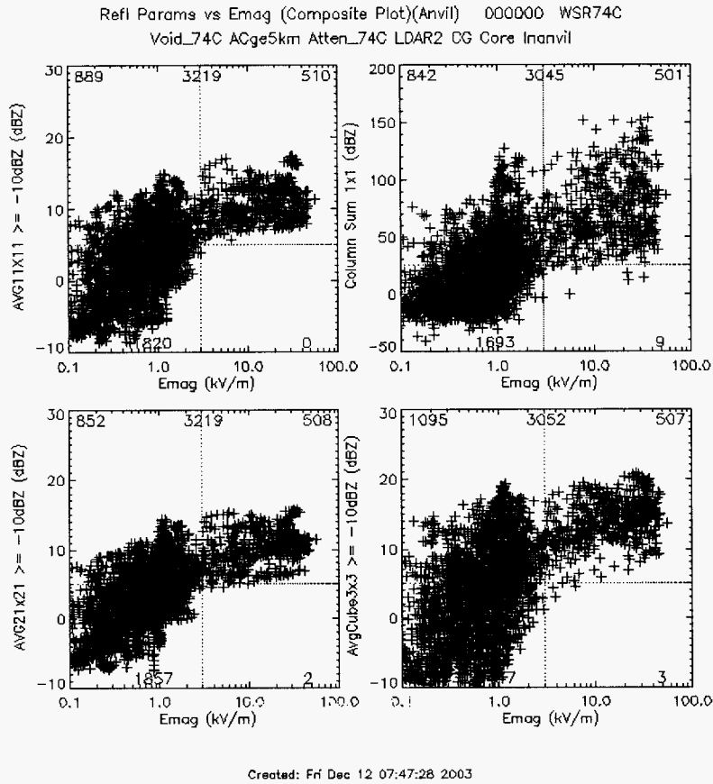
Figure 5.8 Same as figure 5.7 but filtered to remove data when the aircraft was flying near lightning or convective cores.
