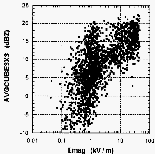
Figure 3.5 Same as Figure 3.4 except with reversal of the X and Y axes.
