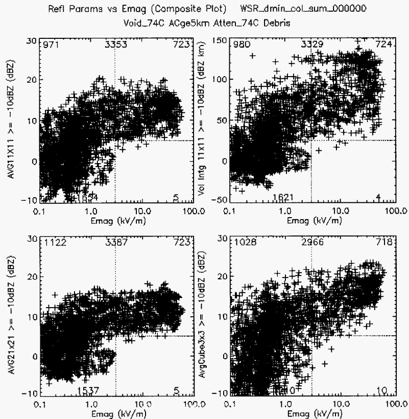
Figure 6.2 Scatter plot of reflectivity parameters as indicated versus Emag for debris clouds with minimum filtering for 74C attenuation, periods when the Citation was flying in the cone of silence above the 74C radar, and when the aircraft was at altitudes < 5 km MSL.
