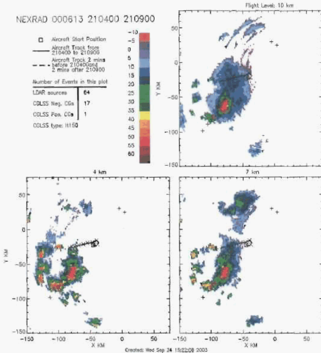
Figure 2.1 CAPPIs at 4, 7 and 10 km MSL showing the Citation track for the period as indicated. CG flashes detected by the CGLSS system are overlaid as red triangles and LDAR VHF sources as black pluses for the period of this volume scan (2104-2109). This storm was ~150 km from LDAR so the detection efficiency was low.
