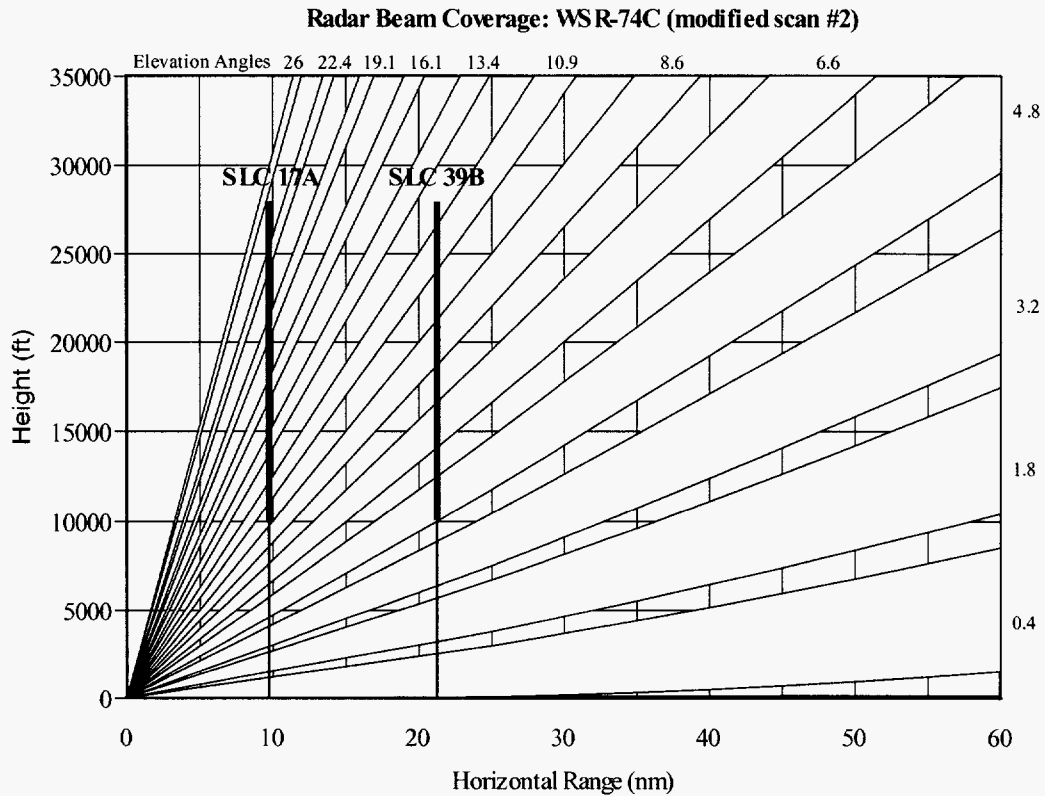
Figure D.1. Vertical cross-section of beam coverage by current WSR-74C volume-scan using 12 elevation angles. Ignore the label "modified scan #2". The elevation angle sequence is designed to produce vertical gaps between half-beamwidths that are constant with range at a fixed altitude. A beamwidth of 1.1^\circ was used. The vertical lines indicate the locations of SLC 39B and SLC 17A relative to the radar. The line is thickened between 10 400 ft and 27 600 ft to emphasize the layer where mixed phase processes and electrification are most likely to occur within clouds. The elevation angles are 0.4^\circ , 1.8^\circ , 3.2^\circ , 4.8^\circ , 6.6^\circ , 8.6^\circ , 10.9^\circ , 13.4^\circ , 16.1^\circ , 19.1^\circ , 22.4^\circ , and 26.0^\circ .
