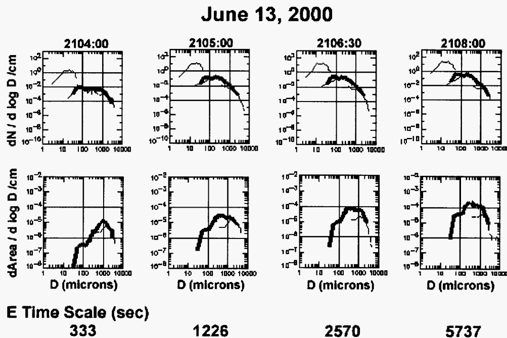
Figure 2.6 Top panel: Concentration size distributions (30 sec averages) for the indicated initial times during the Citation pass shown in Figure 2.1 and 2.3. Bottom panel: Particle cross sectional area size distribution for the same 30 sec time periods. Light line on the left side of each plot -- FSSP (off scale for area plots); Bold line – 2D-C; light line on right of each plot -- SPEC High Volume Particle Spectrometer, HVPS, (~400 \mu\text{m} to ~5 cm range).
