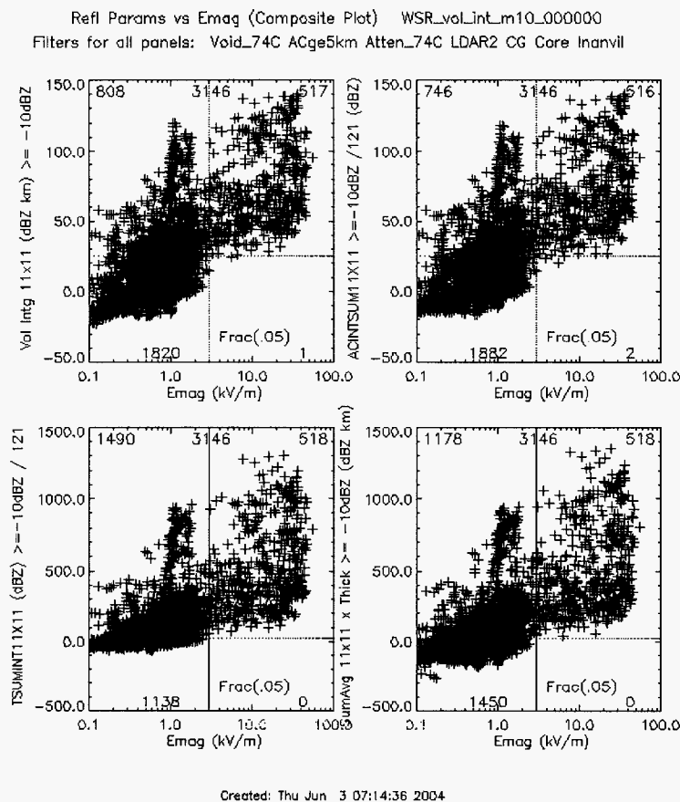
Figure 5.11 Scatter plots of various 11x11 column integrated volume reflectivities. Upper left: Volume Integral, (11x11ColumnAvg x Avg 11x11Thickness). Upper right: ACIS, (Integrated Sum of 1x1 km AvgColumn reflectivity). Lower left: TSum Integrated Reflectivity ([sum of dBZ for all 1 km pixels in the 11x11 Column]/121). Lower right: SumAvgInt (average dBZ in each 11x11 plane summed over each altitude x Avg 11x11Thickness).
