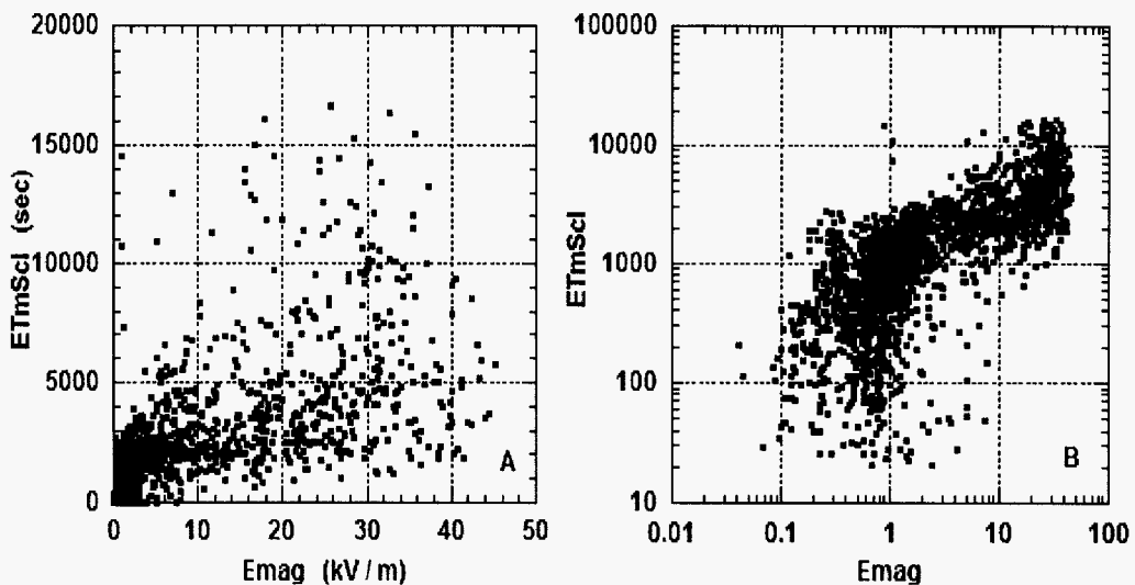
Figure 4.3 Electrical decay time scale plotted as a function of electric field using linear scales ( A ) and logarithmic scales ( B ).
