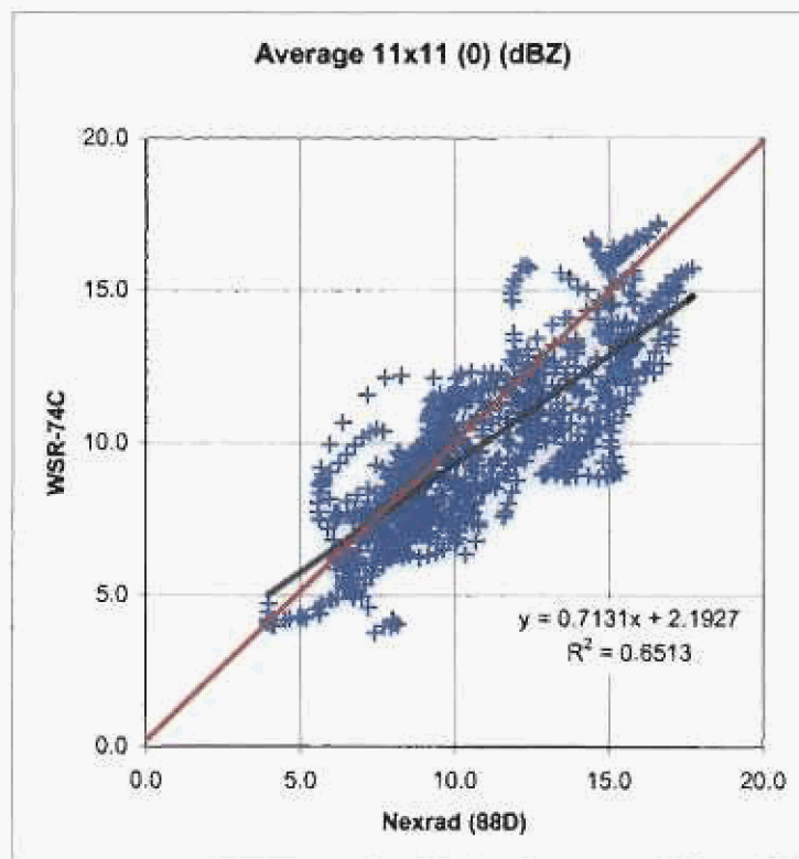
Figure 5.13 11x11 Column Average reflectivity from the WSR74C radar at Patrick Air Force Base compared to the WSR88D NEXRAD radar at Melbourne Florida.
