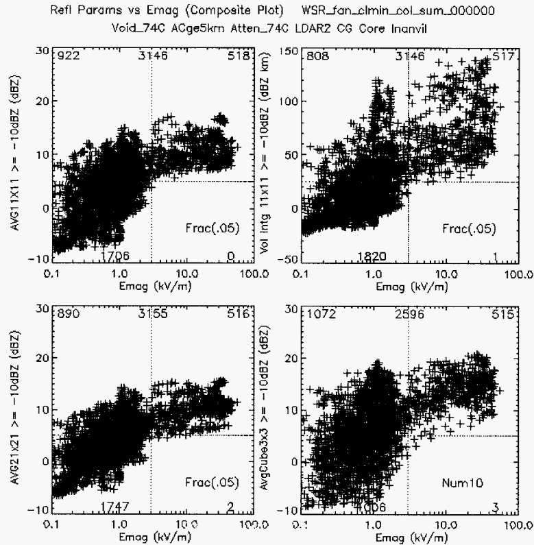
Figure 5.10 Same as figure 5.9 but 11x11 Volume Integral instead of 1x1ColSum.
