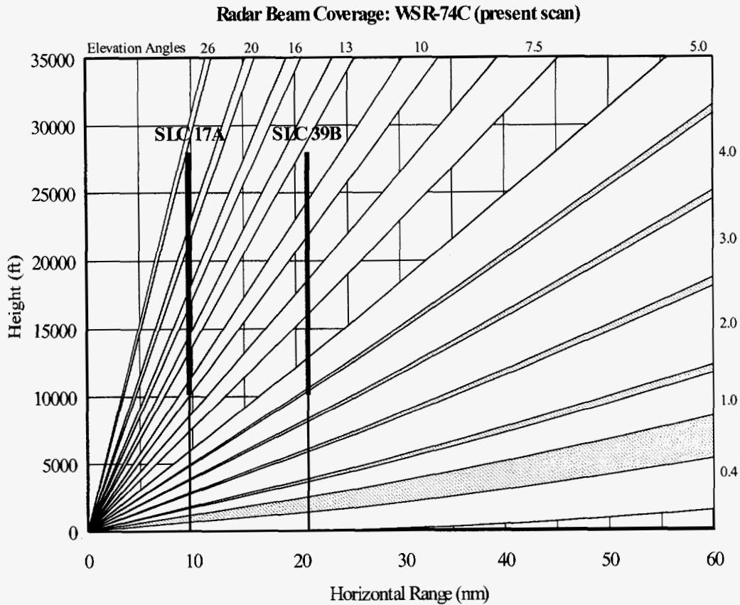
Figure D.2. Vertical cross-section of beam coverage by older WSR-74C volume-scan. Ignore the label "present scan". A beamwidth of 1.1^\circ was used. The stippled pattern indicates overlapping coverage by adjacent beams. The vertical lines indicate the locations of SLC 39B and SLC 17A relative to the radar. The lines are thickened between 10 400 ft and 27 600 ft to emphasize the layer where mixed phase processes and electrification are most likely to occur within clouds. The elevation angles are 0.4^\circ , 1.0^\circ , 2.0^\circ , 3.0^\circ , 4.0^\circ , 5.0^\circ , 7.5^\circ , 10.0^\circ , 13.0^\circ , 16.0^\circ , 20.0^\circ , and 26.0^\circ .
