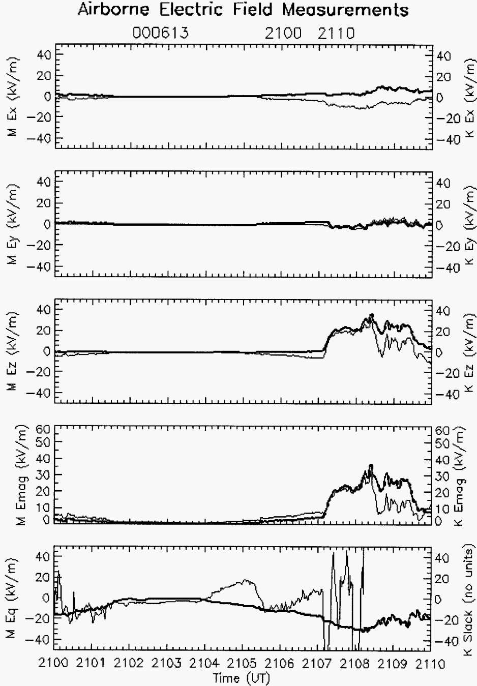
Figure 2.4 First four panels: the E_x , E_y and E_z electric field components (relative to the aircraft attitude) and the magnitude of the total electric field as determined from the M matrix solution (Bold line and left axis for all) and the K matrix solution (light line and right axis). Bottom panel: M_{Eq} , field due to charge on the aircraft from the M solution and K slack, residuals from the K solution.
