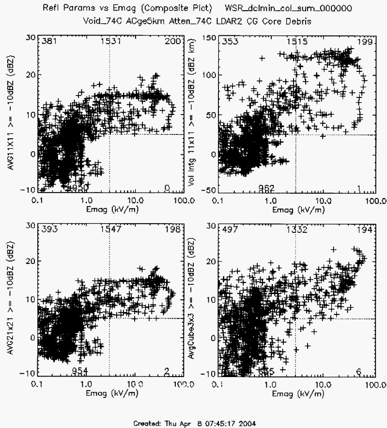
Figure 6.3 Same as figure 6.1 except the debris cloud data set has been filtered for nearby lightning and convective cores.
