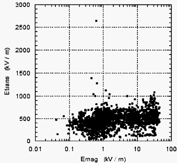
Figure 4.5 The electric field value ( E_{\text{trans}} ) at which attachment of ions to hydrometeors by diffusion becomes equal to that by field driven attachment is plotted as a function of the magnitude of the electric field ( E_{\text{mag}} ).
