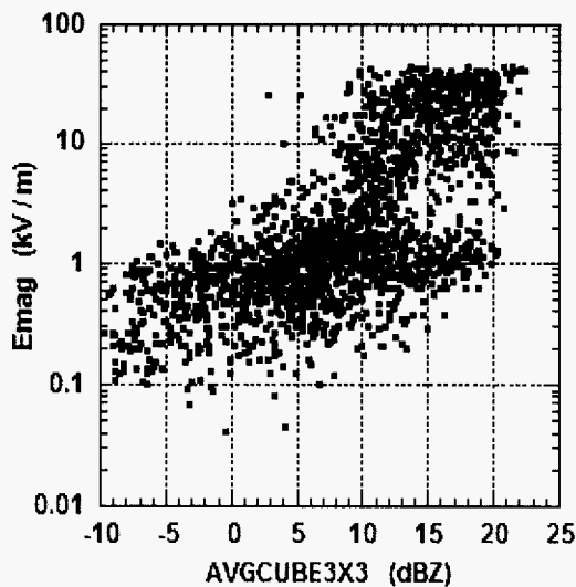
Figure 3.4 E_{mag} plotted as a function of 3km Cube average reflectivity.
