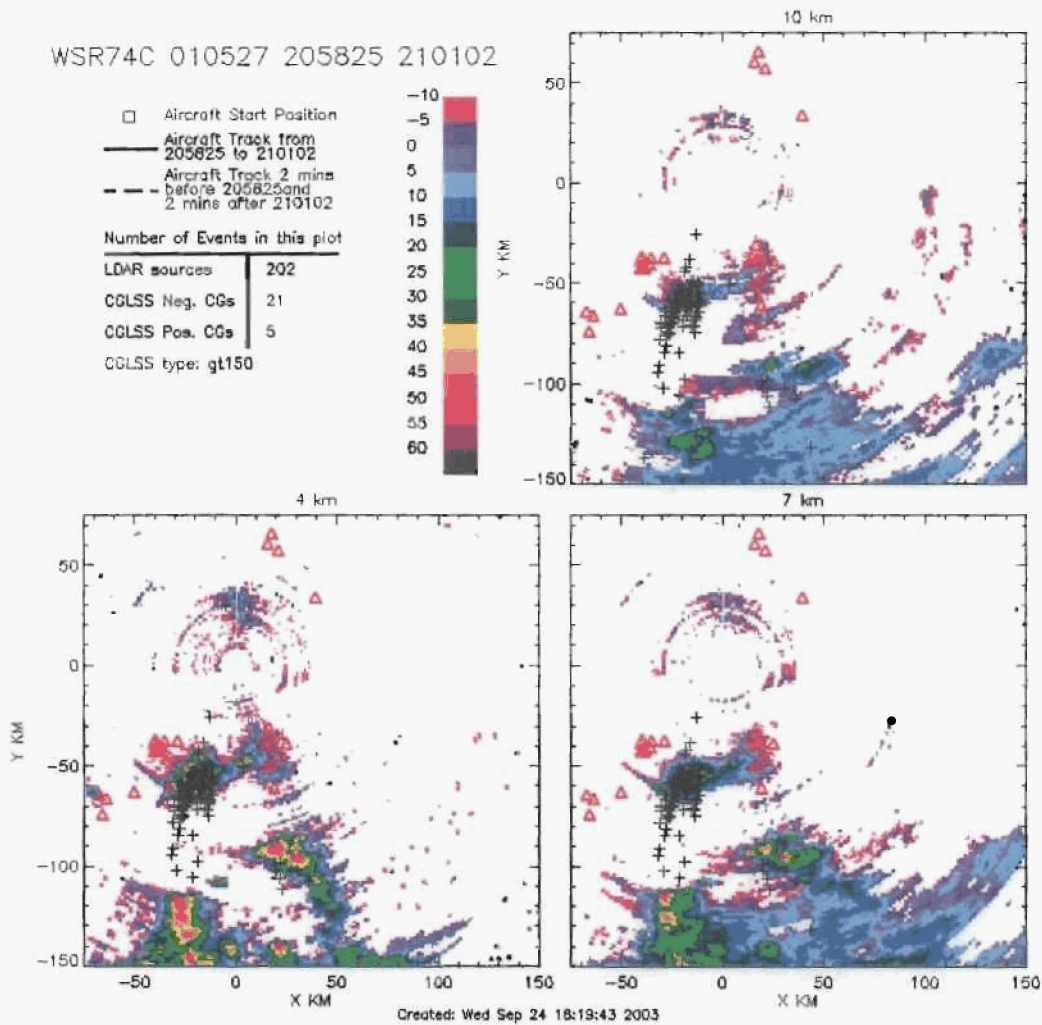
Figure G.2 Capii with Lightning for 010527 showing CGs (red triangles) where there is no LDAR sources (black '+') and no reflectivity.
