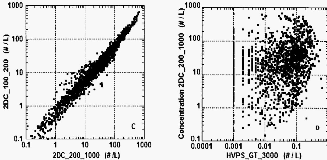
Figure 3.1 (A) Total FSSP concentration vs. concentration of particles from 2DC >1000 \mu . (B) Total 2DC concentration vs. concentration of particles from 2DC >1000 \mu . (C) 2DC concentration of particles 100 to 200 \mu vs. concentration of 200 to 1000 \mu . (D) 2DC concentration of particles 200-1000 \mu vs. HVPS concentration of particles >3000 \mu .
