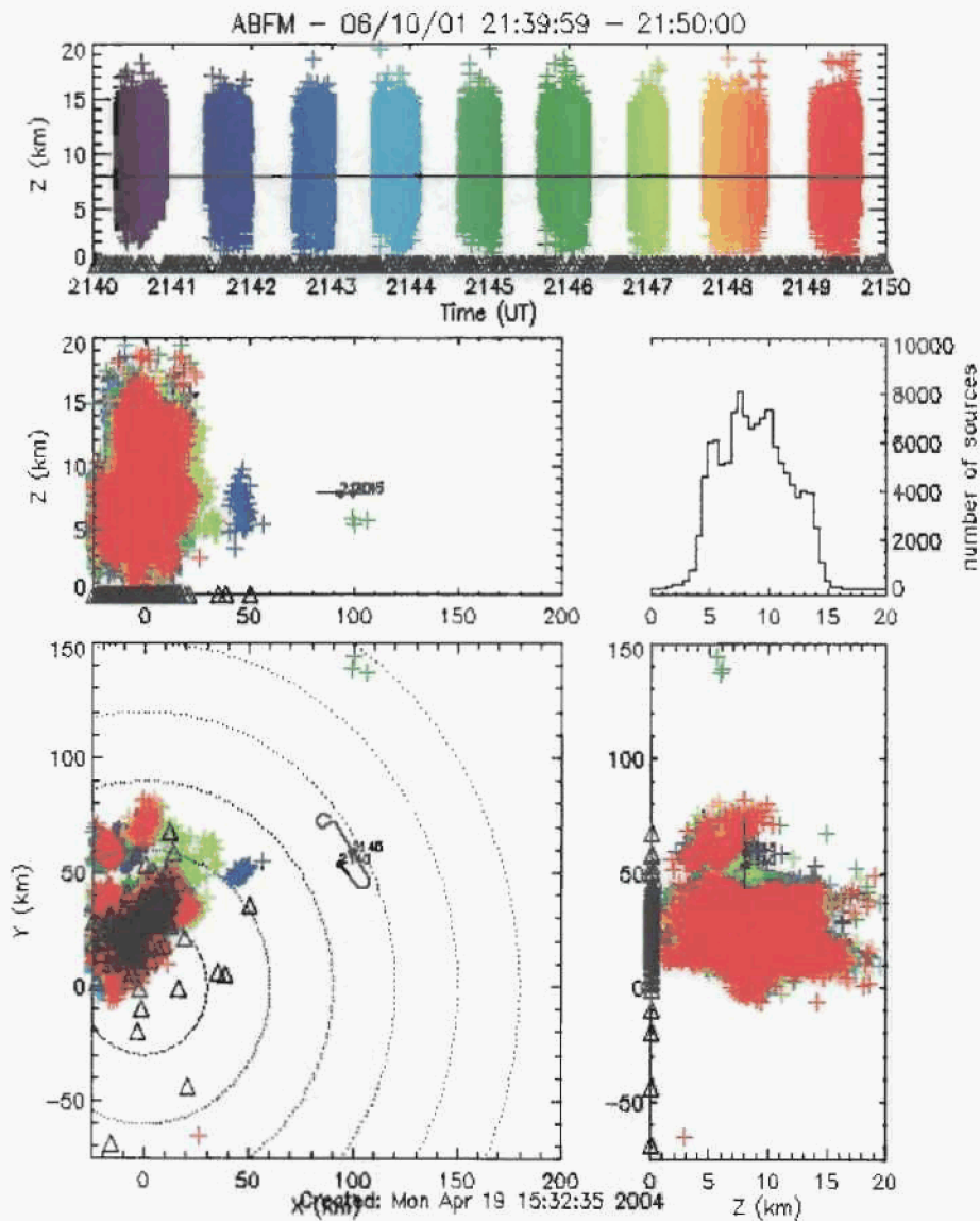
Figure F.2 Lightning plots from 010610 showing a case where the LDAR intermittently stopped showing sources.
