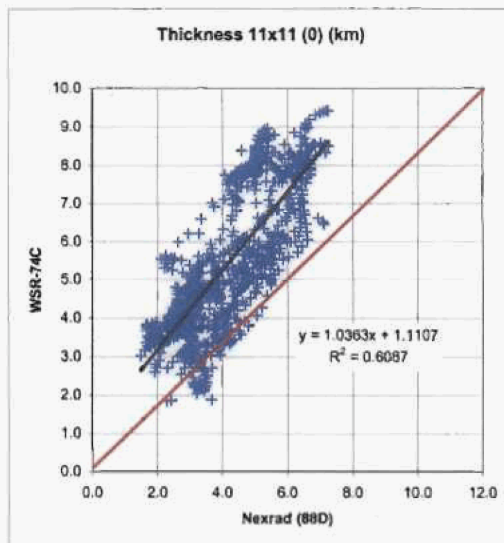
Figure 5.14 Comparison of anvil thickness determined from 74C and NEXRAD measurements using a 0 dBZ cutoff.
