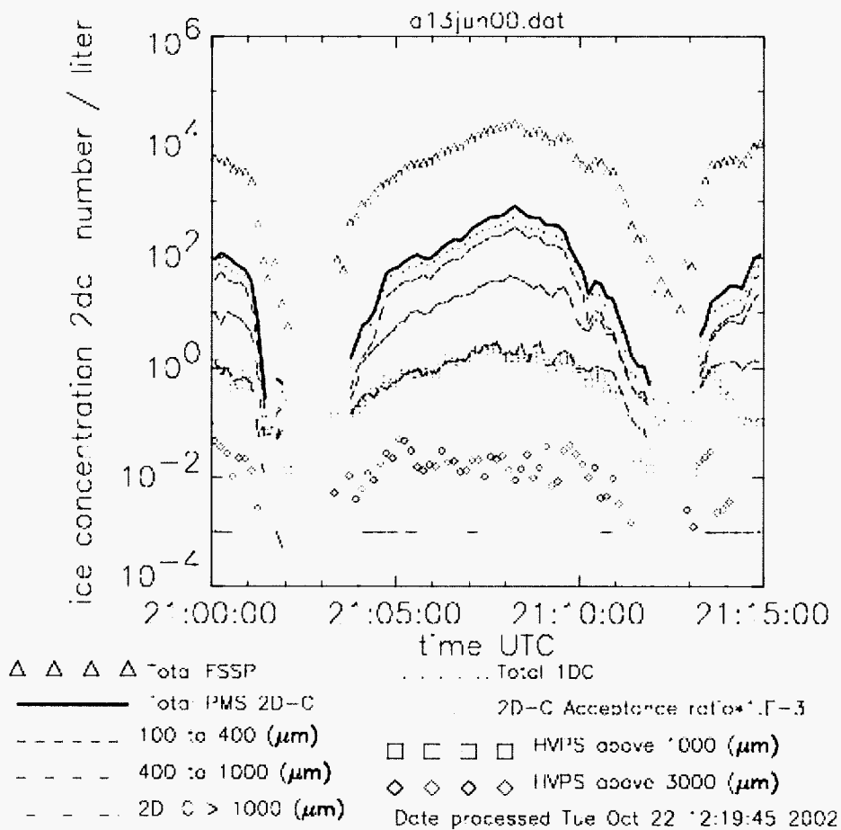
Figure 2.5 Time series plots of 10 second average values of particle number concentration for different probes and size ranges as indicated.
