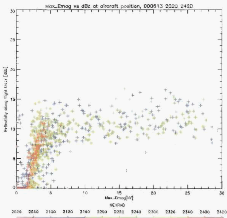
Figure 5.4 Reflectivity at the aircraft versus Emag for entire flight of June 13, 2000.
