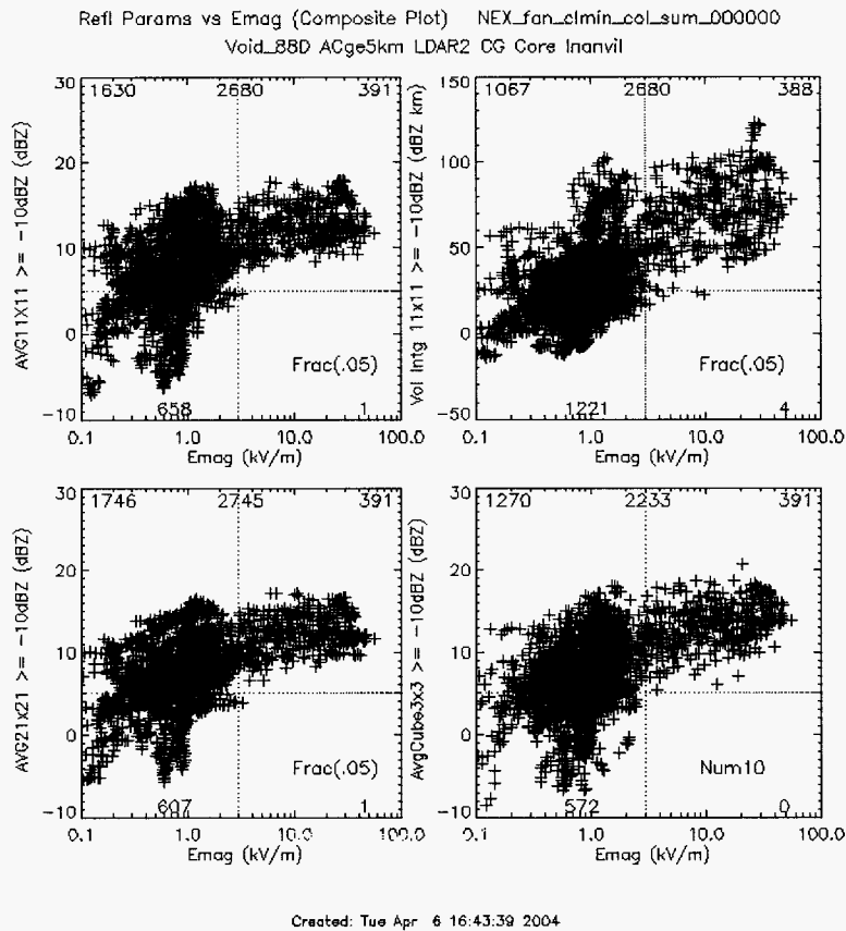
Figure 5.12 Same as Figure 5.10 but for NEXRAD rather than WSR74C. Minimum, In-Anvil, lightning, core, and Frac filters have been applied to the data set.
