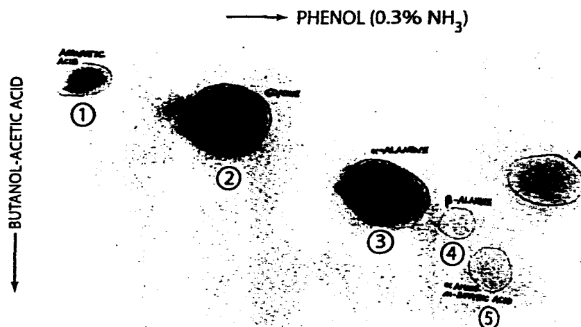
Figure 2. The two-dimensional paper chromatogram of the amino acids produced from the sparking experiment using the apparatus shown in Figures 1a and b (courtesy of Stanley L. Miller). The spots corresponding the various amino acids were produced by spraying the chromatogram with ninhydrin. The amino acid labels are Stanley's original writing. We have added numbers to help identify the various spots. 1 = Aspartic acid; 2 = glycine; 3 = \alpha -alanine; 4 = \beta -alanine; and 5 = \alpha -amino-n-butyric acid. Spots labeled A and B where not identified.
