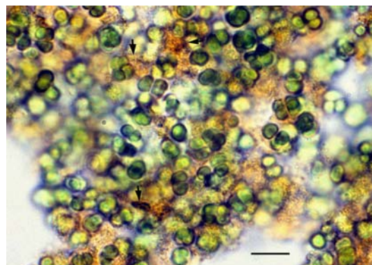
Fig. 1. Light micrograph of the isolate 5.2 s.c.1 grown in liquid medium DH supplemented with 400\mu\text{M Fe}^{3+} , indicating iron-containing precipitates on cell surfaces (black arrows). Bar = 5\mu\text{m} .
