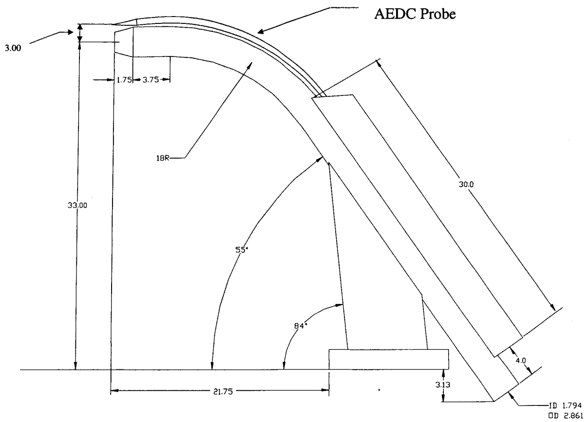
Fig. 1. AEDC particulate probe (dimensions are in inches).
