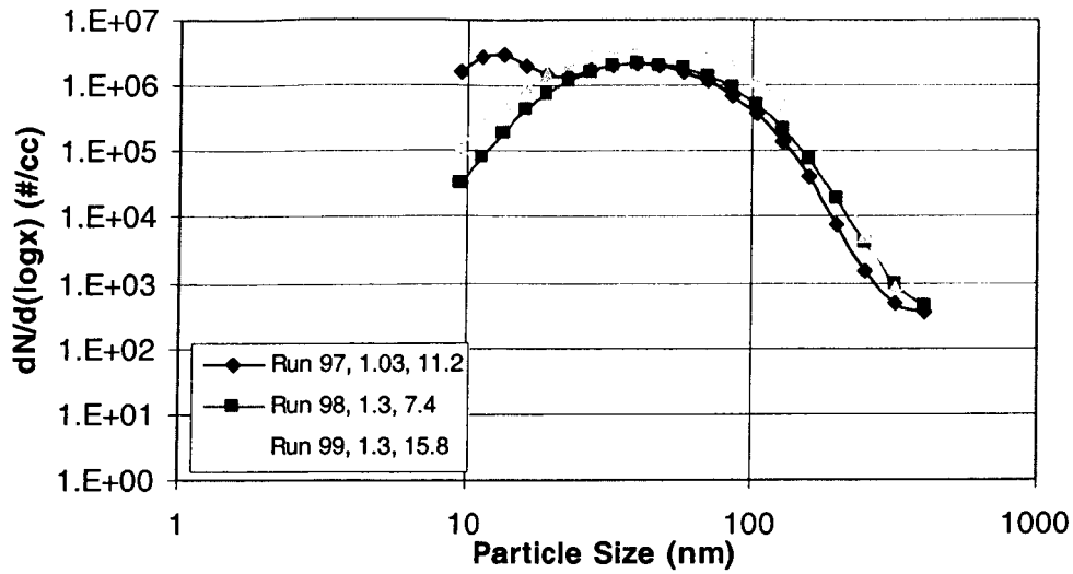
Fig. 3. Particle size distributions, probe distance 1 m, fuel sulfur content 810 ppm; parameters are engine pressure ratio and dilution ratio.
