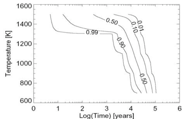
Figure 2. Probability distribution functions (PDFs) for time spent at greater than some temperature T , for survivors released at 1500K, and t=0 .
