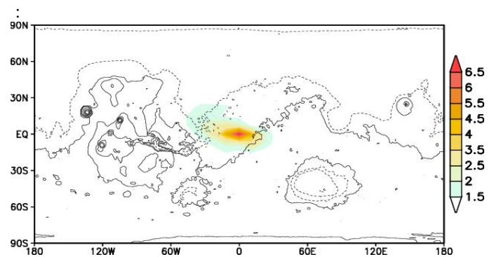
Figure 1: Relative column abundance of a gas with localized source at 0°N 0°E and lifetime of 10 7 s (~100 days) after 10 years. The gas column abundance has been scaled with surface pressure to remove the topography effects and normalized to the global mean abundance.
