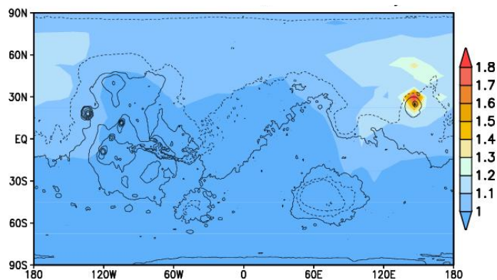
Figure 2: Same as Fig. 1 but for a gas released from the Elysium area with a lifetime of 10^{10} s (320 Earth years; like methane in theory) and after 0.6 Martian years. The local maximum above the source is still significant in spite of the very long lifetime of the gas.
