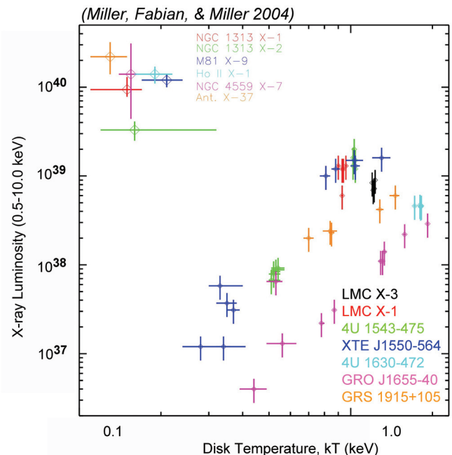
Figure 2: Black hole X-ray luminosity versus implied accretion disk temperature, for a number of stellar-mass black holes in the Milky Way and Large Magellanic Cloud, and a number of the brightest ultraluminous X-ray sources in nearby galaxies. The sources in the upper left hand corner are IMBH candidates. Constellation-X will make definitive spectroscopic and timing measurements to strongly confirm or reject the existence of intermediate-mass black holes.
