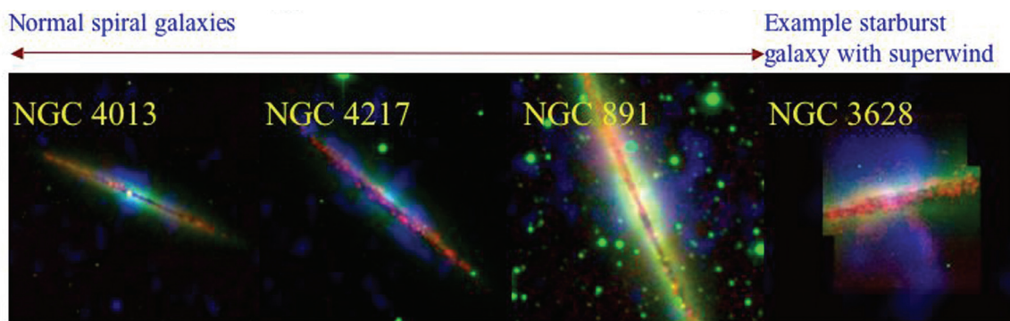
Figure 6: Hot gas around normal disk galaxies - Red: H\text{-}\alpha (WIM), Green: R-band (starlight), Blue: Diffuse soft X-ray ( 3 \text{ million}^\circ gas). The region covered by each image is 20 \times 20 kpc. Intensity scale in square-root.
