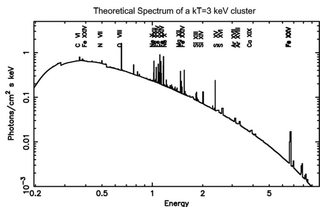
Figure 2: Theoretical spectrum of an isothermal plasma with kT \sim 3 keV, with many of the strong transitions labeled; however, many of the transitions from the same ion (e.g., multiple lines from Fe XXIV) have been suppressed. Note the strong lines from all the abundant elements. The data are plotted in the usual way for X-ray astronomers, photons \text{cm}^{-2} \text{s}^{-1} \text{keV}^{-1} vs. energy in keV, which emphasizes the dynamic range of X-ray spectroscopy.
