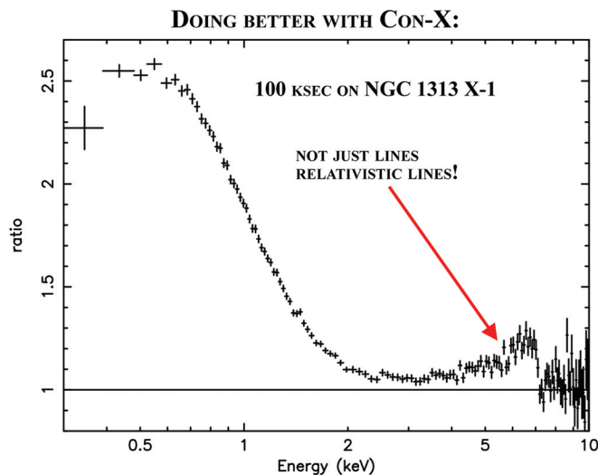
Figure 3: The plot above shows a simulated Constellation X spectrum of the intermediate-mass black hole candidate NGC 1313 X-1, plotted as a ratio to a simple power-law model. A 100 ksec exposure with Constellation-X will clearly reveal the cool accretion disk component glimpsed with XMM-Newton (Miller et al. 2003).
