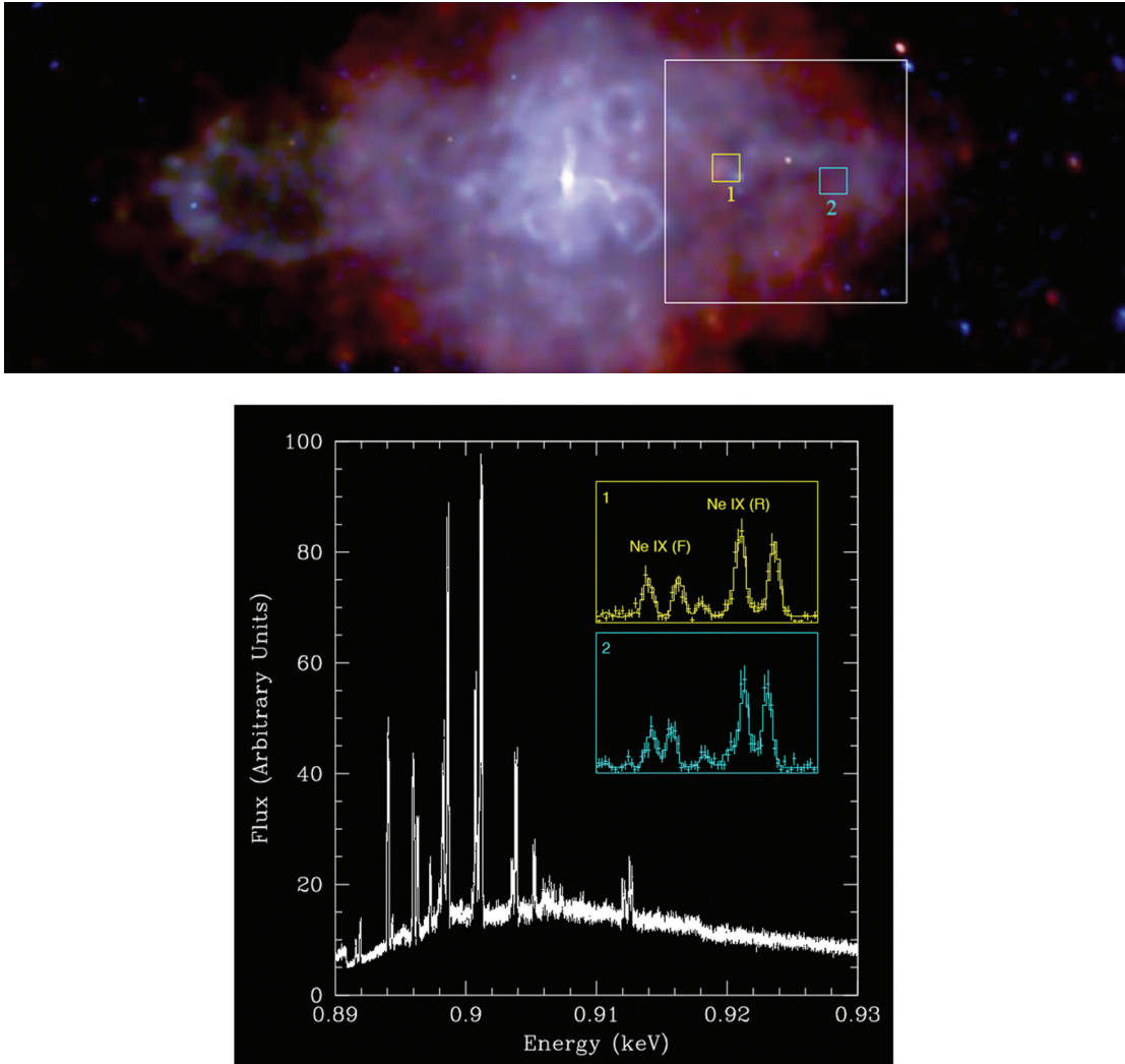
Figure 6: (top): Chandra image of 3C 58 with the Constellation-X calorimeter field of view (white) and two 15'' \times 15'' extraction regions indicated. (bottom): Simulated spectra of the entire region (white) and the Ne IX (helium-like) K line complex from the two smaller regions (yellow and cyan, corresponding to the colored extraction regions). The two-component spectrum observed with Chandra is assumed, with a power law accompanied by a thermal spectrum assumed to originate in a shell. The expansion velocity of the shell is assumed to be 900 \text{ km s}^{-1} , as observed in optical filaments. The Doppler-shifted features from the front and back shells are clearly separated, and the variation in the projected velocity with radius is also evident as a smaller separation between the lines in the western-most (cyan)
