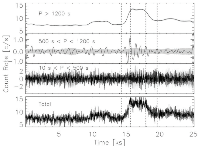
Figure 3 Top: Solar coronal loops undergoing transverse oscillations observed by TRACE (Schrijver et al. 2002). Analysis of loop oscillations by (Wang & Solanki 2004) indicates X-ray intensity variations have a pulse fraction as high as 13%. Bottom: An XMM-Newton lightcurve of a flare on AT Mic decomposed into three frequency bands: low ( P > 1200 \text{ s} ) showing gross flare structure; medium ( 500 \text{ s} < P < 1200 \text{ s} ) illustrating a coherent flare loop oscillation; and the high frequency ( 10 \text{ s} < P < 500 \text{ s} ) noise component. The sum of these add up to the original data (lower panel). Loop oscillations provide direct diagnostics of magnetic field strength and loop length (Mitra-Kraev et al. 2005).
