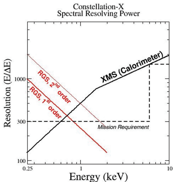
FIGURE 2. Spectral resolving power and requirements for the Constellation-X gratings and calorimeter instruments. Note that calorimeters have a fixed \Delta E (presented as FWHM) so the calorimeter curve reflects the current detector requirements for the calorimeter, not the actual performance of the calorimeter (e.g., the resolution curve might be built up with different types of calorimeter pixels in different locations of the array). These curves will change as the mission design evolves. Note that the gratings have a fixed \Delta\lambda (presented as HEW).
