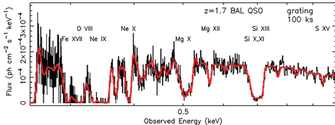
Figure 3: 100 ks Constellation-X simulation of a z = 1.7 quasar with an ionized, high velocity outflow and a flux comparable to PG1115+080 (Chartas et al. 2003). Substantial effective area at low energies (0.2–1 keV) is essential; crucial spectral features such as the resonance lines and edges of highly ionized O, Ne, Mg, and Si ( E = 0.5 – 2.7 keV) move to lower energies with redshift. These spectral features provide important constraints on the physical conditions in moderate column density gas.
