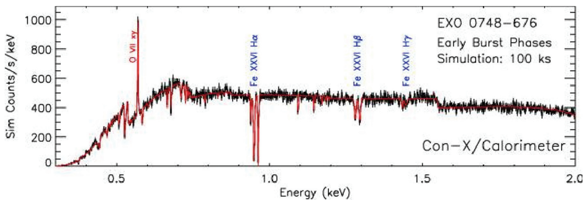
Figure 7: Simulated spectrum of the early phases of the X-ray bursts from the accreting neutron star EXO 0748-676 using the Constellation-X calorimeter. A 100 ks observation should result in 1 ks of burst time. The blue labeled lines are gravitationally red-shifted absorption lines from the neutron star atmosphere. The remaining spectral structure originates in the circumstellar material. The model was developed using the XMM-Newton data and theoretical calculations for the absorption line structure.
