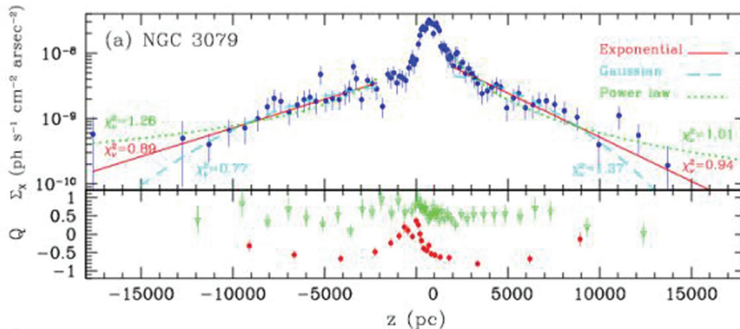
Figure 7: X-ray surface brightness profiles. We observe exponential X-ray surface brightness profiles with scale height \sim 2 - 4 kpc. Spectral hardness Q varies only weakly in halo, at z > 2 kpc. These observations are consistent with the wind hitting and shocking pre-existing exponential halo medium.
