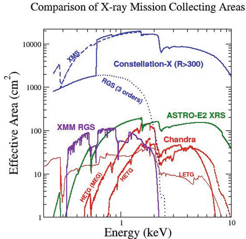
FIGURE 1. Effective area of Constellation-X in the 0.25-10 keV bandpass for both the calorimeter and gratings instruments where the resolution of either (or both) exceeds R=300 . Note that the details of the X-ray Microcalorimeter Spectrometer (XMS) filter transmission below 1 keV will be strongly dependent upon the final mission configuration. The XMM and Chandra effective area curves are for the first order (both dispersion directions co-added).
