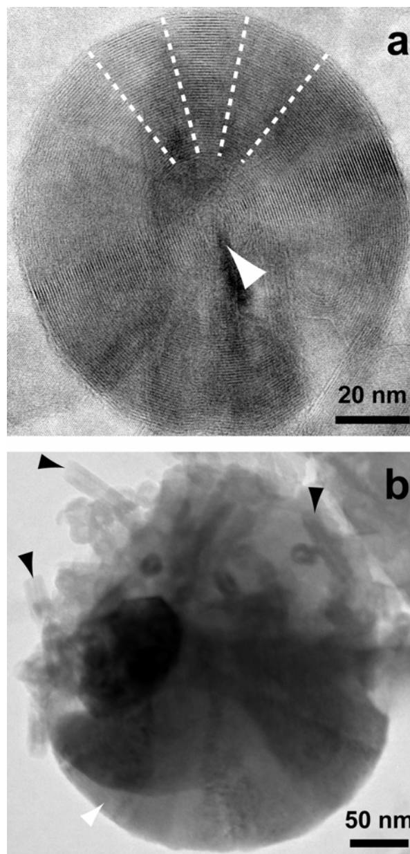
Figure 1 TEM images of the polyhedral material from the Mighei CM chondrite. (a) Sectors (dashed lines) occur around the fiber axis (arrowhead). (b) Partially formed grain. Serpentine nanotubes (black arrowheads) occur with the polyhedral material (white arrowhead).
