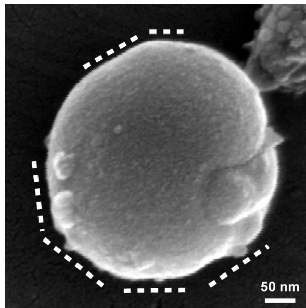
Figure 2 Secondary-electron FEG-SEM image of a polyhedral grain from the Cold Bokkeveld CM chondrite. The sectors (outlined by dashed lines) are visible on the exterior of the grain.
