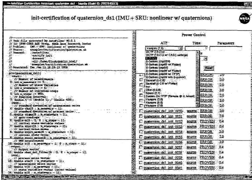
Figure 3: Certification assistant: updated view with prover results
