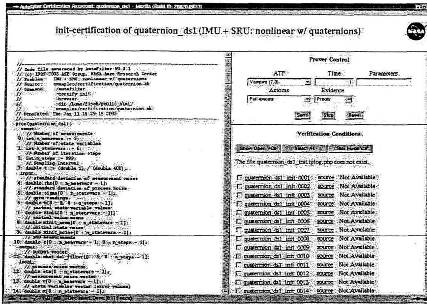
Figure 2: Certification assistant: start-up view
