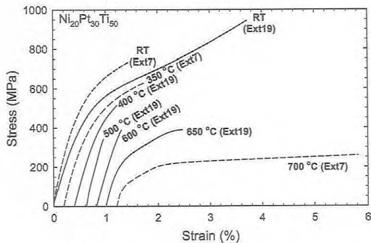
Figure 2. Representative stress-strain curves at various temperatures for the 30Pt materials. Dashed lines are 30Pt (Ext7) and solid lines are for 30Pt (Ext19). Note that tensile curves for temperatures above RT are offset from the origin.
