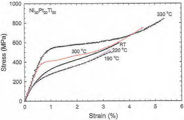
Figure 3. Representative stress-strain curves at various temperatures for the 20Pt alloy.
