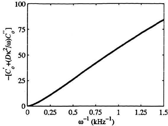
FIG. 3. The dipole coefficient proportionality from Eq. (14) as a function of inverse frequency for a particle with a -120 -mV surface potential and 1 - \mu\text{m} radius in 1 -mM KCl.
