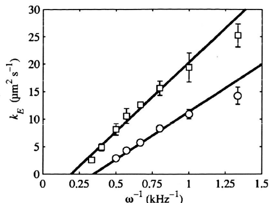
FIG. 9. Aggregation rate constant–frequency relation for two applied potentials. Symbols: circles, \Delta\phi = 4\text{ V} ; squares, \Delta\phi = 6\text{ V} . Each data point is an average from ten experiments; error bars are one standard deviation. Solid lines are linear fits for frequencies of 1\text{ kHz} and larger (inverse frequencies of 1\text{ kHz}^{-1} or smaller).
