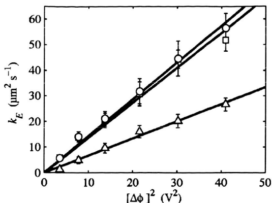
FIG. 8. Aggregation rate constant–applied potential relation. Particles are 2.7\text{-}\mu\text{m} polystyrene in 1.0\text{-mM} KCl. Each point is the mean of ten separate experiments; error bars represent one standard deviation. Two sets of experiments were done at 500\text{ Hz} with particles of same size but different electrophoretic mobilities: circles, M = -8.6\text{ }\mu\text{m cm/V s} ; squares, M = -9.5\text{ }\mu\text{m cm/V s} . Another set of experiments was carried out at 1000\text{ Hz} (triangles). Solid lines were derived by linear regression.
