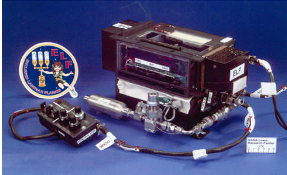
ELF flight hardware assembled for testing.
