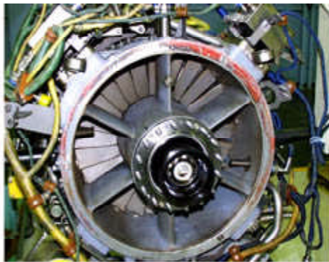
AE 2100 Inlet Housing/Shroud/Guide Vane
