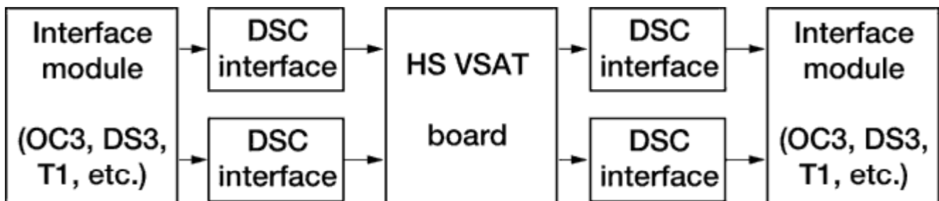
End-to-end user interface for the High Speed VSAT. (Data rates: OC3 = 155 Mbps, DS3 = 43 Mbps, T1 = 1.544 Mbps.)
