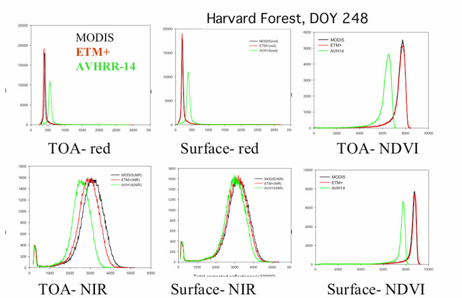
Figure 3. Histograms of red, NIR, and NDVI data over the Harvard forest study site for the 3 sensors, MODIS, Landsat-7 ETM+, and NOAA-AVHRR-14, and for TOA and atmospherically-corrected (surface) conditions.
