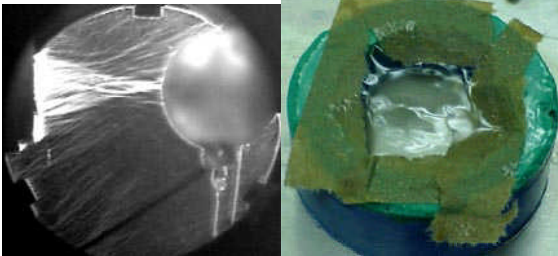
Left: Schlieren image of ultrasonic waves in water deflection in an air-filled glass sphere. Right: Deformation of water surface by acoustic radiation pressure.
