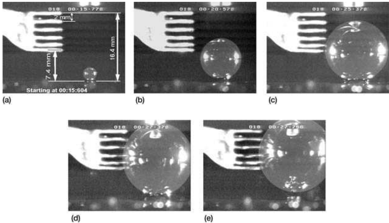
Selected pictures of a single bubble during a growth-departure cycle inception of nucleation.
