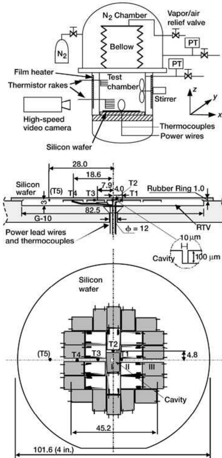
Top: Experimental setup. Center and bottom: Configuration of silicon wafer heater. (Dimensions in millimeters unless marked otherwise.)
